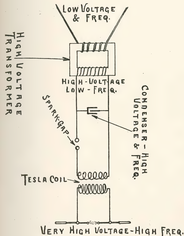
Fig. 14—Diagram of Tesla Type.
