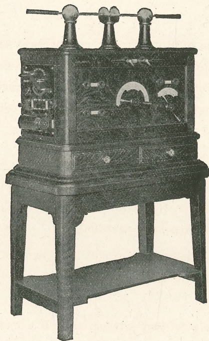
Fig. 1—Large Tesla Coil.
