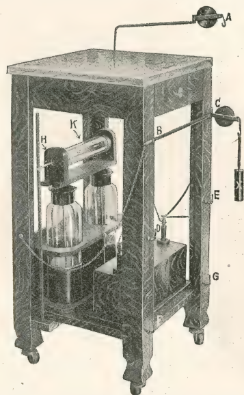
Fig. 25—Resonator for X-Ray Coil.
