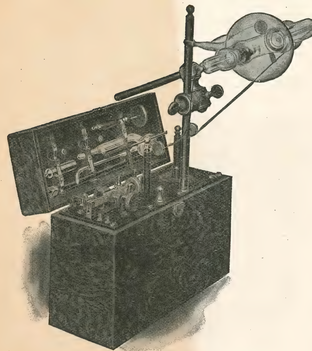
Fig. 40—Portable Coil.
