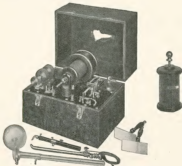
Fig. 54c—Portable Outfit with Two Inductors.
