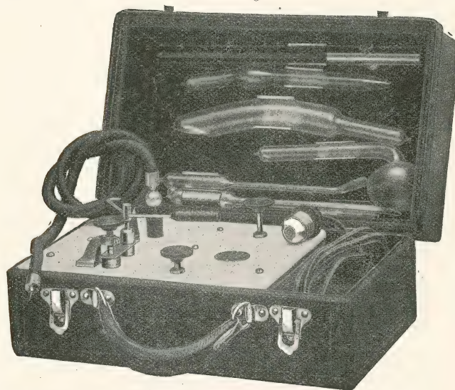
Fig. 54a—Portable Outfit.
