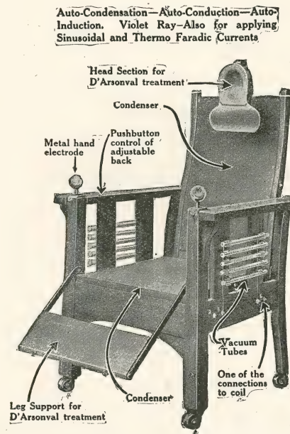
Fig. 37a—A High Frequency Treatment Chair.
