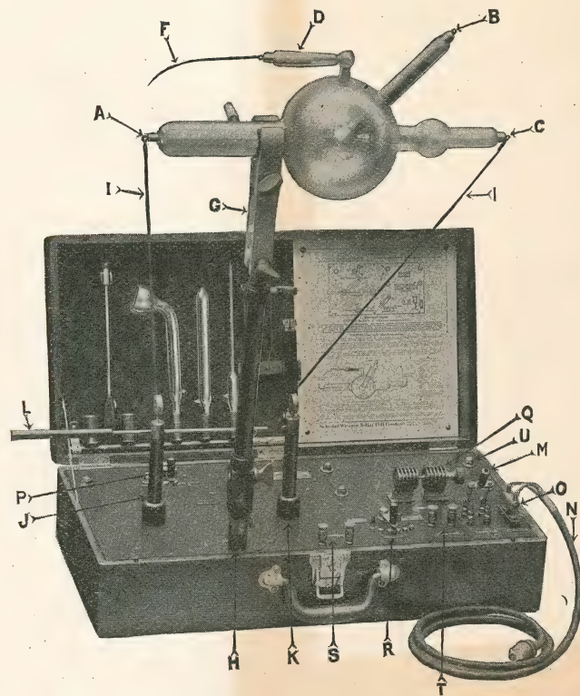
Fig. 39—Portable Coil.
