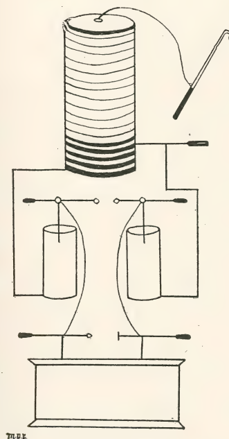
Fig. 15—Diagram of Oudin Resonator.
