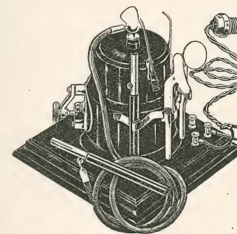
Figs. 11 and 12—Portable Coils.
