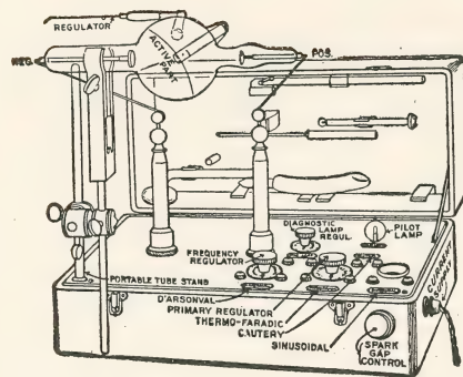
Fig. 5—Portable High Frequency Coils.
