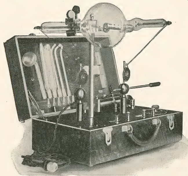
Fig. 64—Portable X-Ray and High Frequency Coil.
