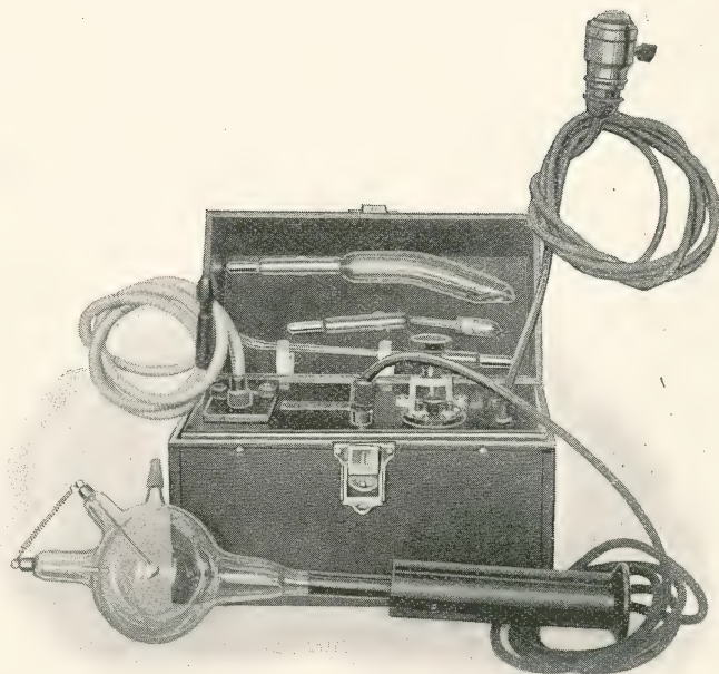
Fig. 44b—Portable Outfit with Novel X-Ray Tube for Surface Treatment.
