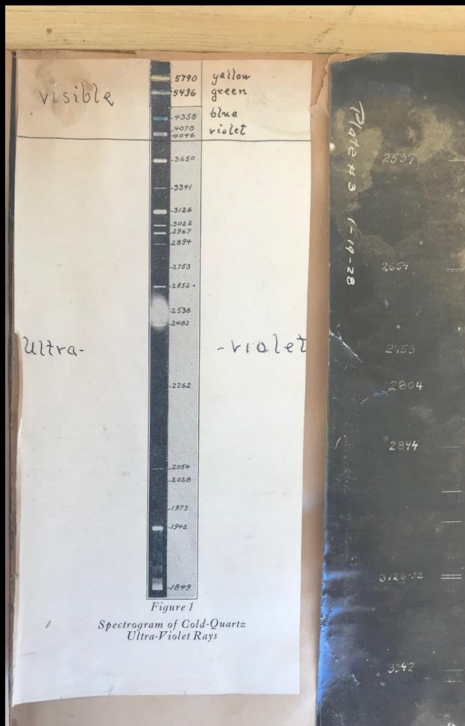
Early spectral analysis of quartz lamps from the scrapbook of Frederick Finch Strong (1920s)
