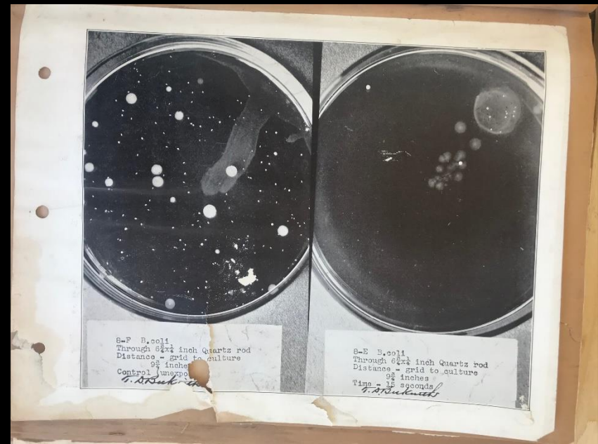
Early records of killing bacteria in petri dishes with ultraviolet radiation. (Frederick Finch Strong scrapbook)
