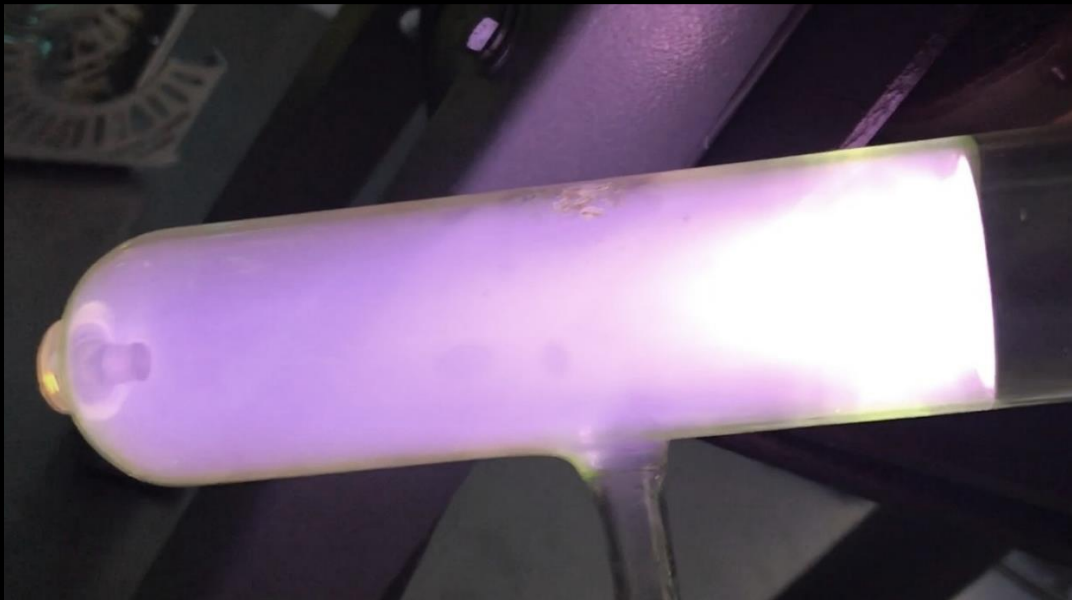
Frederick Finch Strong Ultraviolet Lamp with Iodine Vapor (1900) (Replica built by author)
