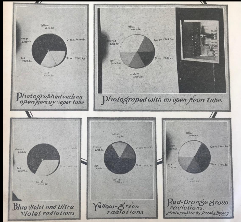
Early spectral analysis of quartz lamps from the scrapbook of Frederick Finch Strong (1920s)
