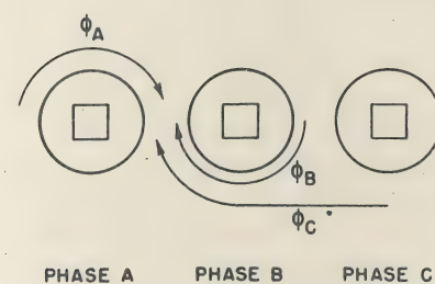
Fig. 3. Flux pattern between sheaths of isolated-phase bus
