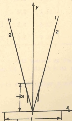
Fig. 5. Resistance measurement for a radial earth electrode. 1. Lines along which equation (4) is satisfied for symmetrically disposed electrodes. For these, x' = y'/15 ; 2. Lines of accurate measurement (columns 3 and 4 of table).
