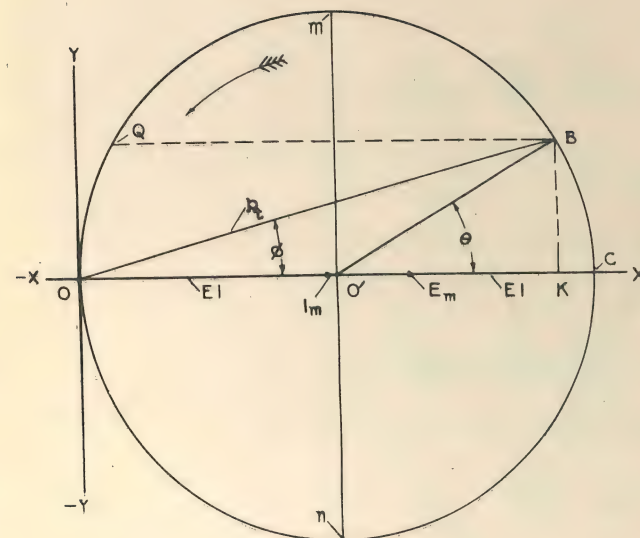
Figure 13. Diagram describing power in a resistive circuit.
