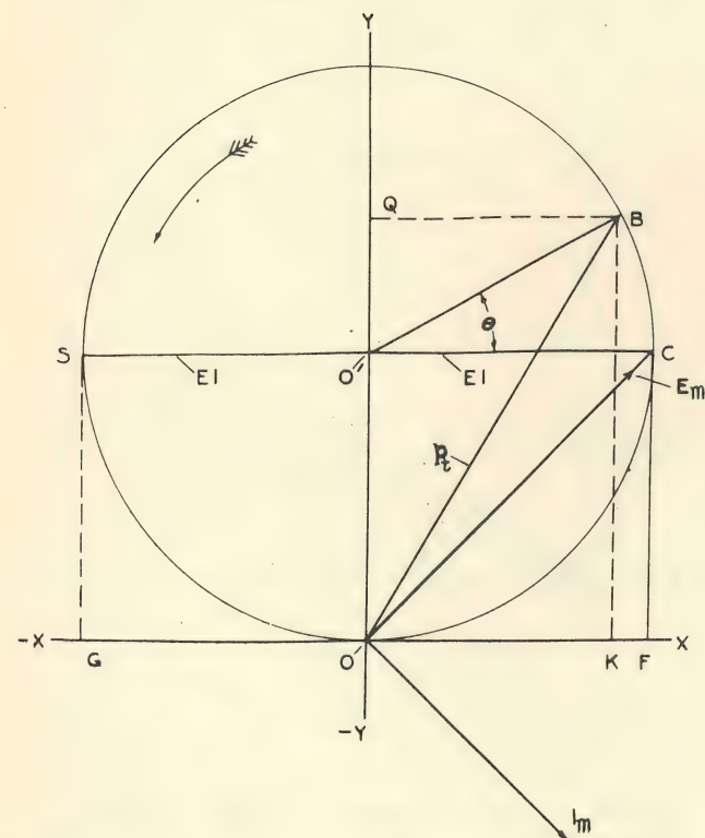
Figure 7. Vector diagram of real and imaginary power and total power in an inductive circuit with resistance negligible.
