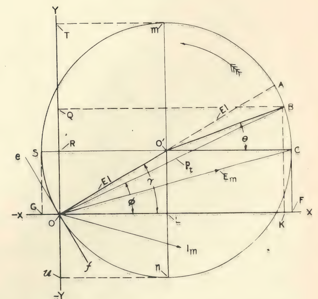
Figure 5. Vector diagram describing real and imaginary power, total power, E.M.F. and current in an inductive circuit.
