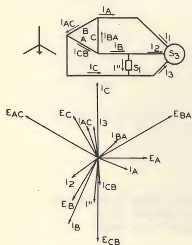
Fig. 3. Circuit Diagram and Phase Relations of a Grounded Wye-Delta Transformer Bank
