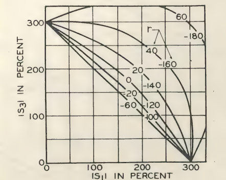
Fig. 12. Load Limit Curves for Transformer C of Ungrounded Wye-Delta Banks in Percent of Allowable Transformer Load
