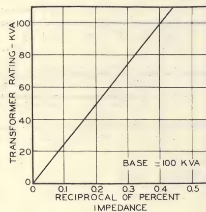
Fig. 21. Relationship between Transformer Rating and Impedance for Three to One Hundred KVA Transformers
