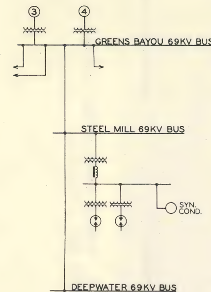
Fig. 1. Method of serving arc furnaces
