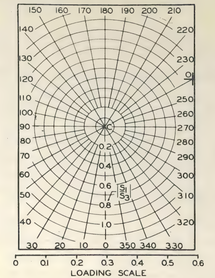
Fig. 8. Transformer B Circle Diagram for Ungrounded Wye-Delta Banks
