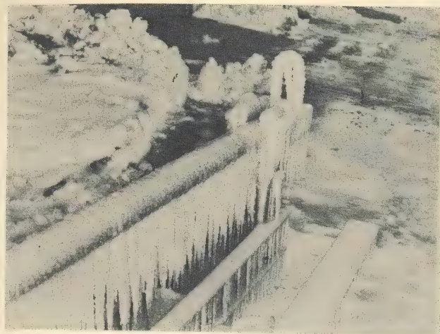
Fig. 14. Ice Test 1600 Amp. 161 KV Switch. From Closed to Open - Switch Shown Frozen in Closed Position.
