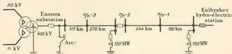
FIG.6. The diagram of the 400 kV Kuibyshev-Moscow line during the experiments with extinction of the sustained faulty current arc.
