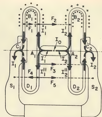
Fig. 6. Distribution of Currents and Magnetic Fields in Loop Contact Assembly.
