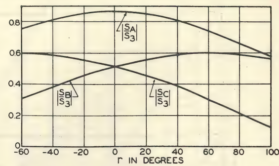
Fig. 20. Comparison of Transformer A , B , and C Loading Curves for Delta-Delta or Grounded Wye-Delta Banks
