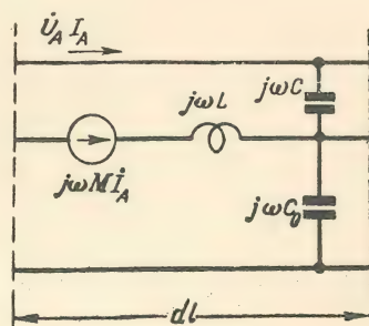
FIG.2. The diagram of the element of the line with distributed parameters for the calculated example.
