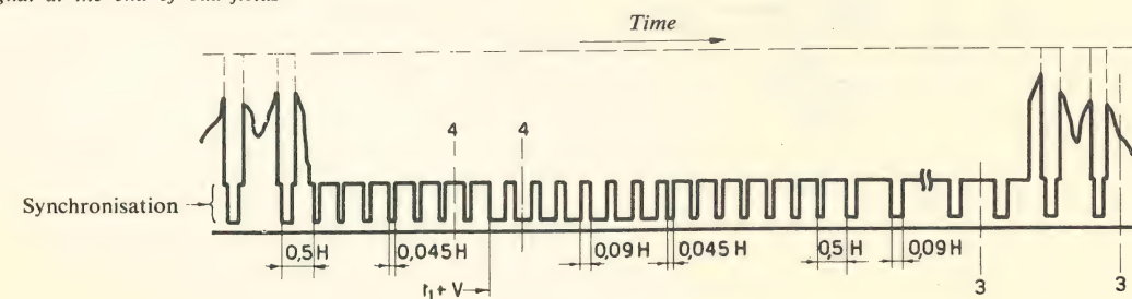
Fig. 7 - Synchronizing Waveform, System VIII
