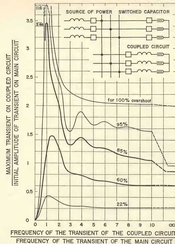
Fig. 15. Relationship between coupled circuit and main circuit overvoltages for circuits of the types shown (left)
