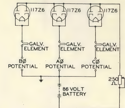
Fig. 2. Oscillograph voltage biasing circuit.
