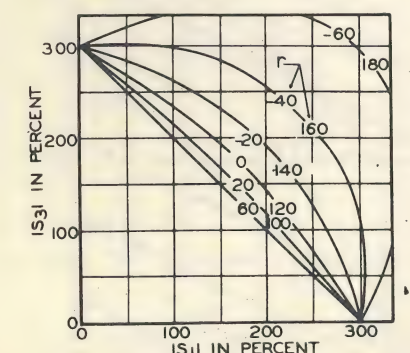
Fig. 11. Load Limit Curves for Transformer B of Ungrounded Wye-Delta Banks in Percent of Allowable Transformer Load
