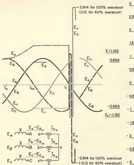
Fig. 11. Circuit and voltages considered in the 3-phase capacitive restrike case when the restrike occurs in phases A and C 7/12-cycle after interruption in phase A (left)
