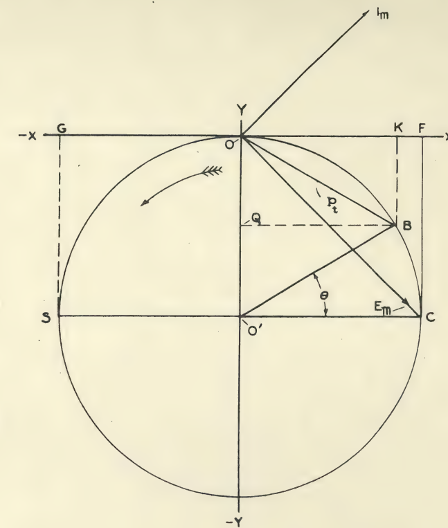
Figure 11. Diagram describing power in a capacitive circuit with resistance negligible.
