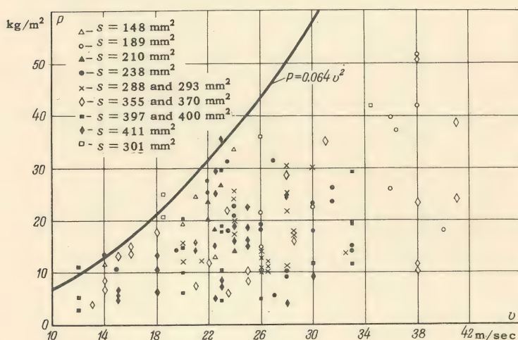
FIG. 6. Relation between wind pressure on conductor projection area normal to wind direction and wind speed according to measurements in France.
