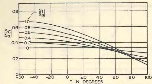
Fig. 19. Transformer C Loading with all Units Identical for Delta-Delta or Grounded Wye-Delta Banks
