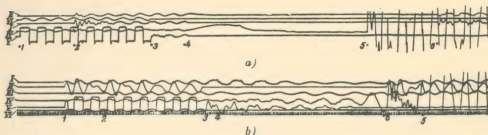
FIG.9. Oscillograms of the experiments with the three-phase switching off and reclosing. (a) section of the line with a voltage transformer; (b) section of the line with a voltage transformer and reactor. I—voltage of the "yellow" phase U_y ; II—current of the "yellow" phase I_y ; III—voltage of the "green" phase U_g ; IV—voltage of the arc (of the "red" phase) U_r ; V—current I_{su} ; VI—short-circuit current I_{sh} . (1) the beginning of the short-circuit; (2) reclosing of the sound phase with a delay; (3) switching off the "red" phase (the end of the short-circuit); (4) switching off the "yellow" and "green" phases; (5) reclosing of the "red" phase; (6) reclosing of the "yellow" and "green" phases.
