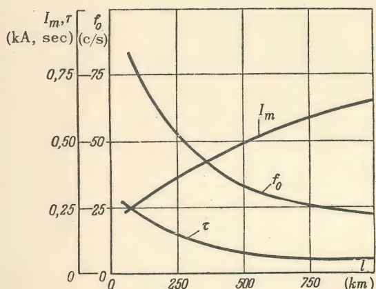
FIG.1. The values of the amplitudes of the discharge current I_m , time constant of the discharge \tau and the proper frequency f_0 at the discharge of the line through the shunting reactor as a function of the length of the disconnected section.
