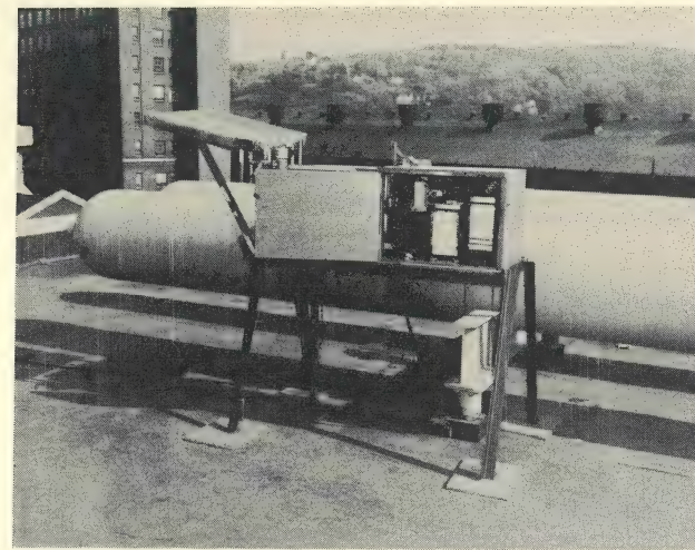
Fig. 1. Rainfall gauge located on roof of the new High Power Laboratory at East Pittsburgh, Pa.
