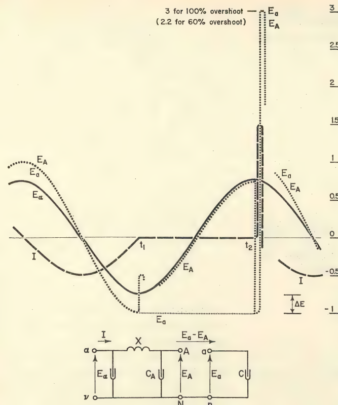
Fig. 7. Circuit, voltages, and current considered in the single-phase capacitive restrike case
