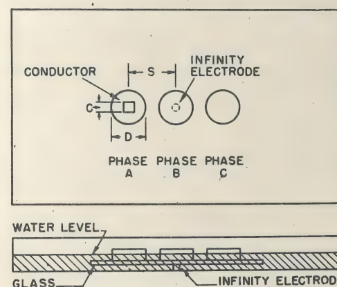
Fig. 2. Field analyzer set-up of isolated-phase bus
