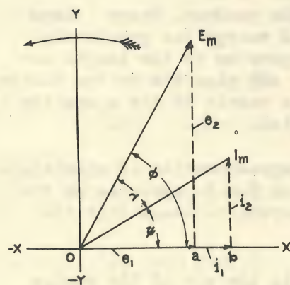
Figure 1. Vector diagram of the E.M.F. and current in an inductive circuit.
