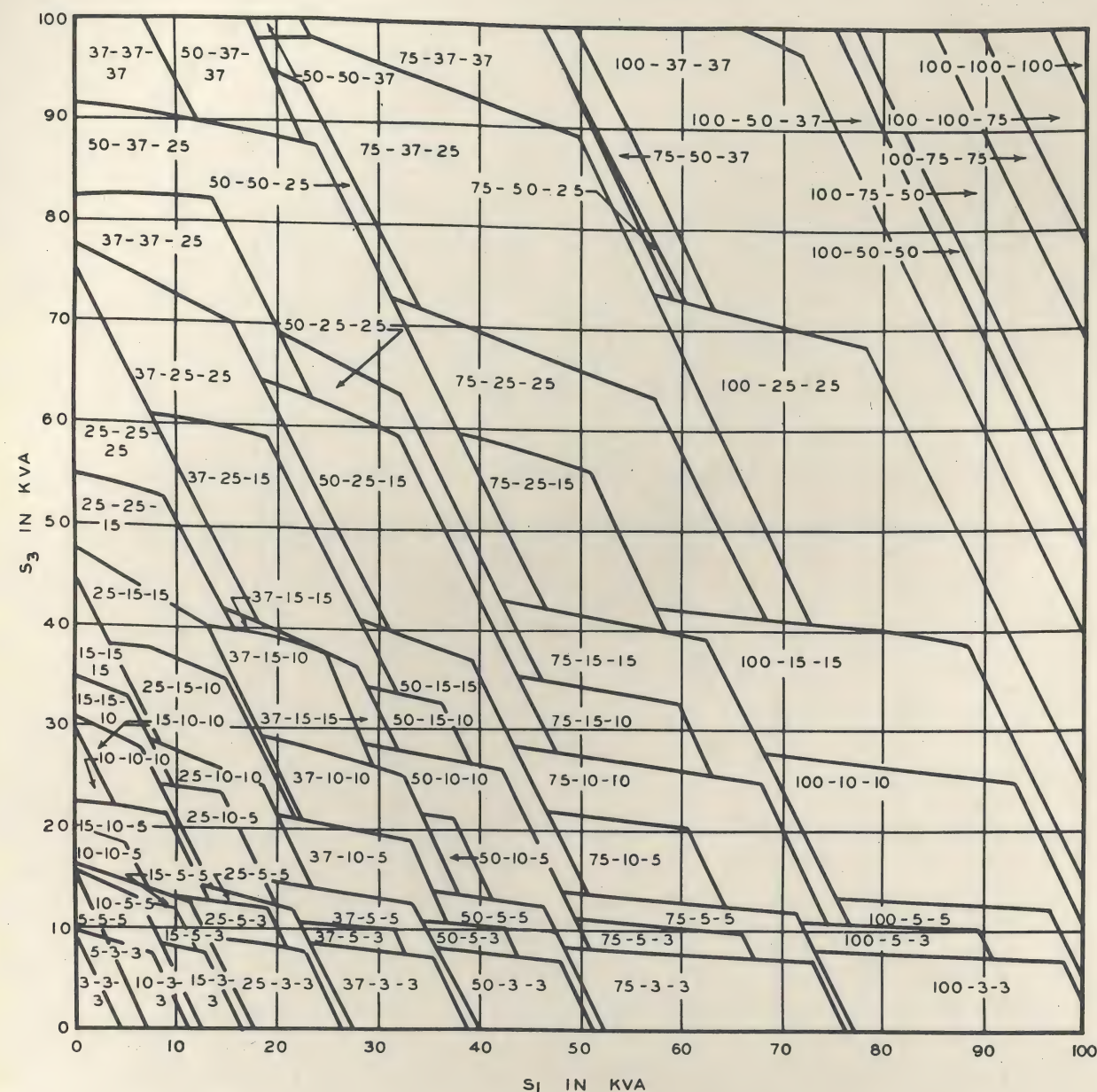
Fig. 25. Preferred Loading Curves with r = 20^\circ for Delta-Delta or Grounded Wye-Delta Banks
