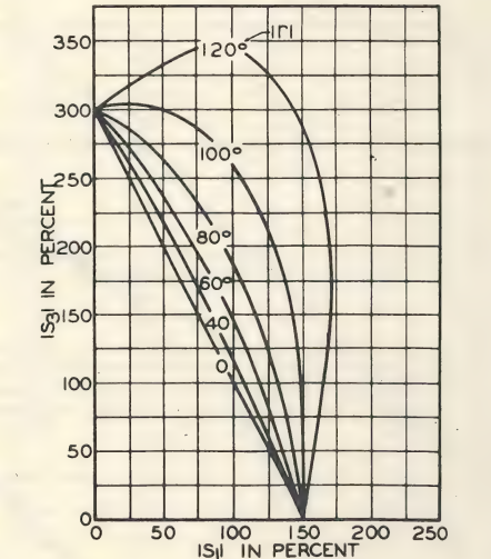
Fig. 10. Load Limit Curves for Transformer A of Ungrounded Wye-Delta Banks in Percent of Allowable Transformer Load
