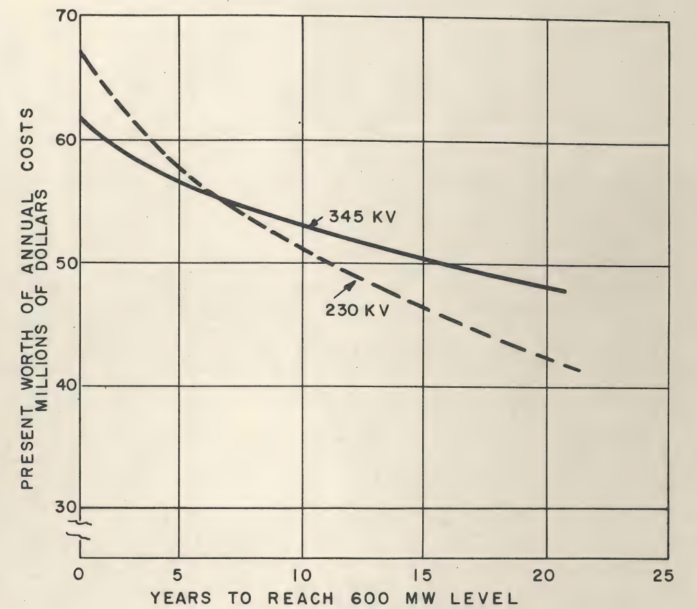
Fig. 4. Revenue requirements for 100 mile transmission as a function of the time to full utilization of the station capacity
