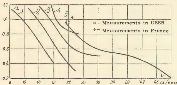
FIG. 4. Relation between greatest values of coefficient a and wind speed as measured in different countries:
