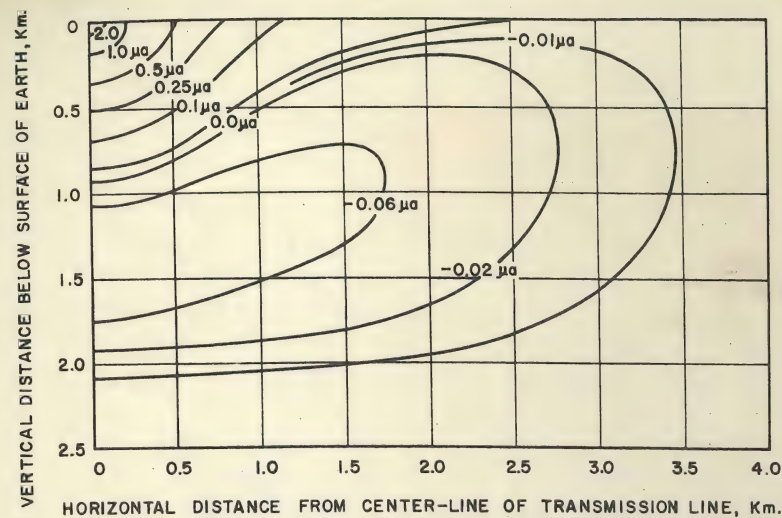
Figure 3. Constant current density plot of the imaginary component of zero-sequence current density in microamps per square meter per amp of zero-sequence current per phase. Conductor height 20 meters, spacing 10 meters and earth conductivity 10 micromhos/meter.
