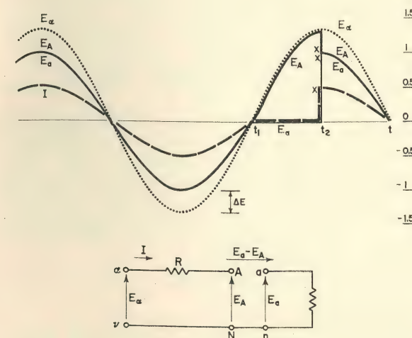
Fig. 1. Circuit, voltages, and current considered in the single-phase resistive restrike and energizing cases (left)
