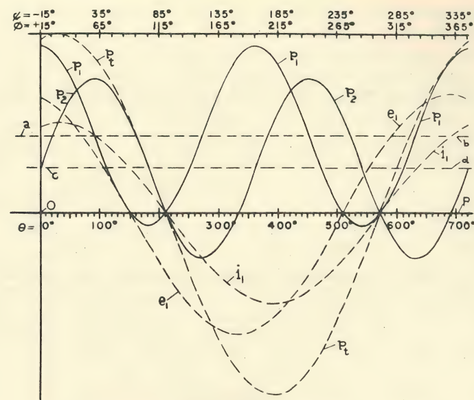
Figure 6. Curves describing real and imaginary power, total power, E.M.F. and current in an inductive circuit.
