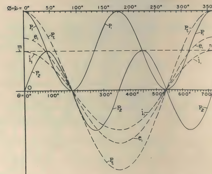
Figure 14. Power curves together with E.M.F. and current in a resistive circuit.
