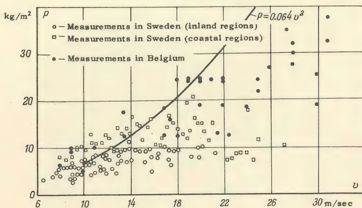
FIG. 5. Relation between wind pressure on conductor projection area normal to wind direction and wind speed according to measurements in Sweden and Belgium.
