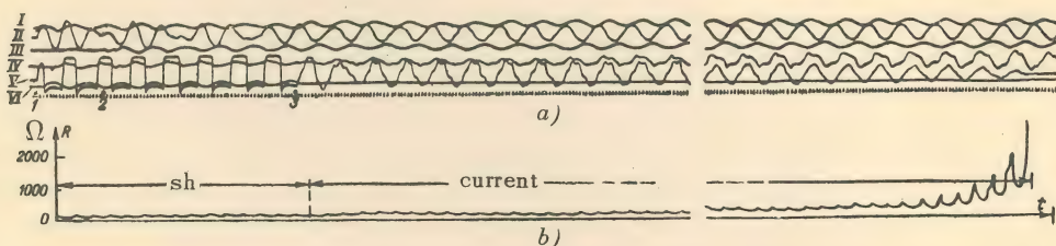
FIG.8. Oscillogram of the experiment (a) and the graph of the resistance of the path of the arc (b) on the single-phase short-circuit and switching off one phase. I — voltage of the "yellow" phase U_y . II — current of the "yellow" phase I_y . III — voltage of the "green" phase U_g . IV — voltage on the arc (of the "red" phase) U_r . V — current I_{su} . VI — short-circuit current I_{sh} (1) the beginning of the short-circuit; (2) connecting of the sound phase with a delay; (3) switching off the "red" phase (the end of the short-circuit).
