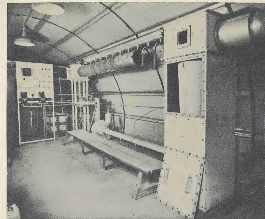
Fig. 3. Electrostatic precipitator pilot plant.
