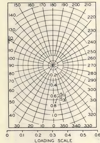
Fig. 9. Transformer C Circle Diagram for Ungrounded Wye-Delta Banks
