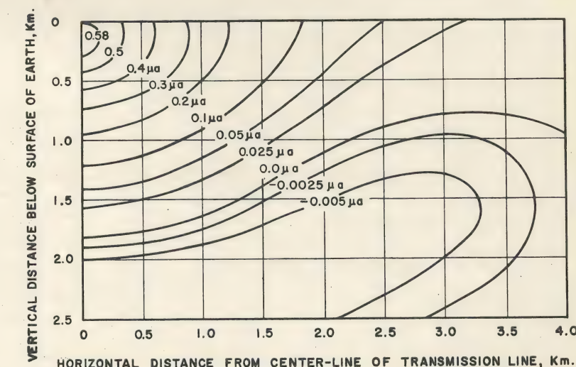
Figure 2. Constant current density plot of the real component of zero-sequence current density in microamps per square meter per amp of zero-sequence current per phase. Conductor height 20 meters, spacing 10 meters and earth conductivity 10 micromhos/meter.
