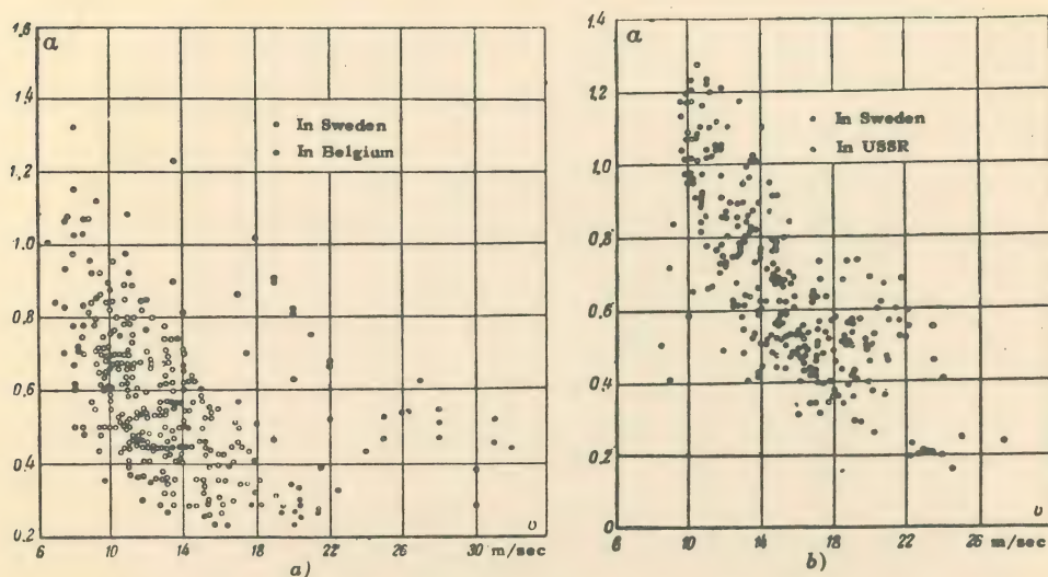
FIG. 1. Relationship between the coefficient \alpha and wind velocity
