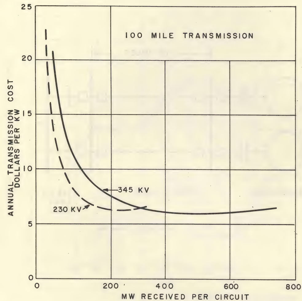
Fig. 3. Annual revenue requirements for 100 mile transmission system at a 15 per-cent annual carrying charge rate
