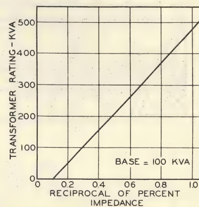
Fig. 22. Relationship between Transformer Rating and Impedance for Fifty to Five Hundred KVA Transformers
