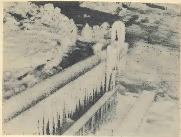
Fig. 14. Ice Test 1600 Amp. 161 KV Switch. From Closed to Open - Switch Shown Frozen in Closed Position.
