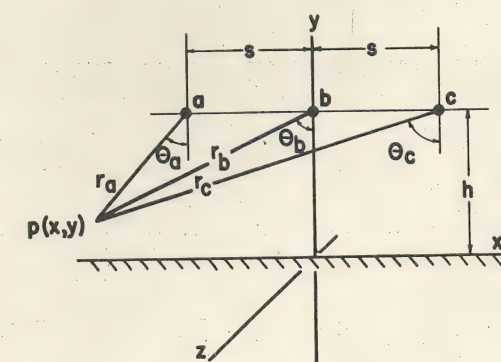
Figure 1. Transmission line conductor spacing and location of images.
