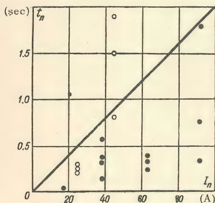
FIG. 10. Experimentally found durations of the arc extinction in relation to the current:
