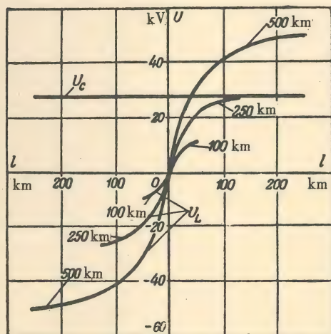
FIG.3. Capacitive U_c and inductive U_l component of the voltage on the disconnected phase (in the absence of the reactor).
