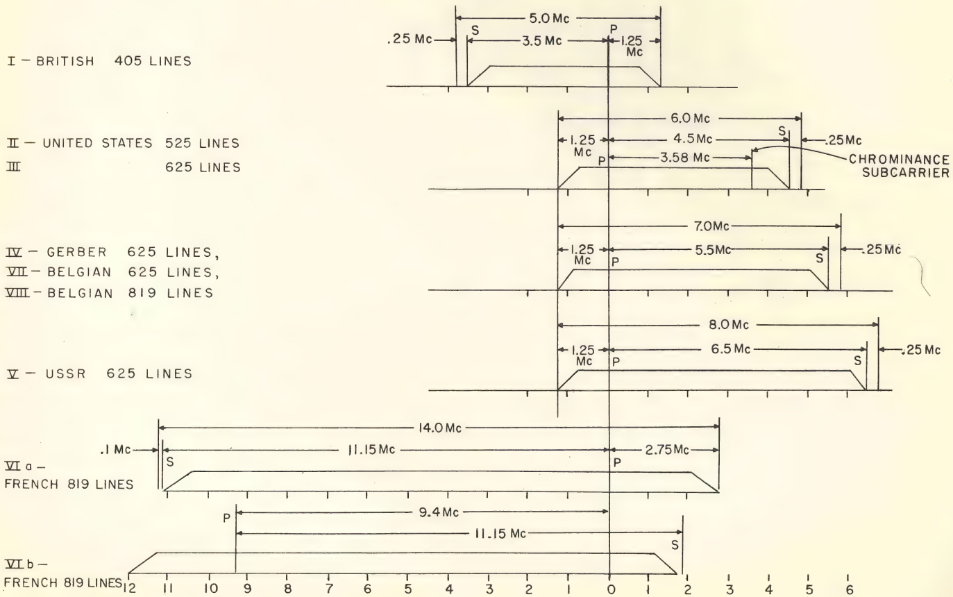
Fig. 1 - Channel Arrangement for Various Systems
