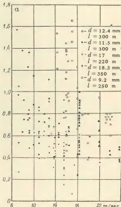
FIG. 3. Relation between coefficient a and wind speed according to results obtained in the U.S.S.R.
