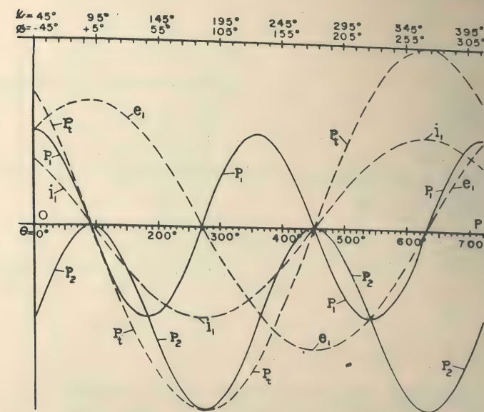
Figure 12. Power curves together with E.M.F. and current in a capacitive circuit with resistance negligible.
