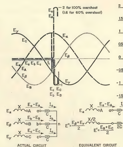
Fig. 13. Circuit, voltages, and current considered in the single-phase capacitive energizing case (left)
