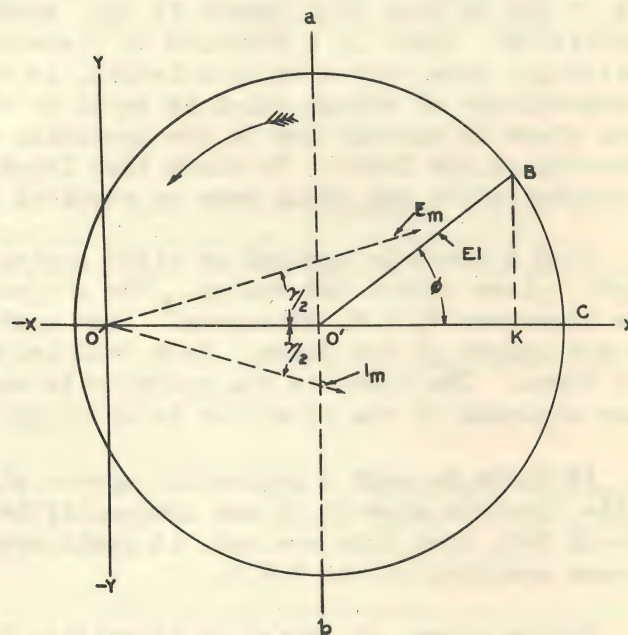
Figure 2. Vector diagram of real power in an inductive circuit.
