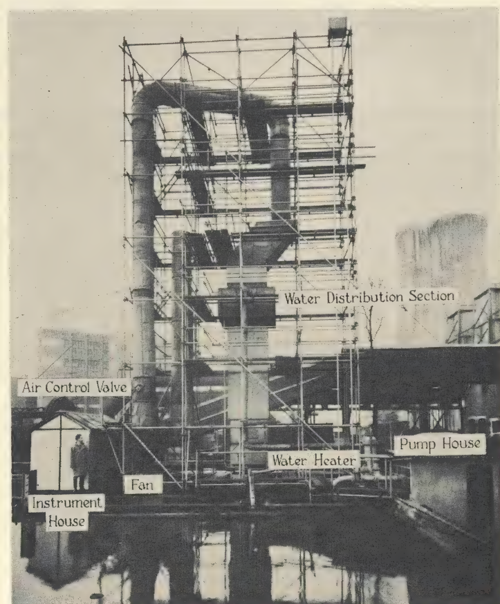
Fig. 2. Experimental water-cooling tower.
