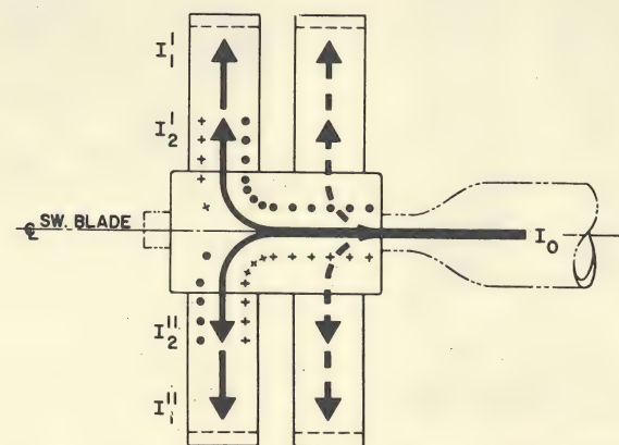
Fig. 9. Current and Field Distribution in "Offset" Jaw with Loop Contacts.
