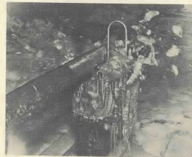
Fig. 12. Ice Test 1600 Amp. 161 KV Switch. Second Stage - Blade Coming Down in Jaw.
