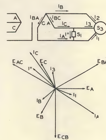
Fig. 6. Circuit Diagram and Phase Relations of an Open-Delta Transformer Bank with an Open Connection
