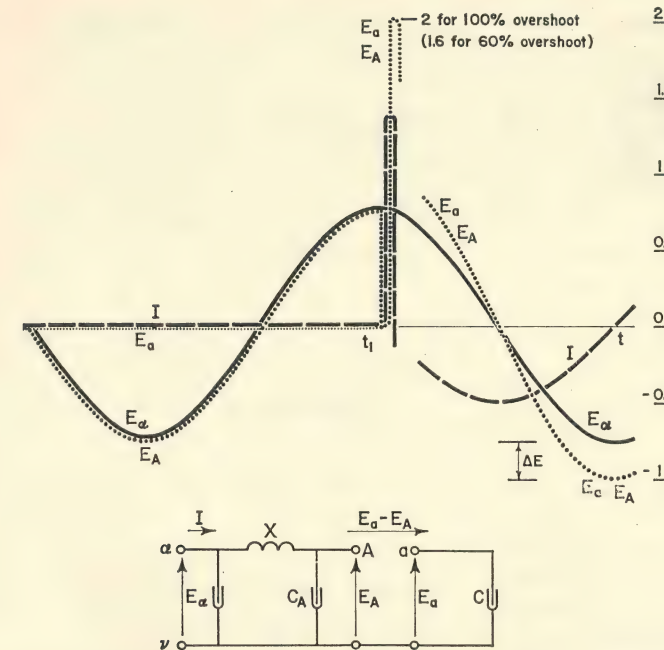
Fig. 13. Circuit, voltages, and current considered in the single-phase capacitive energizing case (left)
