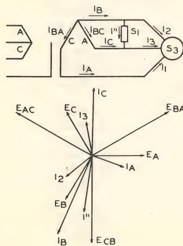
Fig. 5. Circuit Diagram and Phase Relations of an Open-Delta Transformer Bank with a Leading Connection
