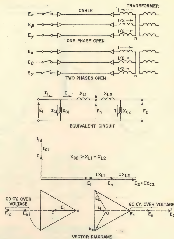
Fig. 15. Relationship between coupled circuit and main circuit overvoltages for circuits of the types shown (left)
