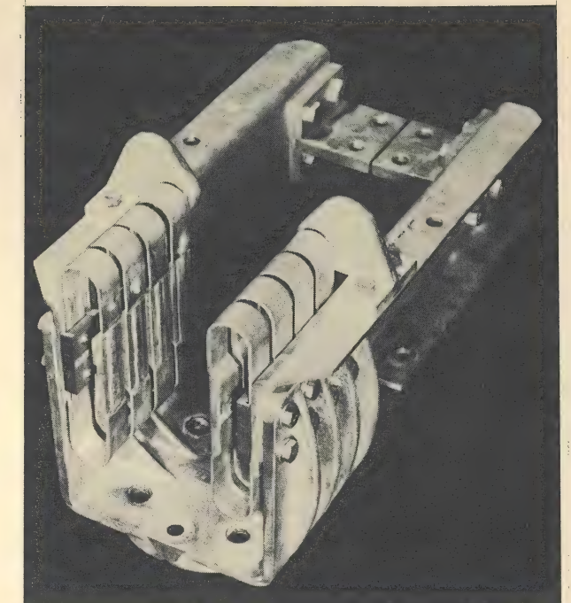
Fig. 3. Jaw Assembly after Momentary Tests Table IV.
