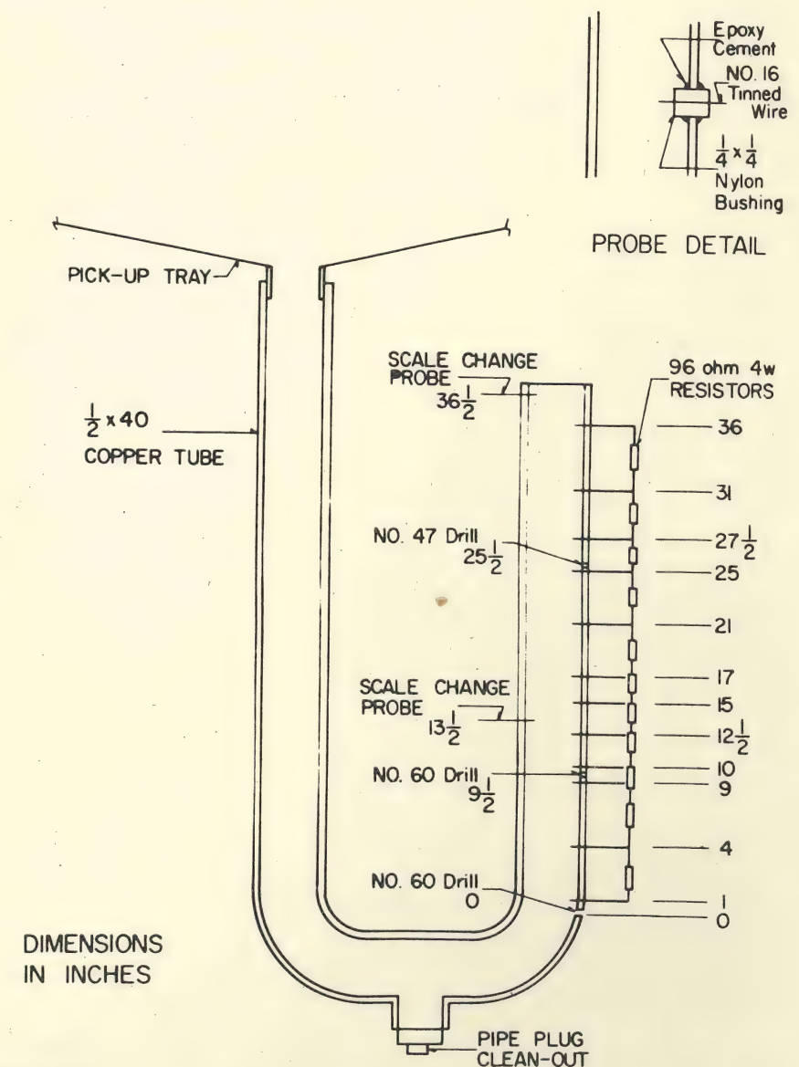
Fig. 2. U-tube rainfall rate gauge
