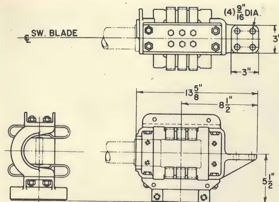
Fig. 5. Jaw Assembly 1200 Amp. 161 KV Horizontal Double Break Switch.
