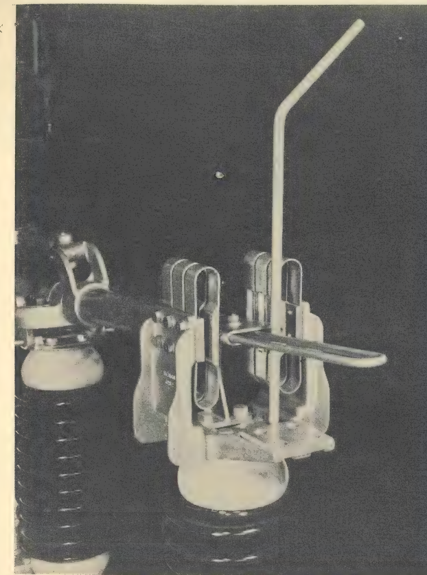
Fig. 1. 34.5 KV 1200 Amp. Switch with Loop Contacts.
