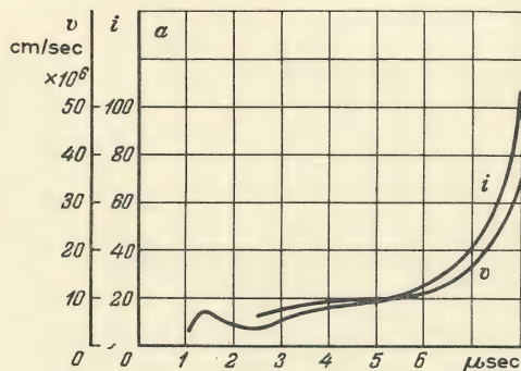
Fig.1 Leader current and leader tip velocity. Spark gap "rod-plane", 100 cm long. Discharge circuit resistance 2.5 k \Omega .
