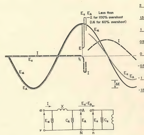
Fig. 5. Circuit, voltages, and current considered in the single-phase inductive energizing case (left)
