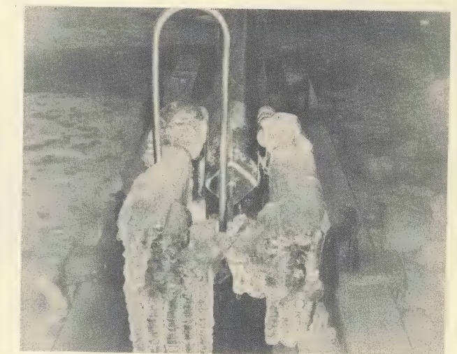
Fig. 13. Ice Test 1600 Amp. 161 KV Switch. Final Stage - Jaw Assembly After Blade Reached Fully Closed Position.
