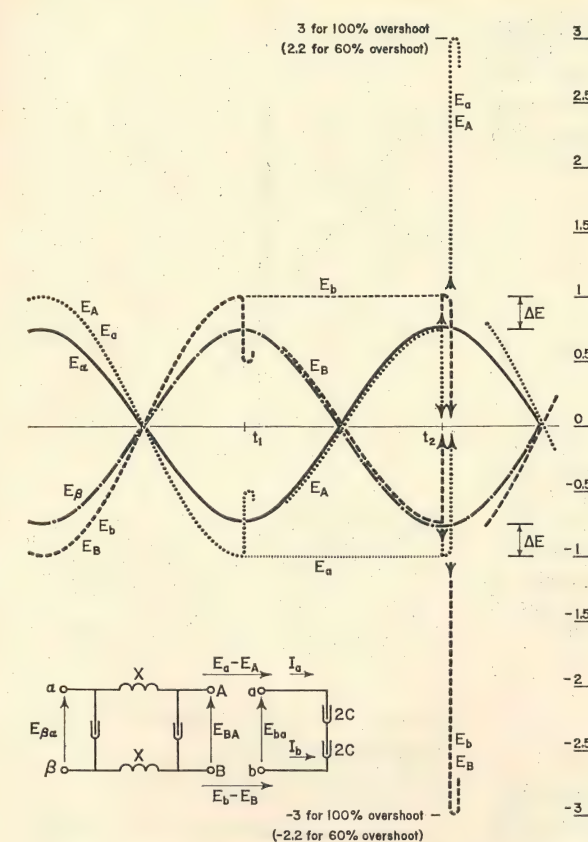
Fig. 9. Circuit, voltages, and current considered in the single-phase capacitive restrike case when both sides of the line contain impedance (left)
