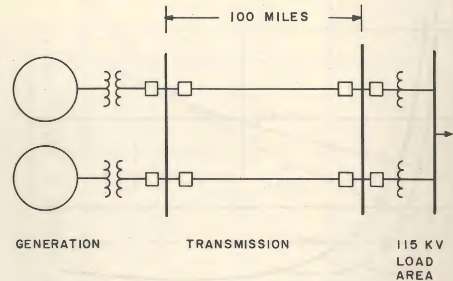
Fig. 2. 100 mile transmission system for economic example
