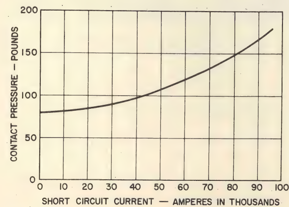
Fig. 7. Relationship between Short-Circuit Current and Contact Pressure in 1200 Amp. Loop Contact Assembly.
