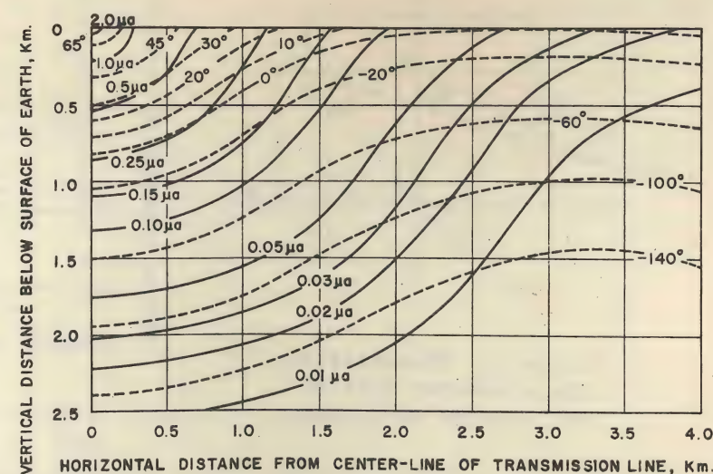
Figure 4. Constant current density plot of the magnitude and phase angle of the zero-sequence current density in microamps per square meter per amp of zero-sequence current per phase. Conductor height 20 meters, spacing 10 meters and earth conductivity 10 micromhos/meter.
