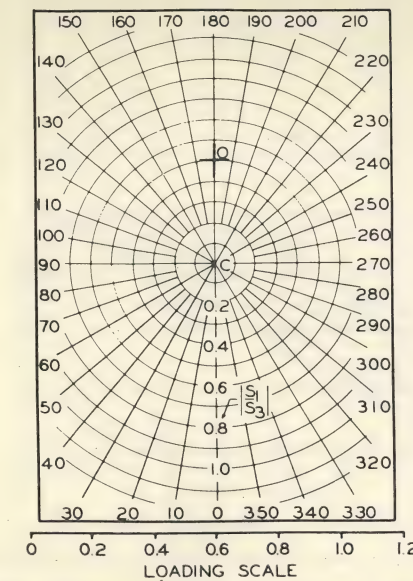
Fig. 7. Transformer A Circle Diagram for Ungrounded Wye-Delta Banks
