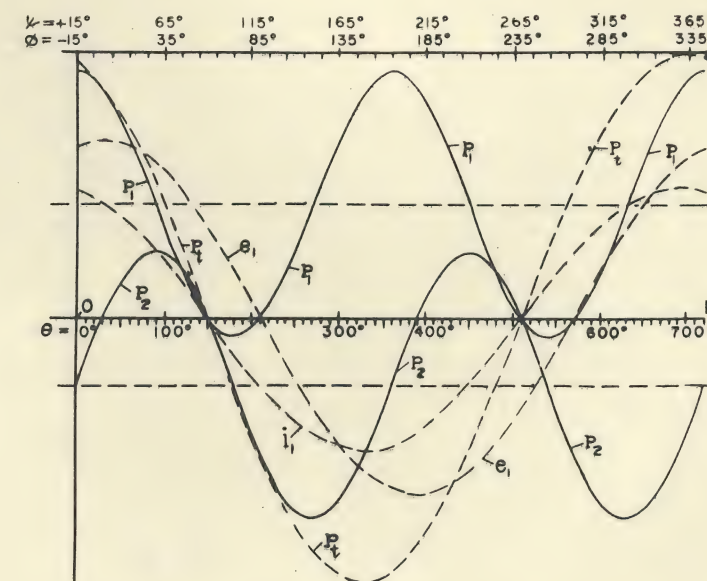
Figure 10. Power curves in a capacitive circuit together with the E.M.F. and current.
