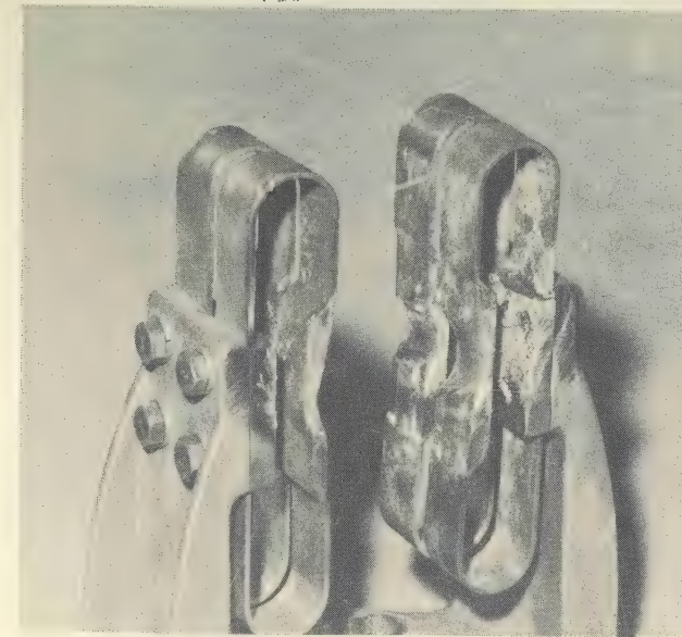
Fig. 10. Loop Contact Assembly Tested to Destruction; Table II Test No. 12; with Current for above NEMA Momentary Rating.
