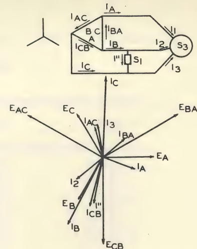
Fig. 2. Circuit Diagram and Phase Relations of an Ungrounded Wye-Delta Transformer Bank
