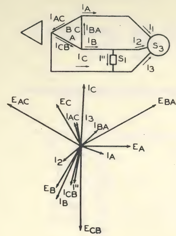
Fig. 1. Circuit Diagram and Phase Relations of a Delta-Delta Transformer Bank
