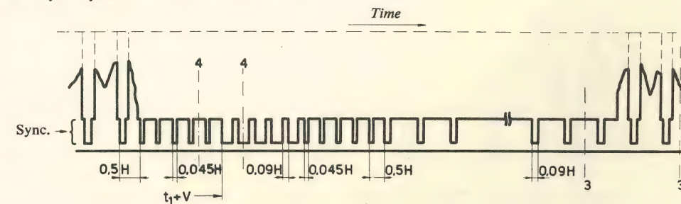
Fig. 6 - Synchronizing Waveform, System VII
