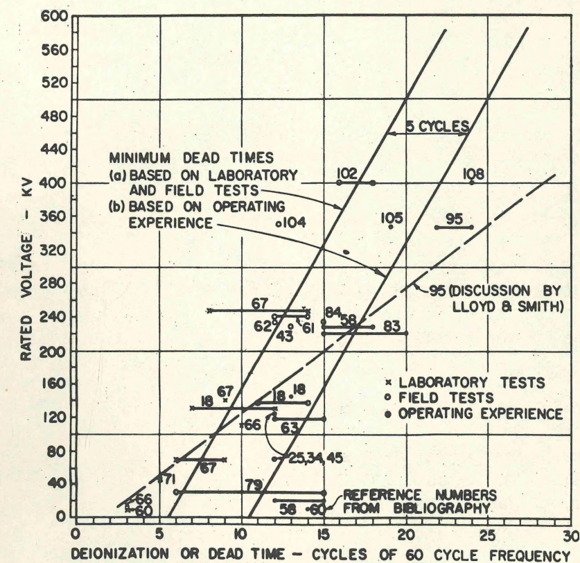
Fig. 1. High Speed Three-Pole Reclosing Deionization Time
