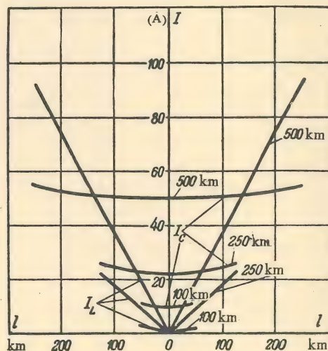
FIG.4. Capacitive I_c and inductive I_l components of the sustained fault current when one phase is disconnected (in the absence of the reactor).
