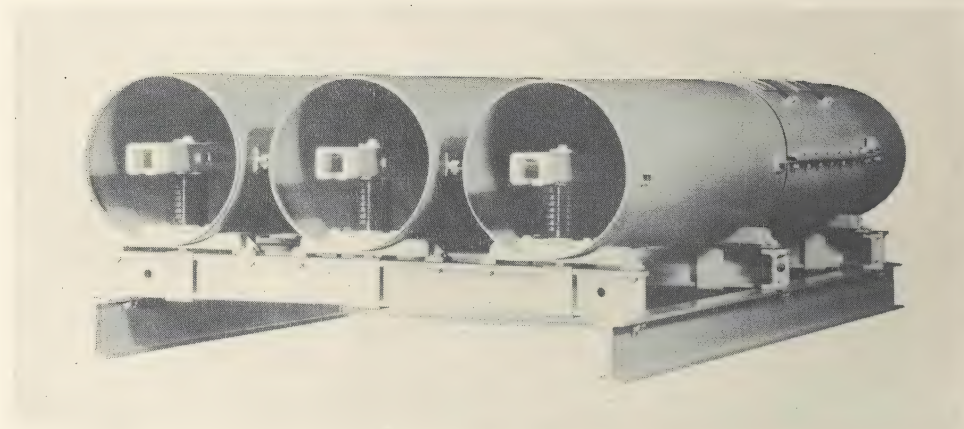
Fig. 1. Typical isolated-phase bus
