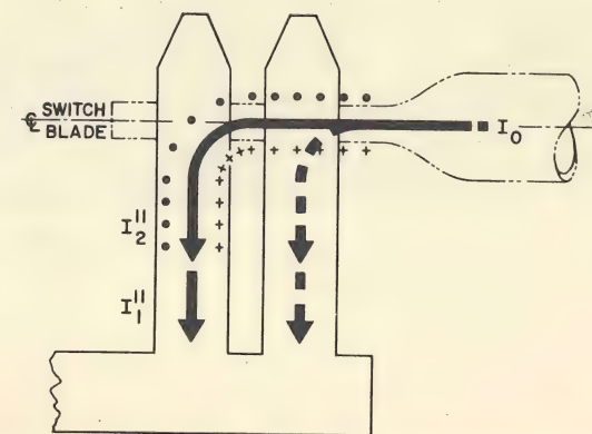
Fig. 8. Current and Field Distribution in "Offset" Jaw with Conventional Contacts.
