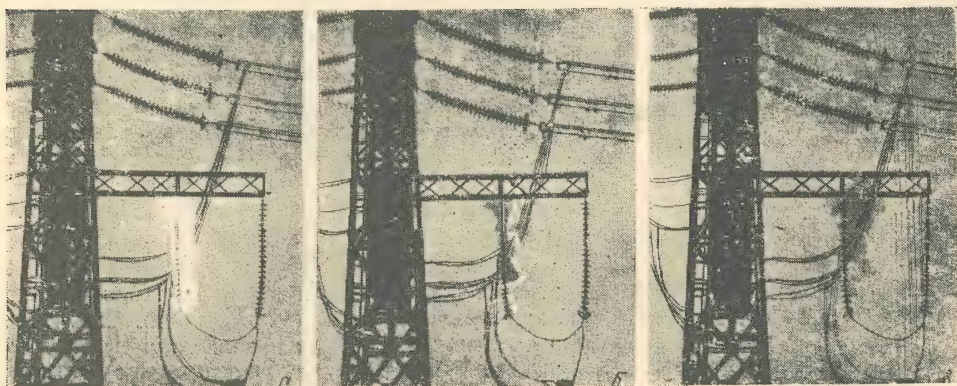
FIG.7. Separate cine-frames of the single-phase short-circuit with the following sustained current arc: (a) short-circuit arc; (b) the sustained current arc before the beginning of extinction; (c) cooling of gases after extinction of the sustained current arc.
