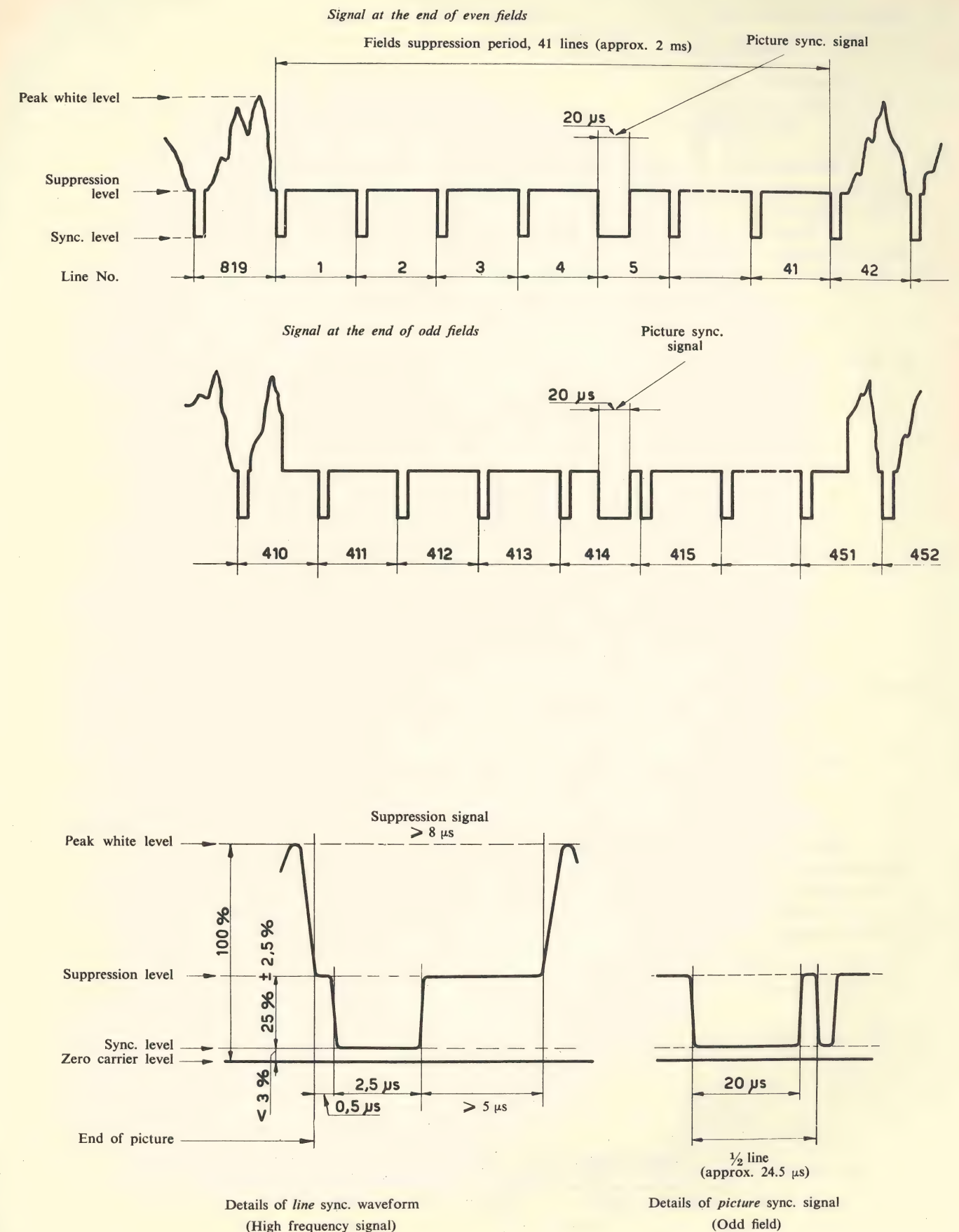
Fig. 5 - Synchronizing Waveform, System VI
