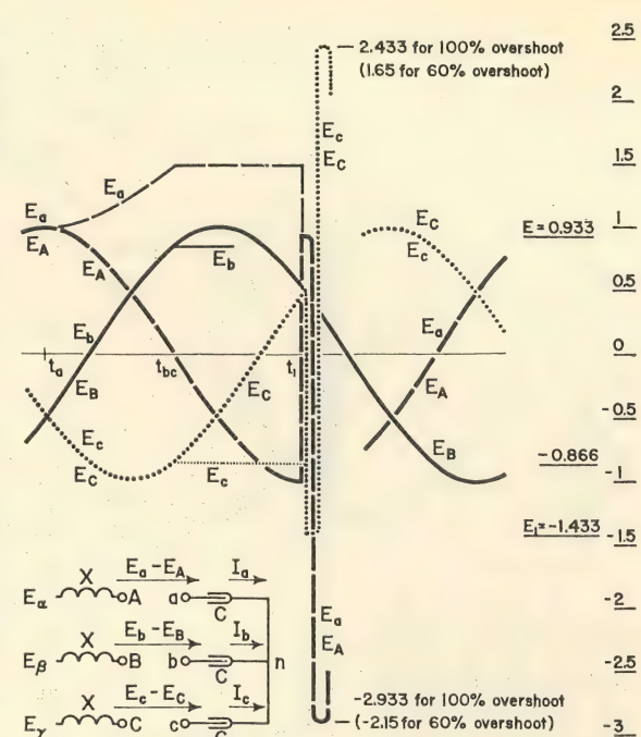
Fig. 9. Circuit, voltages, and current considered in the single-phase capacitive restrike case when both sides of the line contain impedance (left)
