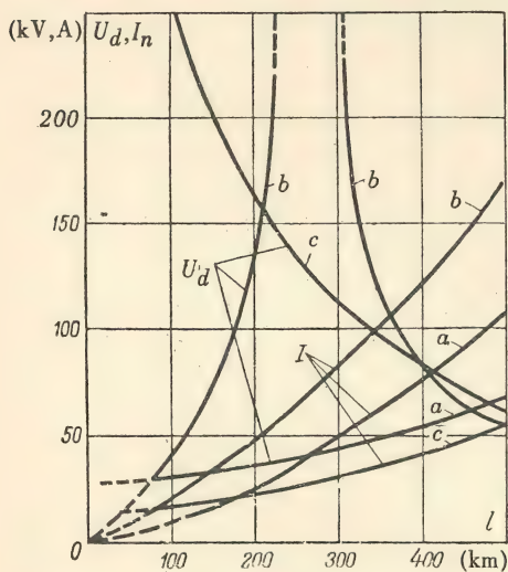
FIG.5. The sustained current and the recovery voltage on the disconnected phase for a point of the end at the section: (a) one phase disconnected, reactor absent; (b) one phase disconnected, reactor present; (c) three phases disconnected, reactor present.
