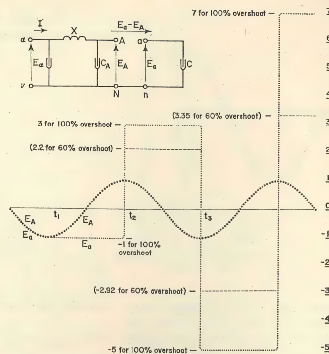
Fig. 8. Voltage build-up attending repetitive restrikes in single-phase capacitive case
