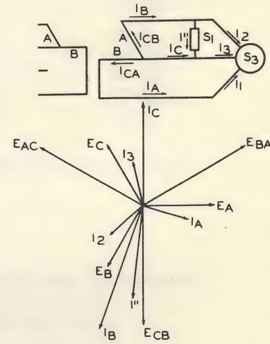
Fig. 4. Circuit Diagram and Phase Relations of an Open-Delta Transformer Bank with a Lagging Connection
