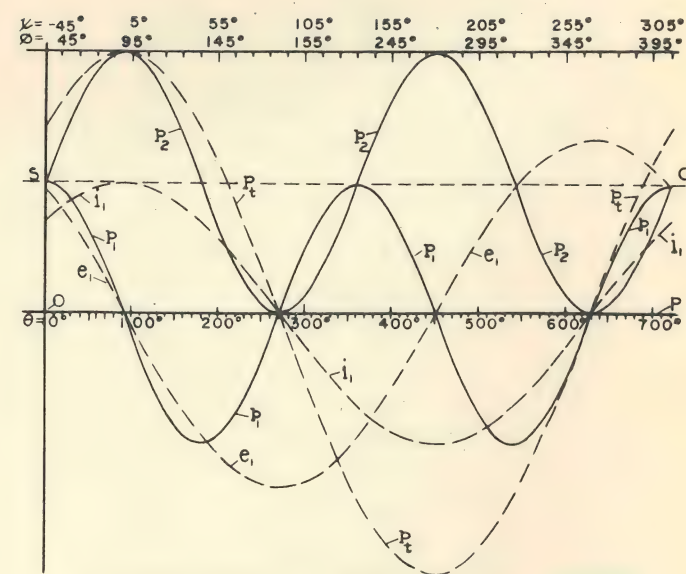
Figure 8. Curves of real and imaginary power, total power, E.M.F. and current in an inductive circuit with resistance negligible.
