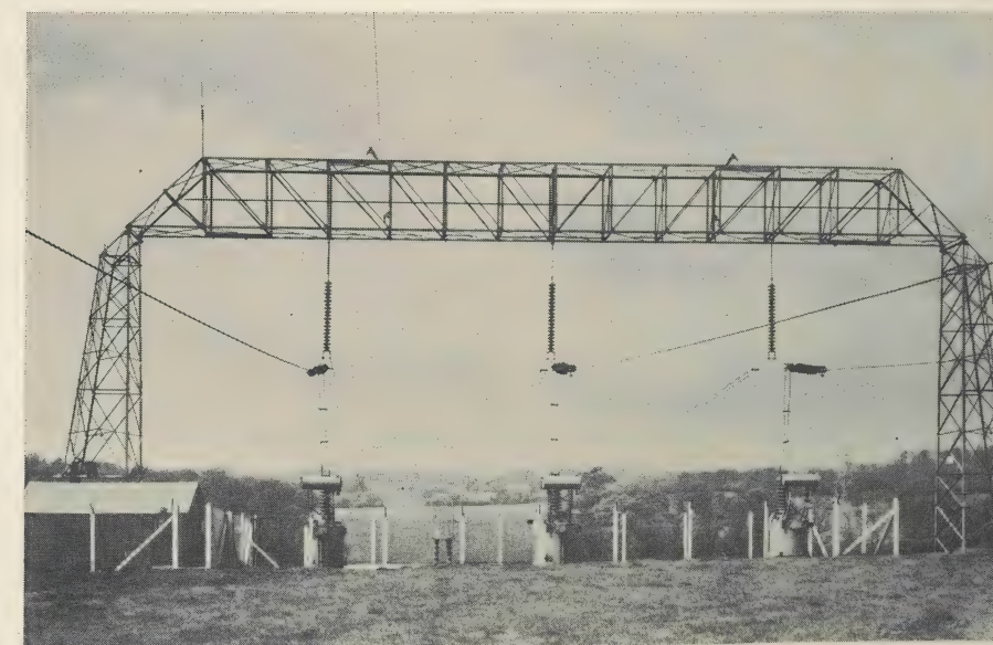
Fig. 4. High-voltage experimental transmission line.
