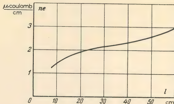
Fig. 2 Distribution of the excess positive charge along the leader (for the discharge of Fig. 1).
