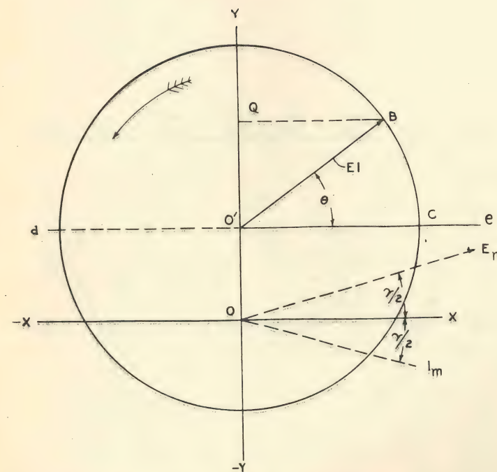
Figure 4. Vector diagram of imaginary power in an inductive circuit.
