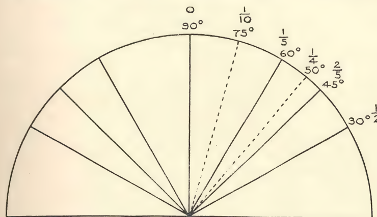
FIG. 3.—DIAGRAM SHOWING COMPENSATORY TIME INCREMENTS FOR VARIOUS ANGLES OF INCIDENCE OF THE RAYS.
