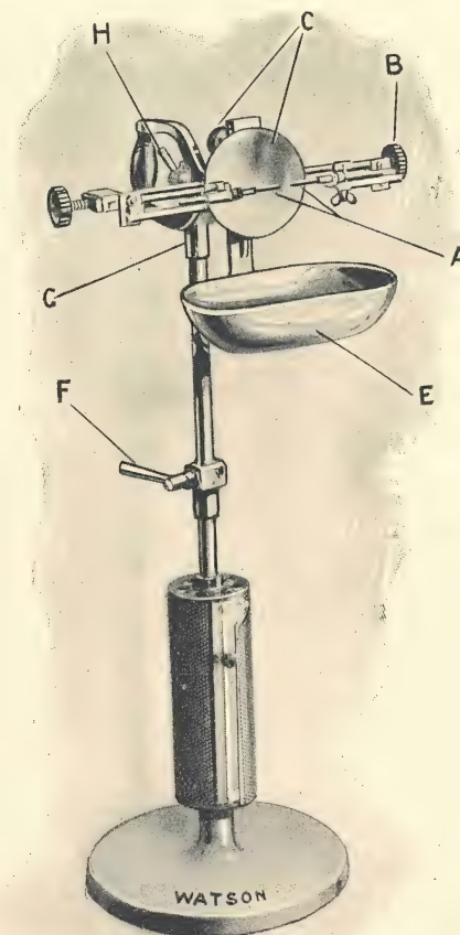
FIG. 9.—TUNGSTEN ARC LAMP AS DESIGNED BY DR. PERCY HALL.
