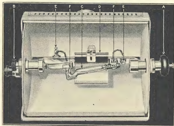
FIG. 6.—AIR-COOLED QUARTZ LAMP. (The Victor Corporation, U.S.A.)
