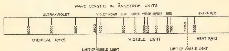
FIG. 2.—DIAGRAM OF THE SPECTRUM.
