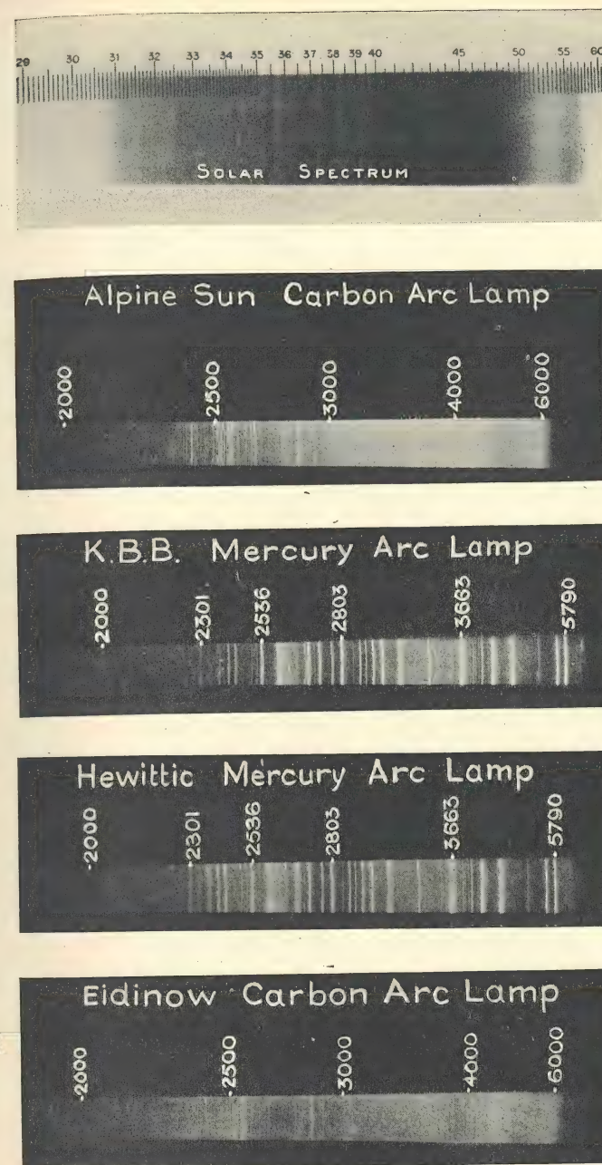
FIG. 13.—SPECTROGRAMS SHOWING COMPARISON BETWEEN THE SOLAR SPECTRUM AND THE SPECTRA GIVEN BY THE MERCURY VAPOUR AND THE CARBON ARC LAMPS.
