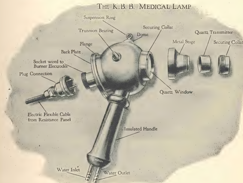
FIG. 5.—THE WATER-COOLED MERCURY VAPOUR ARC LAMP; SHOWING PARTS.
