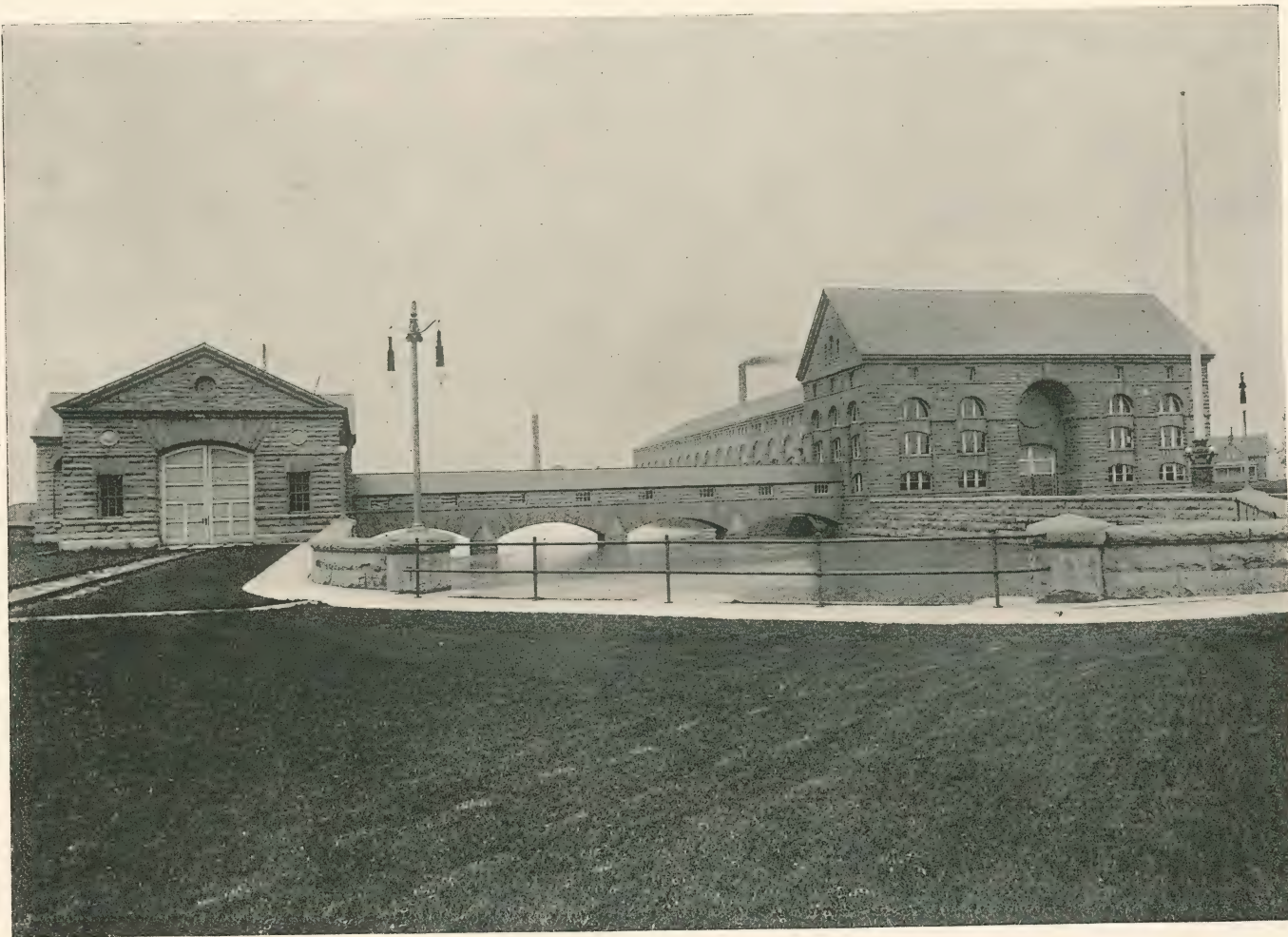
NIAGARA FALLS POWER COMPANY'S PLANT — Where the energy which for centuries has been going to waste has now been harnessed for the service of mankind.
