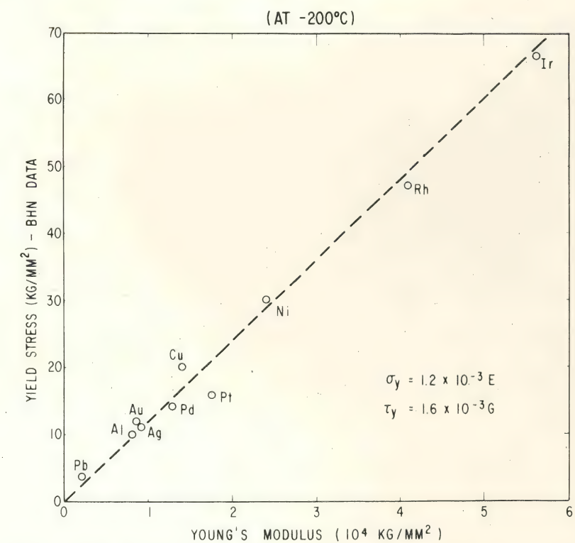
Fig. 17 Relation of yield stress to elastic modulus for face-centered cubic metals.
