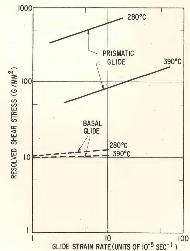
Fig. 6 Translation gliding in the close-packed direction is more difficult on the prism planes of zinc crystals than on their basal plane.
