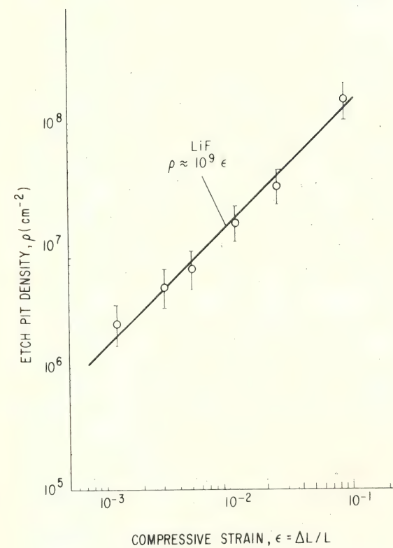
Fig. 22 Average dislocation density vs plastic strain for a typical LiF crystal.
