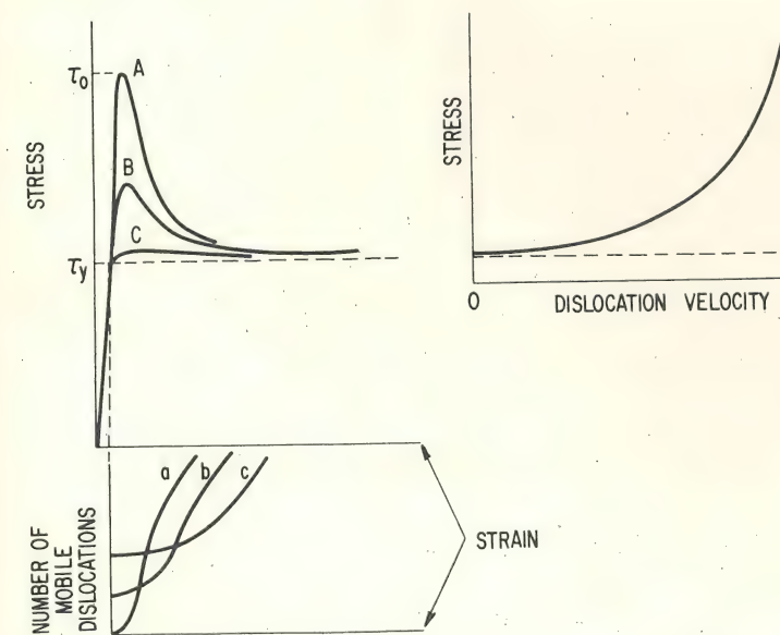
Fig. 24 Interpretation of plastic instability at yield point.
