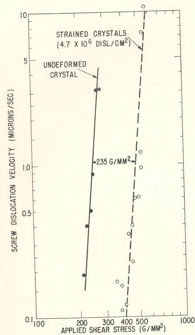
Fig. 14 Effect of strain-hardening on mobility of dislocations in lithium fluoride crystals.
