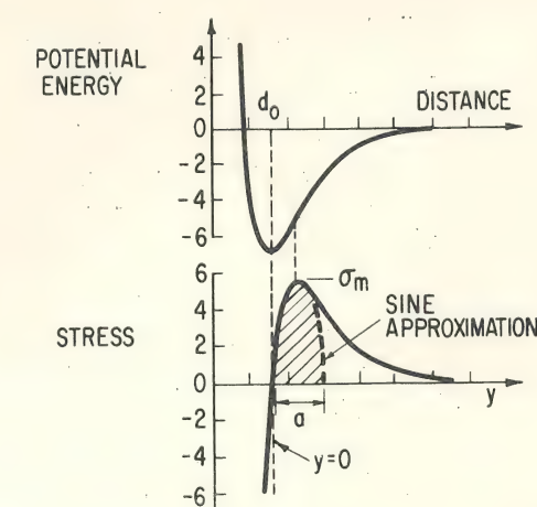
Fig. 25 Schematic energy and stress between two adjacent planes of a crystal.
