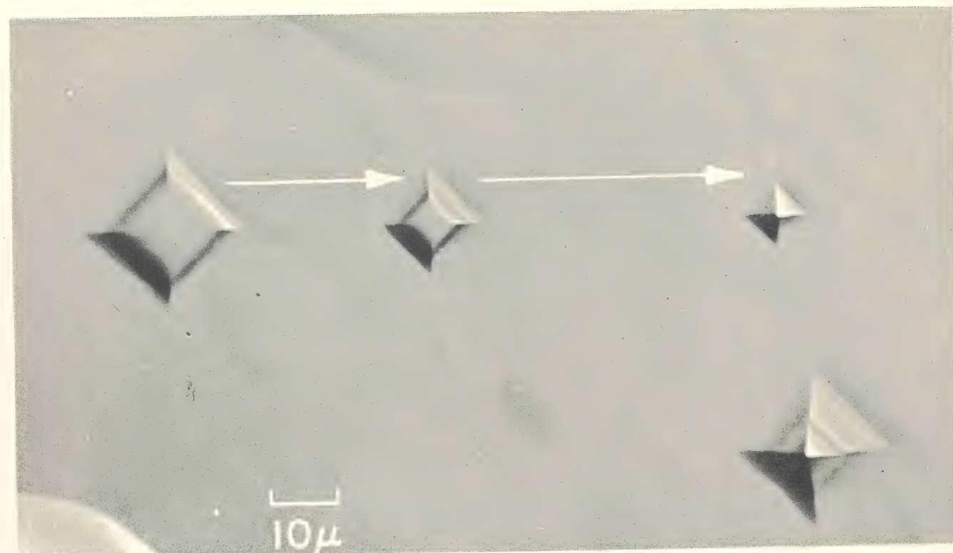
Fig. 11 Glide of an isolated dislocation in a lithium fluoride crystal revealed by etch-pits (after Gilman and Johnston). The crystal was etched to show the initial dislocation position; then a stress was applied to move the dislocation, and the crystal was re-etched to show the new position of the dislocation some more, and the crystal was etched a third time to show the final position of the dislocation. The arrows indicate the direction of motion.
