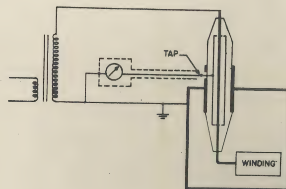
Figure 6. Simplified Circuit Diagram of Ungrounded Specimen Test on Transformer Bushing
