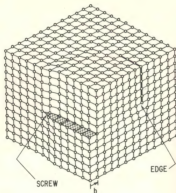
Fig. 4 Distortions of a crystal near the screw and edge orientations of a dislocation line.
