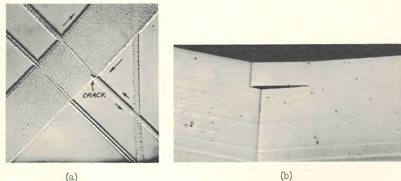
Fig. 30 Examples of cracks that were produced by plastic deformation: (a) crack in MgO crystal (courtesy W.G. Johnston); example of cracking by mechanism of Fig. 26(c); (b) crack in Zn crystal; example of cracking by mechanism of Fig. 26(b) (after Gilman).
