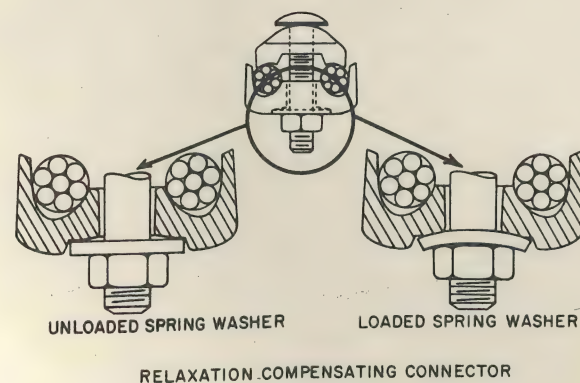
Fig. 5. Relaxation compensating connector
