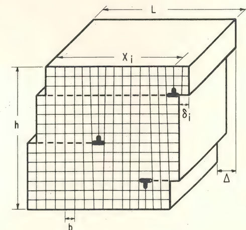
Fig. 2 The strain caused by dislocations.
