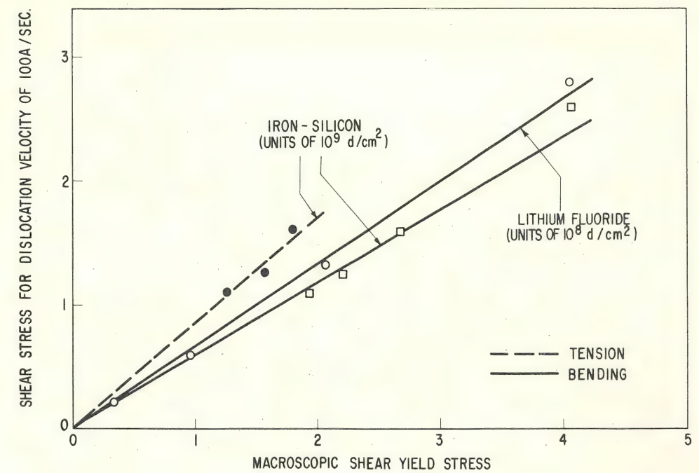
Fig. 16 Correlation between stress to cause dislocation motion and the macro-yield stresses of crystals.
