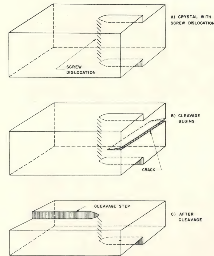
Fig. 34 Cleavage step formation by the intersection of a crack with a screw dislocation.
