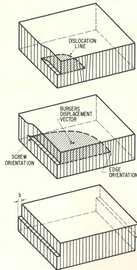
Fig. 1 Spread of translation gliding across a crystal.
