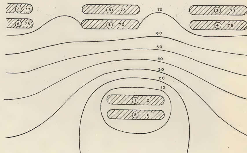
Figure 6. Magnetic flux lines in a portion of a pulse transformer winding. An uncircled number denotes flux linkage with respect to conductor number one. As very little flux penetrates a conductor under pulse conditions, this number is constant for each conductor.
