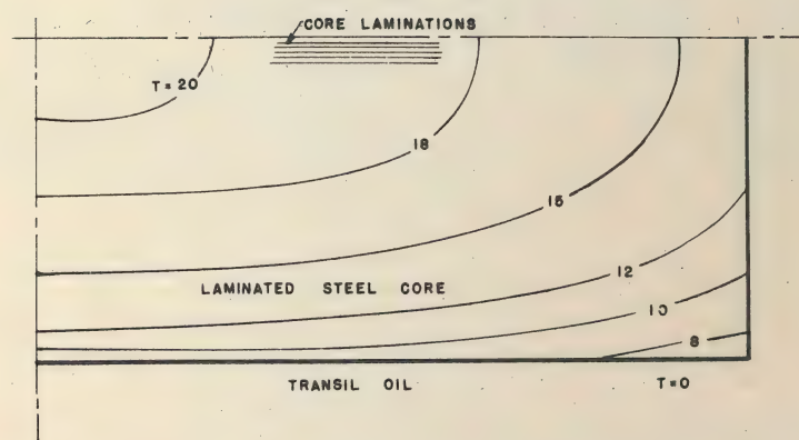
Figure 9. Temperatures in a cross section through one quarter of a transformer core. The contours are isothermal lines representing the temperature rise T in degree C with respect to the surrounding oil. No isothermal lines appear in the oil which is at a uniform temperature ( T=0 ).
