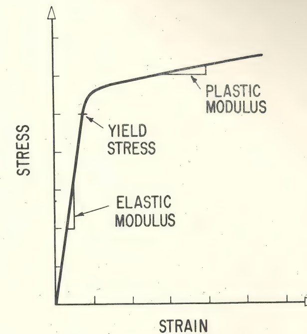
Fig. 23 General form of stress-strain curves.
