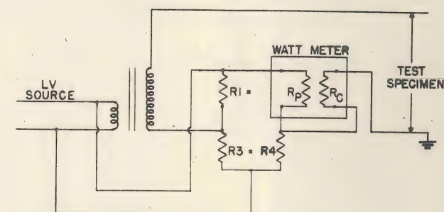
Figure 2. Compensated Wattmeter Circuit
