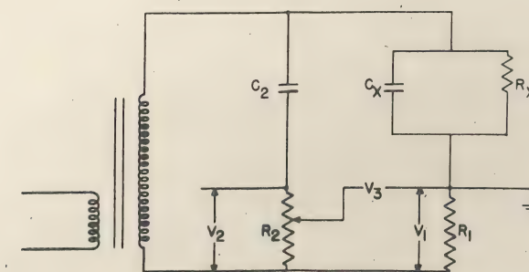
Figure 3. Simplified Circuit Diagram - Component Separation Method
