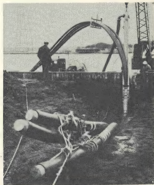
HYDRO-JETTER UNIT: 1-water-pressure hose; 2-injector; 3-plastic conduit to be embedded in river bottom; 4-winch line; 5-free-running conduit coils
