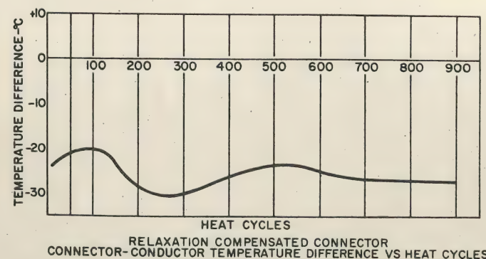
Fig. 6. Relaxation compensated connector
