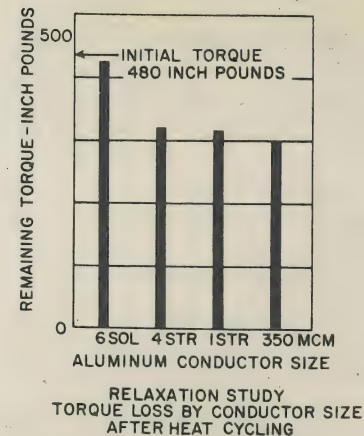
Fig. 2. Torque loss by conductor size after heat cycling
