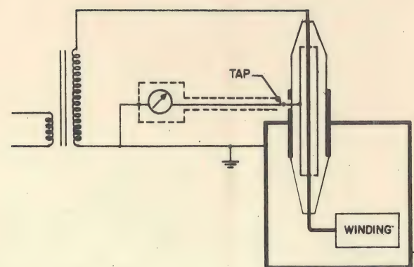
Figure 6. Simplified Circuit Diagram of Ungrounded Specimen Test on Transformer Bushing
