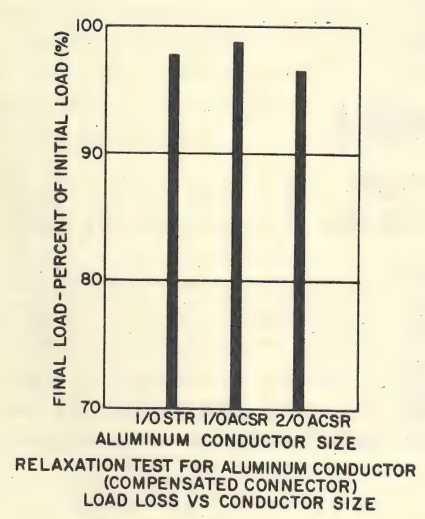
Fig. 3. Relaxation test for aluminum conductor (compensated connector)
