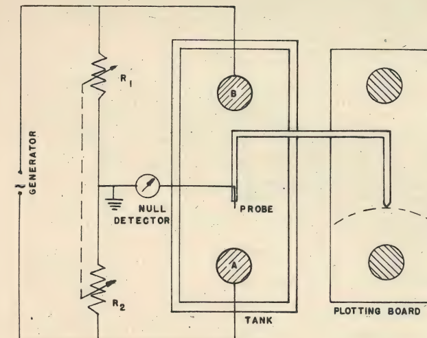
Figure 1. Elements of the Electrolytic Field-Analyzer. The model consists of tank, electrolyte and the electrodes A and B.
