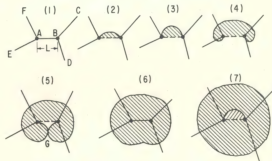
Fig. 18 Multiplication of dislocations via a Frank-Read source.
