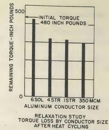
Fig. 2. Torque loss by conductor size after heat cycling
