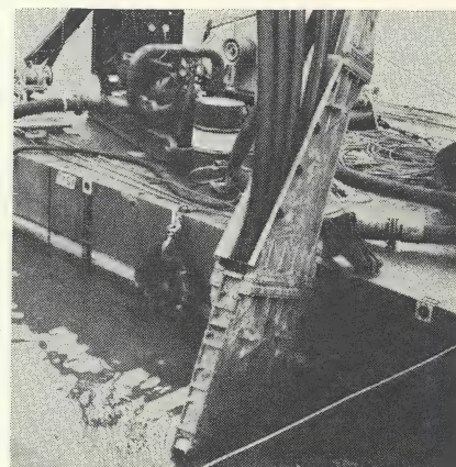
INJECTOR , including high-pressure water section, conduit guide section and jet nozzles, is depth-controlled
