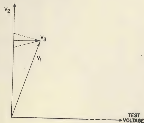
Figure 4. Phasor Diagram - Component Separation Method
