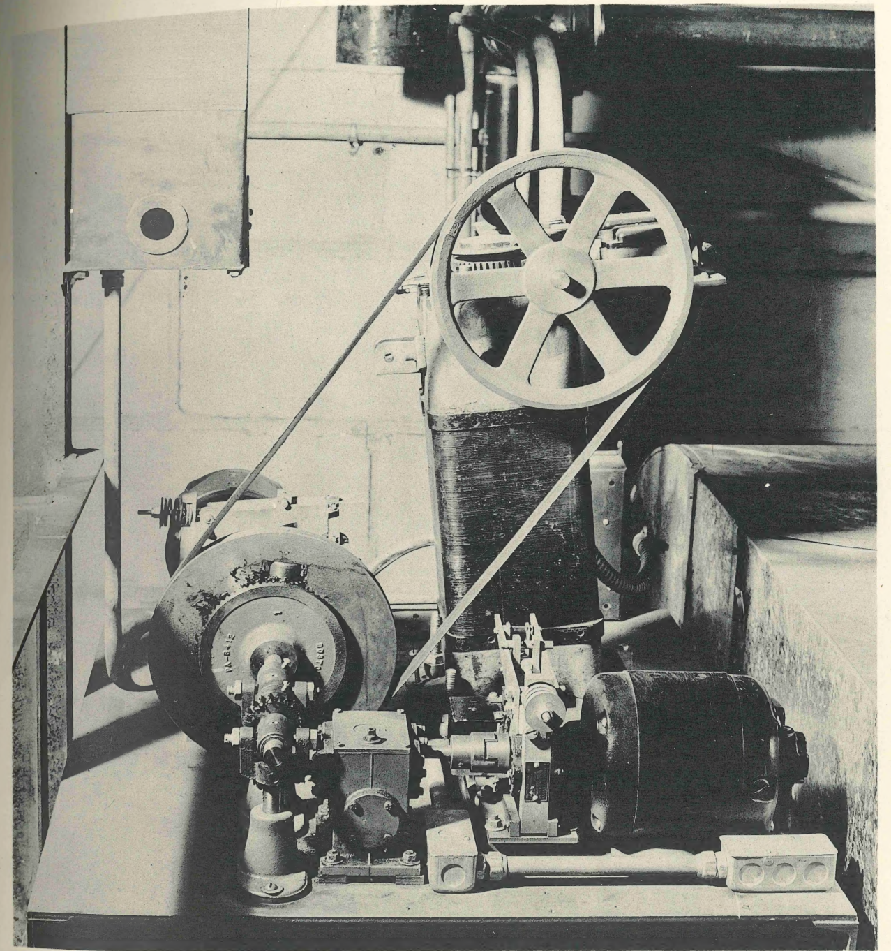
FIG. 2 - MOTOR DRIVE UNIT OF ADJUSTABLE RATE OF RISE CONTROL SYSTEM FOR DIELECTRIC STRENGTH TESTING
