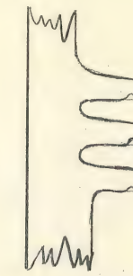
Unit B Hoods - 18 Flashover Length - 29" Leakage Length - 95"
