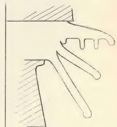
7785 Cap & Pin Insulator Hoods - 3 Flashover Length - 14-1/2" Leakage Length - 33"
