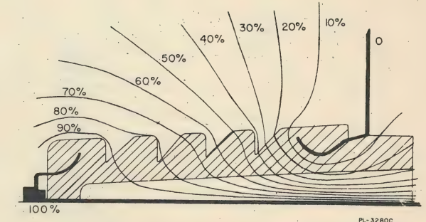
Figure 3. Potential field of a glass bushing obtained with the electrolytic field-analyzer. The contours are equipotential lines with the voltage of each indicated as a percentage of the total applied voltage.
