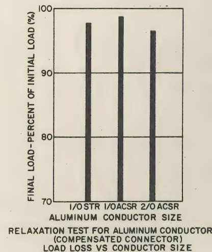
Fig. 3. Relaxation test for aluminum conductor (compensated connector)
