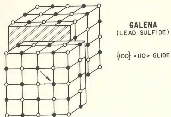
Fig. 7 Translation-gliding in the same direction, but on two different planes in crystals with the rocksalt structure.
