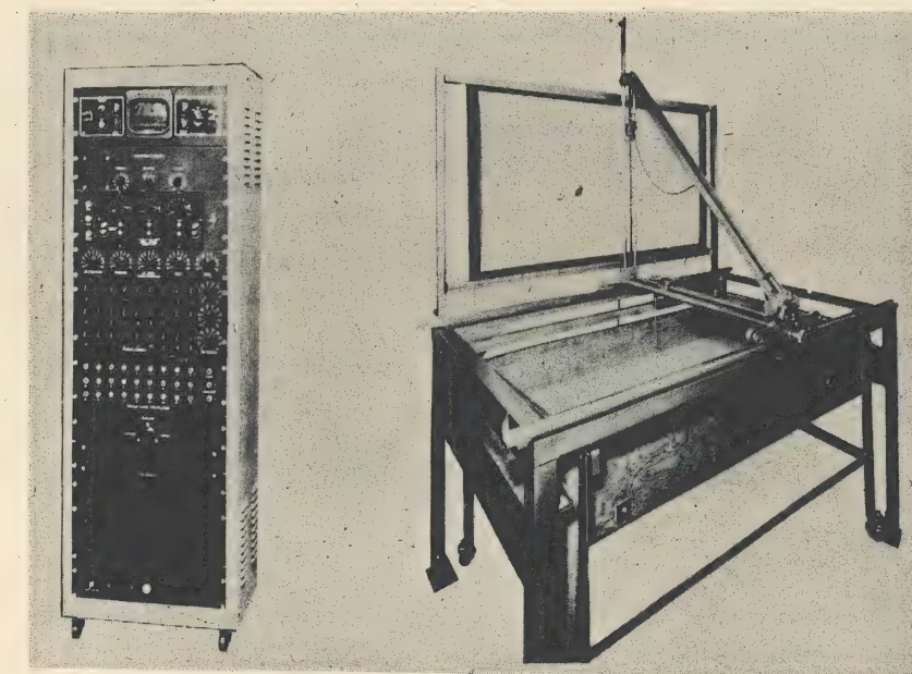
Figure 2. Equipment for field analysis
