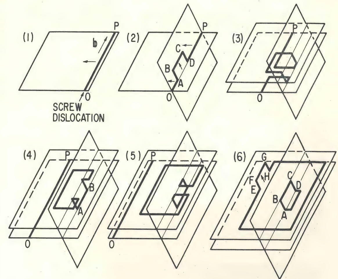
Fig. 20 Multiplication of dislocations via multiple cross-glide.
