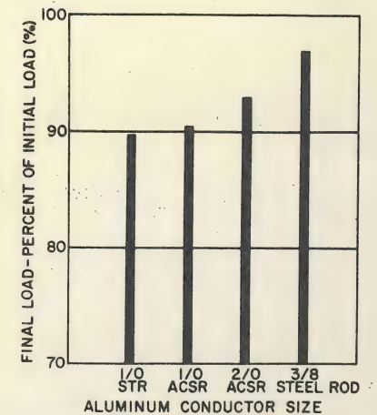
RELAXATION TEST FOR ALUMINUM CONDUCTOR (NON-COMPENSATED CONNECTOR) LOAD LOSS VS CONDUCTOR SIZE
