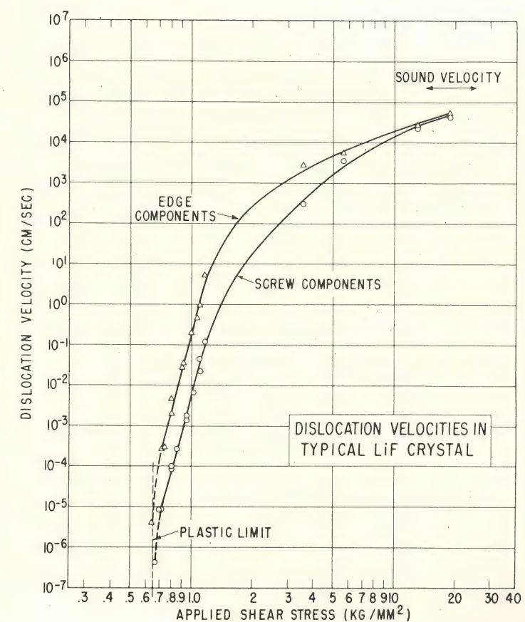
Fig. 12 Dislocation velocities in typical LiF crystal.
