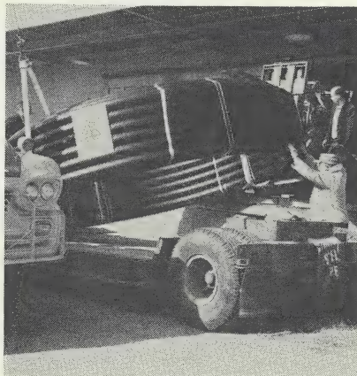
PLASTIC CONDUIT , in 750-ft lengths, is shipped to work-site in 14-ft OD coils on over-the-road flat-bed-trailers
