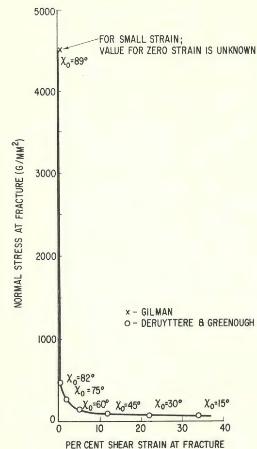
Fig. 29 Effect of glide strain on fracture stress of zinc crystals (at -196^\circ\text{C} ).
