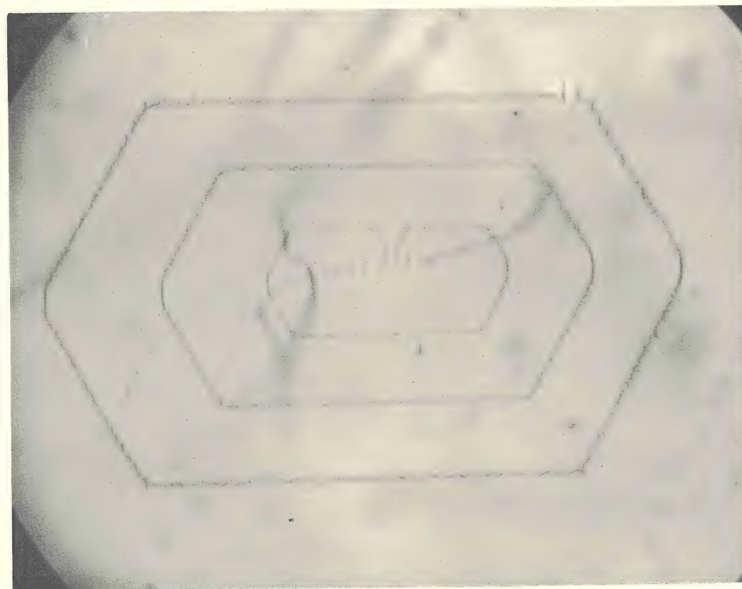
Fig. 19 A Frank-Read source seen in plastically deformed silicon. Copper precipitates reveal the dislocation lines. The dislocations lie on the (111) plane of silicon (Courtesy of W.C. Dash). 400X
