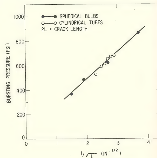
Fig. 32 Griffith's data for stresses required to propagate cracks in glass.
