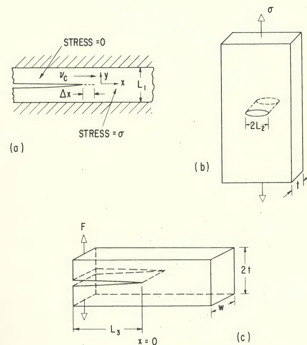
Fig. 31 Some schematic configurations of cracks in solids.
