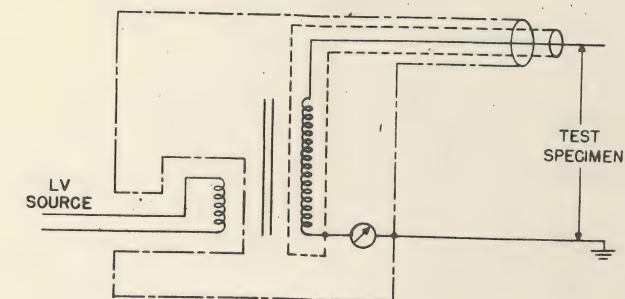
Figure 1. Double Shielded Measurement System
