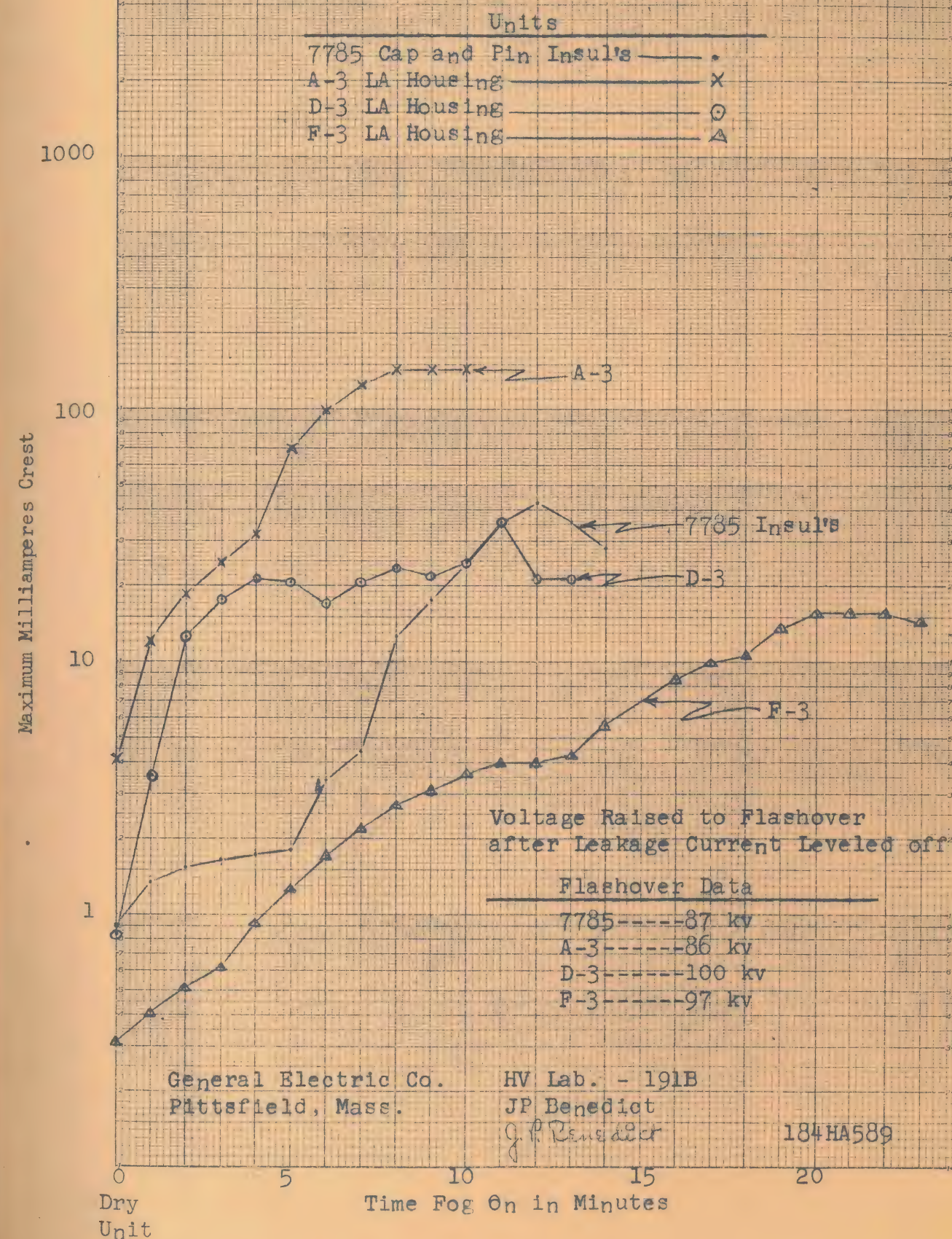
Figure 4 Leakage Current at 50 kv for Contaminated Units under Fog Condition
