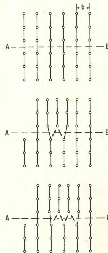
Fig. 9 Balanced forces at a moving dislocation.
