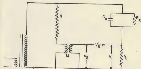
Figure 5. Component Separation Circuit with Mutual Inductor
