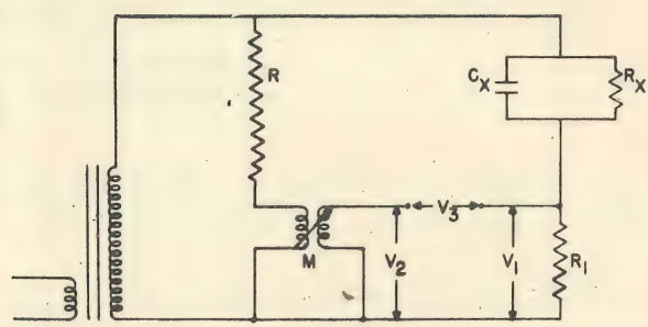
Figure 5. Component Separation Circuit with Mutual Inductor
