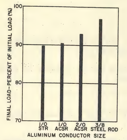
Fig. 1. Relaxation test for aluminum conductor (non-compensated connector)
