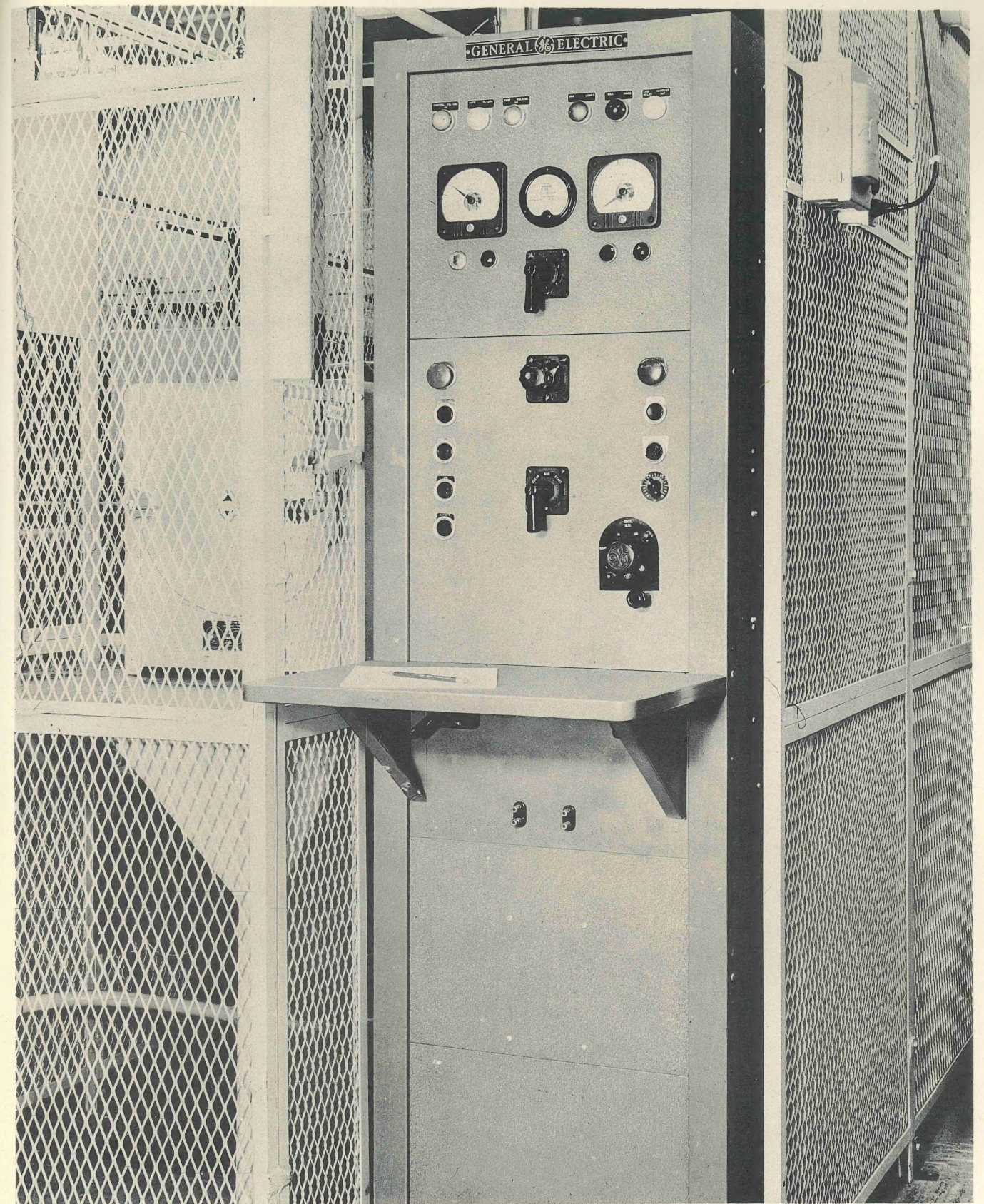
FIG. 3 - CONTROL CABINET OF ADJUSTABLE RATE OF RISE CONTROL SYSTEM FOR DIELECTRIC STRENGTH TESTING
