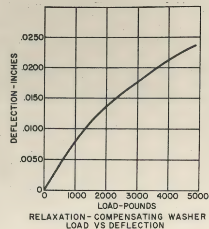
Fig. 4. Relaxation compensating washer
