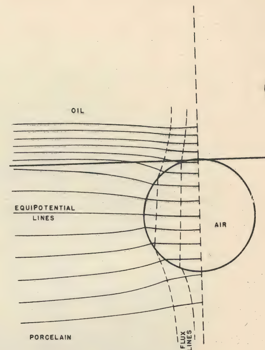
Figure 5. The electrostatic field about a gas inclusion in porcelain near oil. Different models were used for the two types of lines.
