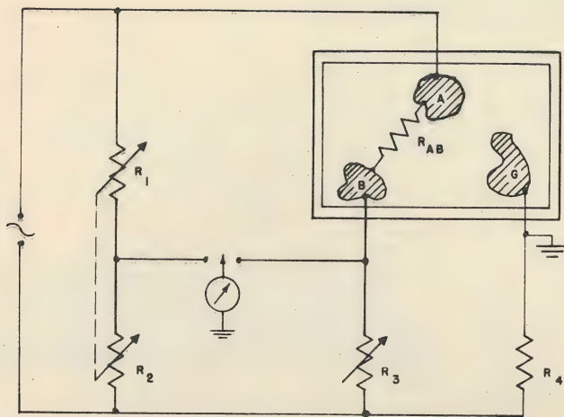
Figure 4. Guarded bridge circuit used with an electrolytic model for the determination of the partial capacitance between electrodes A and B.
