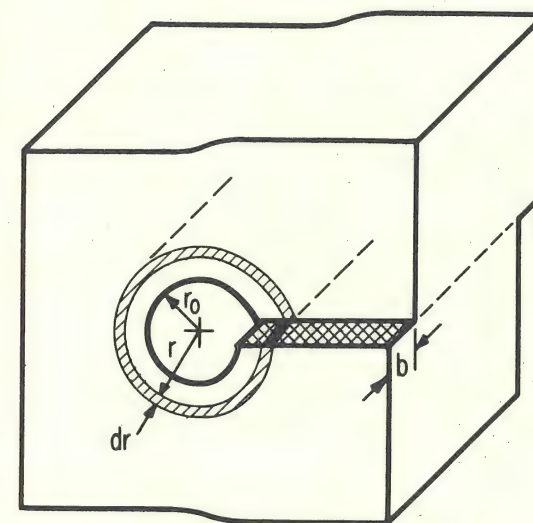
Fig. 5 Strained elastic shell around a screw dislocation.
