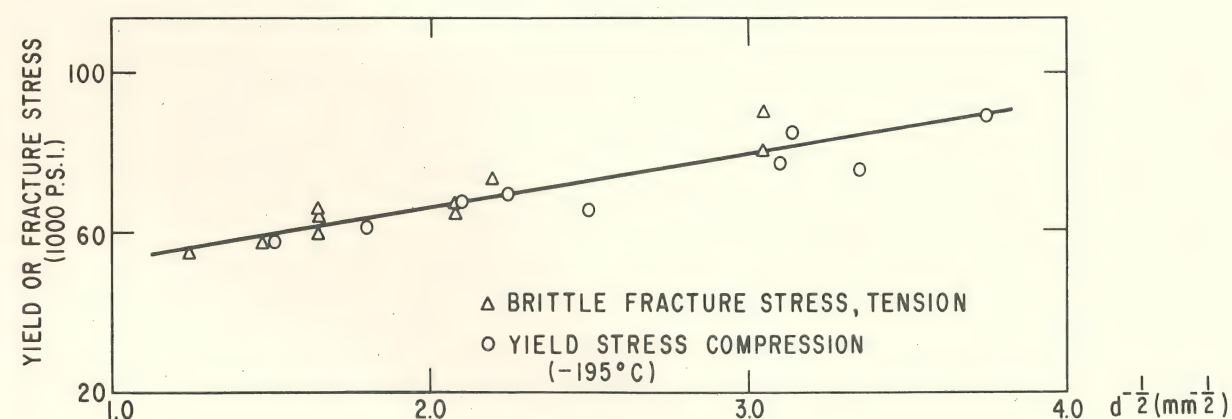
Fig. 28 Equality of fracture stress (tension) and yield stress (compression) for mild steel specimens of various grain sizes (after Low).
