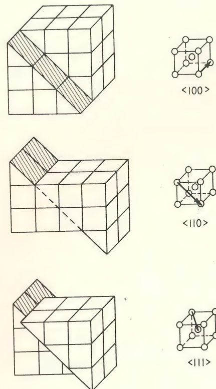
Fig. 3 Three possible glide directions in iron--the shortest one, \langle 111 \rangle , is preferred.
