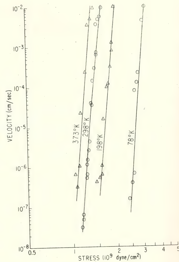
Fig. 15 Edge dislocation motions in Fe - 3 per cent Si crystals (Stein and Low).
