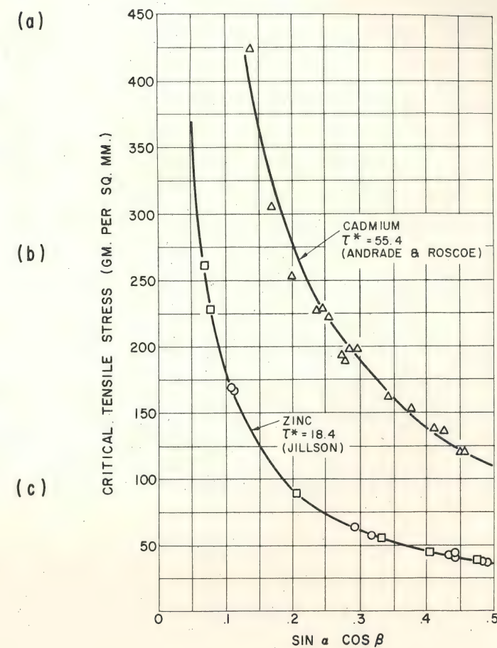
Fig. 10 Tensile stresses required to cause plastic flow in zinc and cadmium crystals as a function of orientation angles (Jillson, Andrade, and Roscoe).
