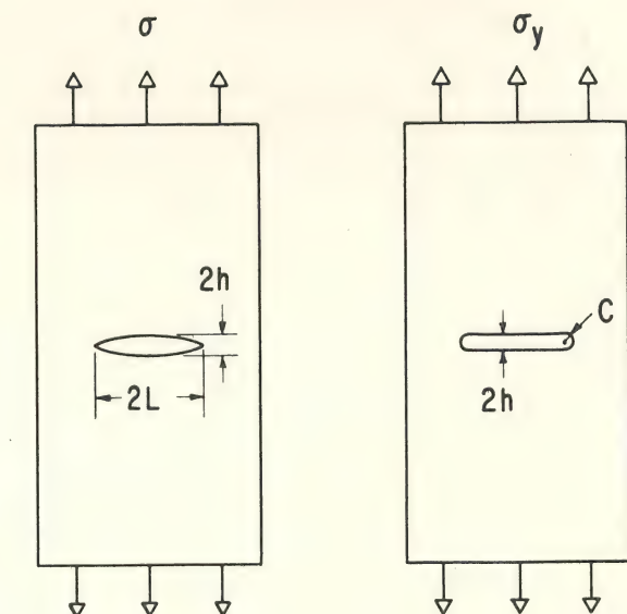
Fig. 35 Effect of plastic relaxation on the shape of a crack.
