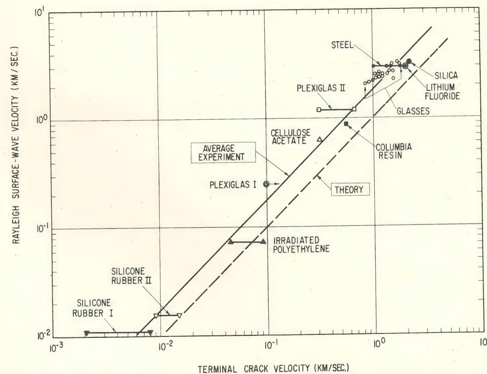
Fig. 33 Approximate equality of terminal crack velocities and sound wave velocities in various solids.
