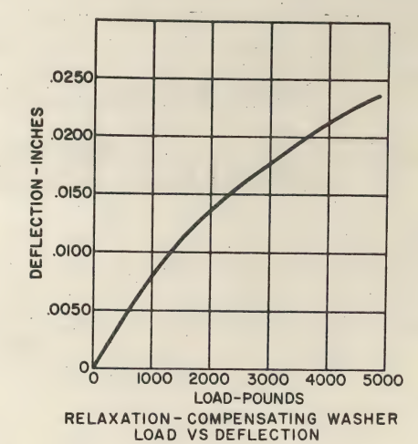
Fig. 4. Relaxation compensating washer
