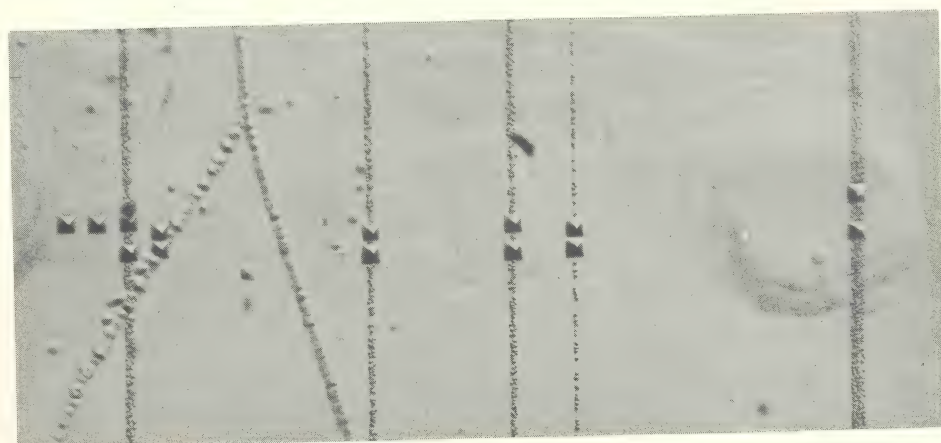
Fig. 21 Dislocation multiplication in a LiF crystal (after Gilman and Johnston): (a) dislocation half-loops at the surface; (b) same area after crystal had been bent; glide steps pass through five of the pairs of pits; (c) same area after light etch; showing many pits at each glide step.
