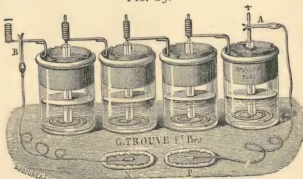
Four Callaud-Trouvé gravitation elements arranged in series.
