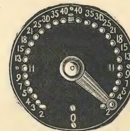
Dial collector arranged for starting from either end of the battery.
