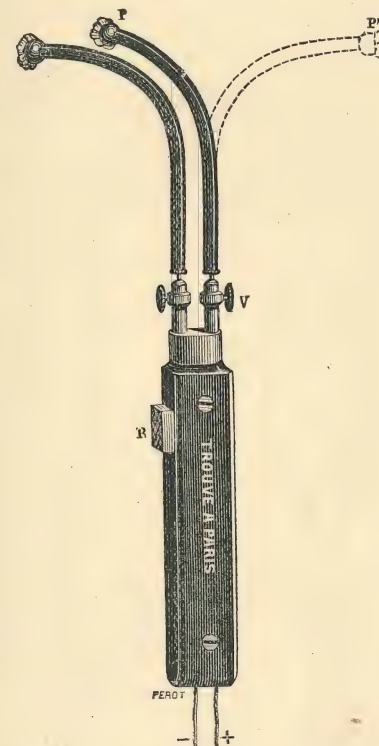
Trouvé's bipolar electrode.
