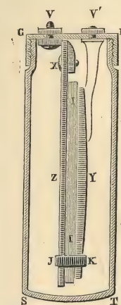
GAIFFE'S CHLORIDE OF SILVER ELEMENT.
