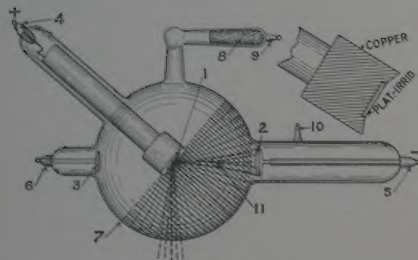
CHART OF AN X-RAY TUBE.
