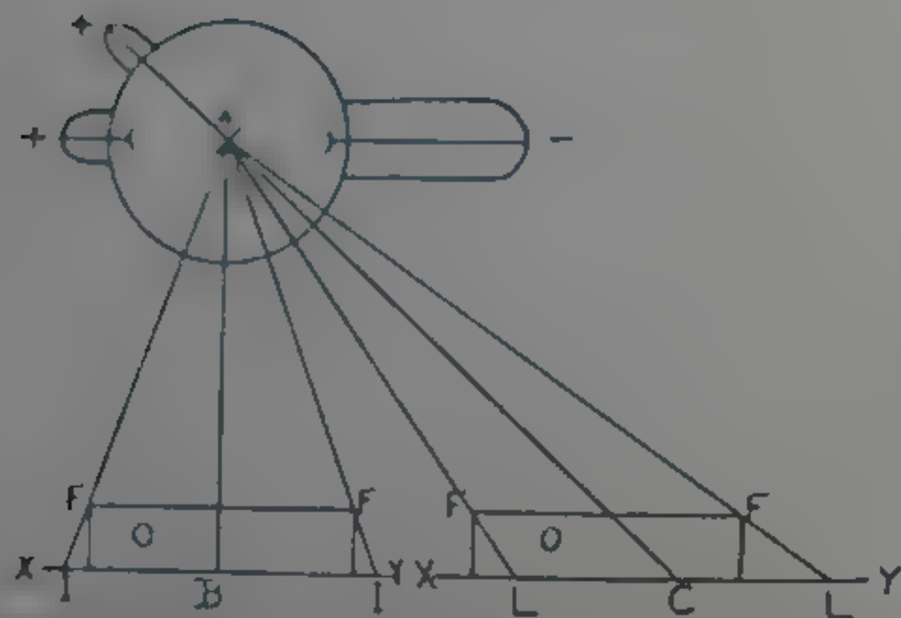
FIGURE 1. Shows How to Place the Plate to Obtain a Proper Image. (See Page 91.) The Lower Illustration Shows How the Object O is Magnified but Not Distorted if the Central Ray AB is Perpendicular to the Center of O and XY. If the Ray (AC) is Not Perpendicular the Points FF Appear at LL Thus Producing a Distorted Image.
