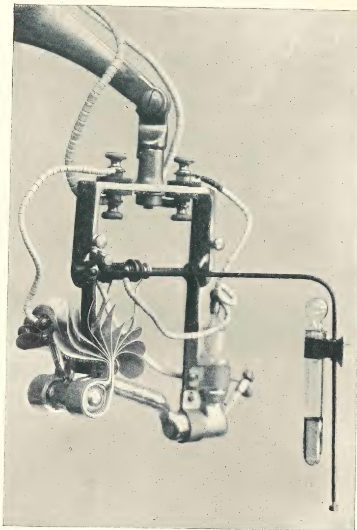
FIG. 30.—KING'S ACTINOMETER: THE 250-VOLT ATMOSPHERIC QUARTZ MERCURY VAPOUR LAMP IN ITS HOLDER AT THE END OF THE ARM OF THE STAND
