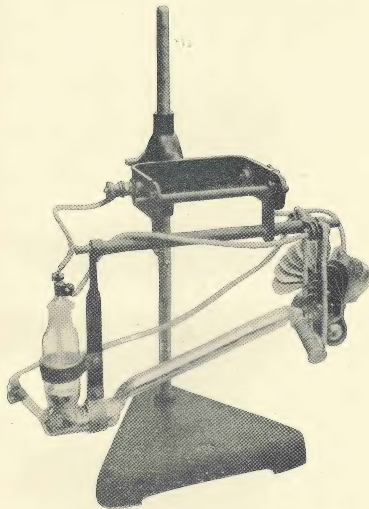
FIG. 24.—AIR-COOLED ATMOSPHERIC TYPE BURNER. K.B.B. 440-VOLT PATTERN.
