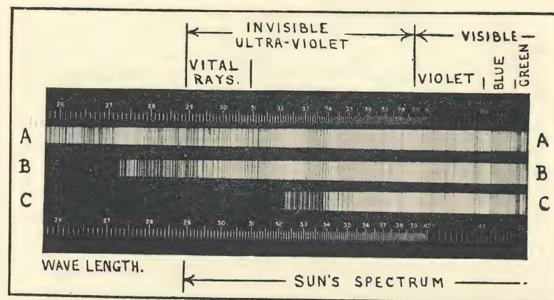
FIG. 15.—Spectrum photograph, illustrating the composition of light from an electric arc between iron poles, taken by the Hilger Quartz Spectrograph, with wave-length scale.
