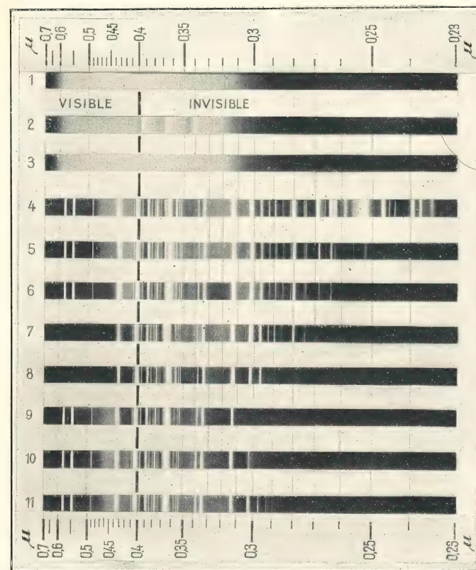
FIG 2.—SPECTRA OF DIFFERENT SOURCES OF LIGHT The spectra shown were obtained from exposures of similar negatives for the same time.
