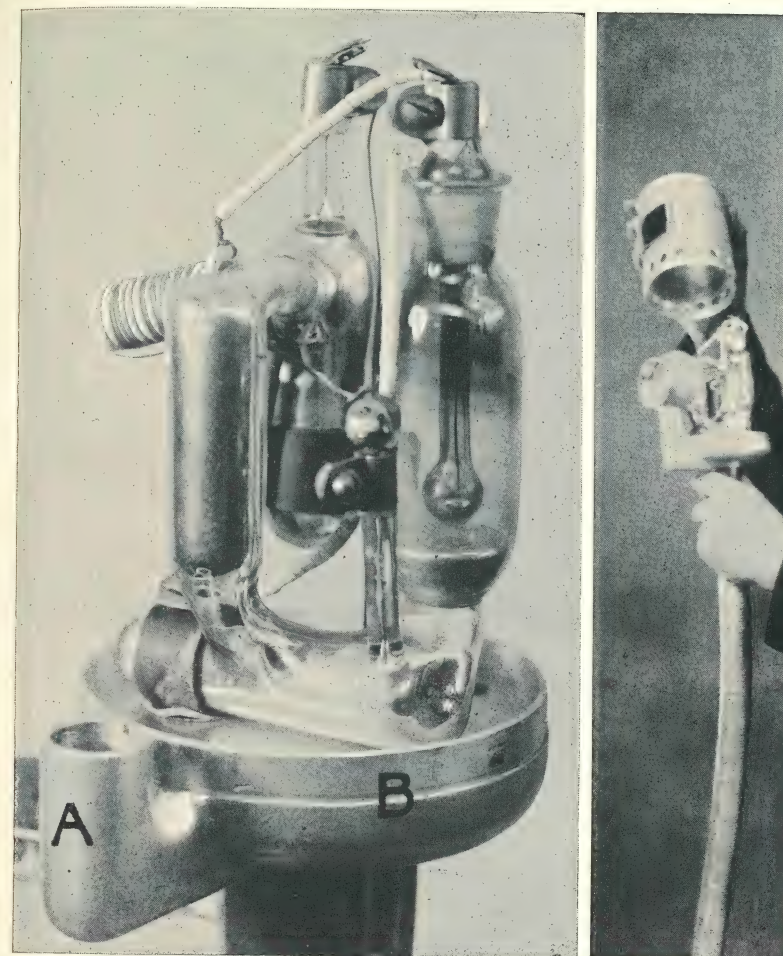
FIG. 28.—ATMOSPHERIC TYPE MERCURY VAPOUR ARC LAMP COOLED BY FORCED DRAUGHT
