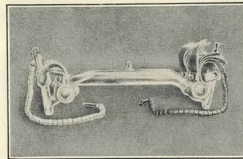
FIG. 22.—AIR-COOLED VACUUM TYPE BURNER (HANOVIA). DIRECT CURRENT.
