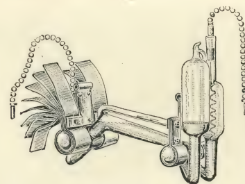
FIG. 33.—"MONTANA" BURNER: TYPE B. 220 VOLTS, 3 AMPS., AUTOMATIC STARTING.
