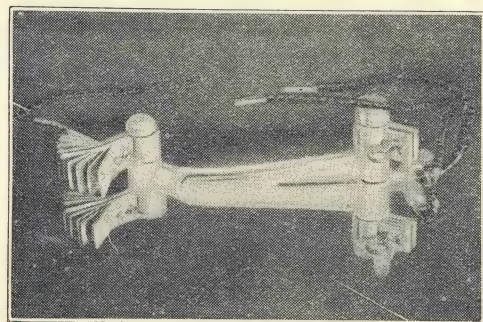
FIG. 23.—AIR-COOLED VACUUM TYPE BURNER (HANOVIA). ALTERNATING CURRENT, SHOWING DOUBLE POSITIVE POLE.
