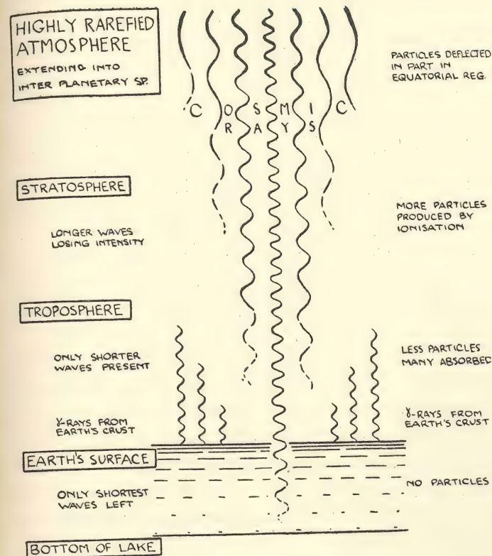
DIAGRAM SHOWING THE GRADUAL ABSORPTION OF COSMIC RAYS IN THE ATMOSPHERE AND IN WATER
