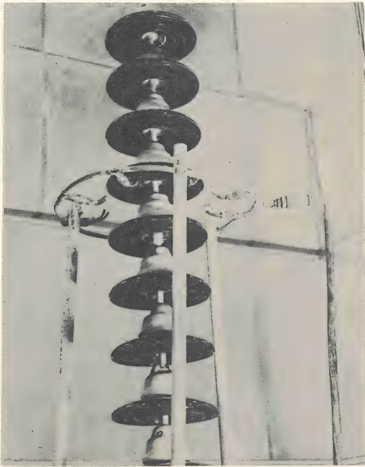
Fig. 1. Apparatus for Flow-coating Suspension Insulators.
