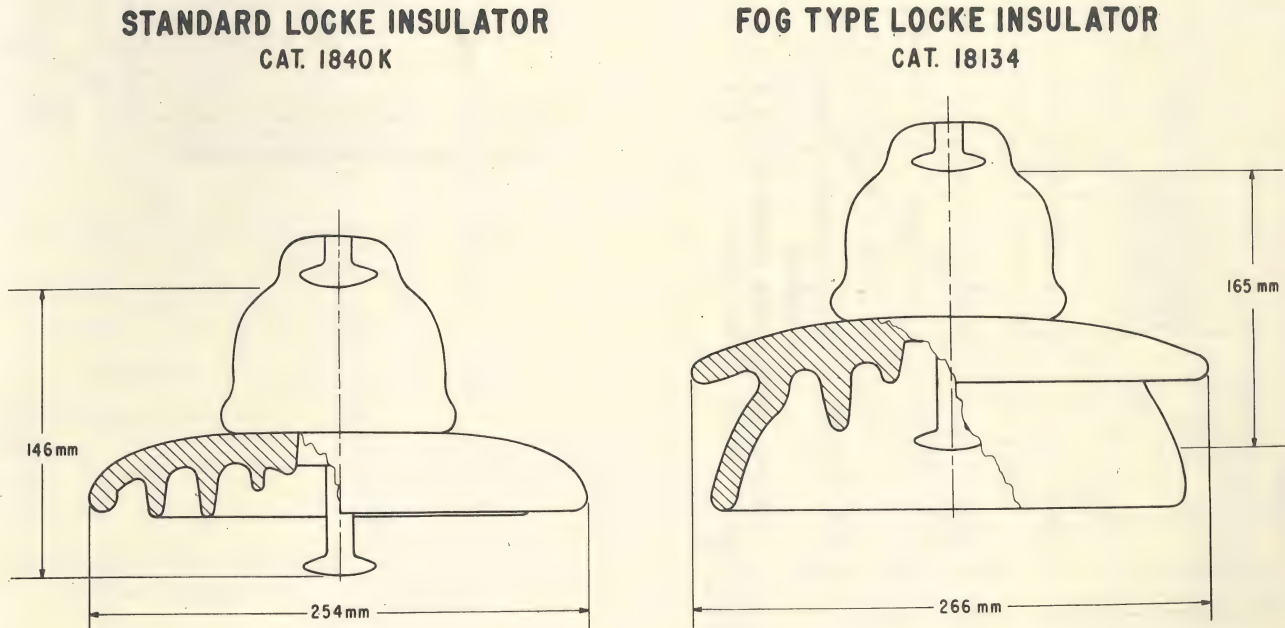
Fig. 3. Test Insulators.
