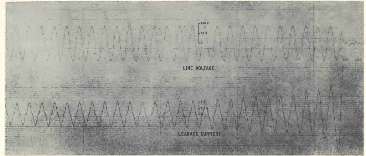
Fig. 14. Applied Voltage and Leakage Current Record: Test with Flashover Showing Wave Distortion.
