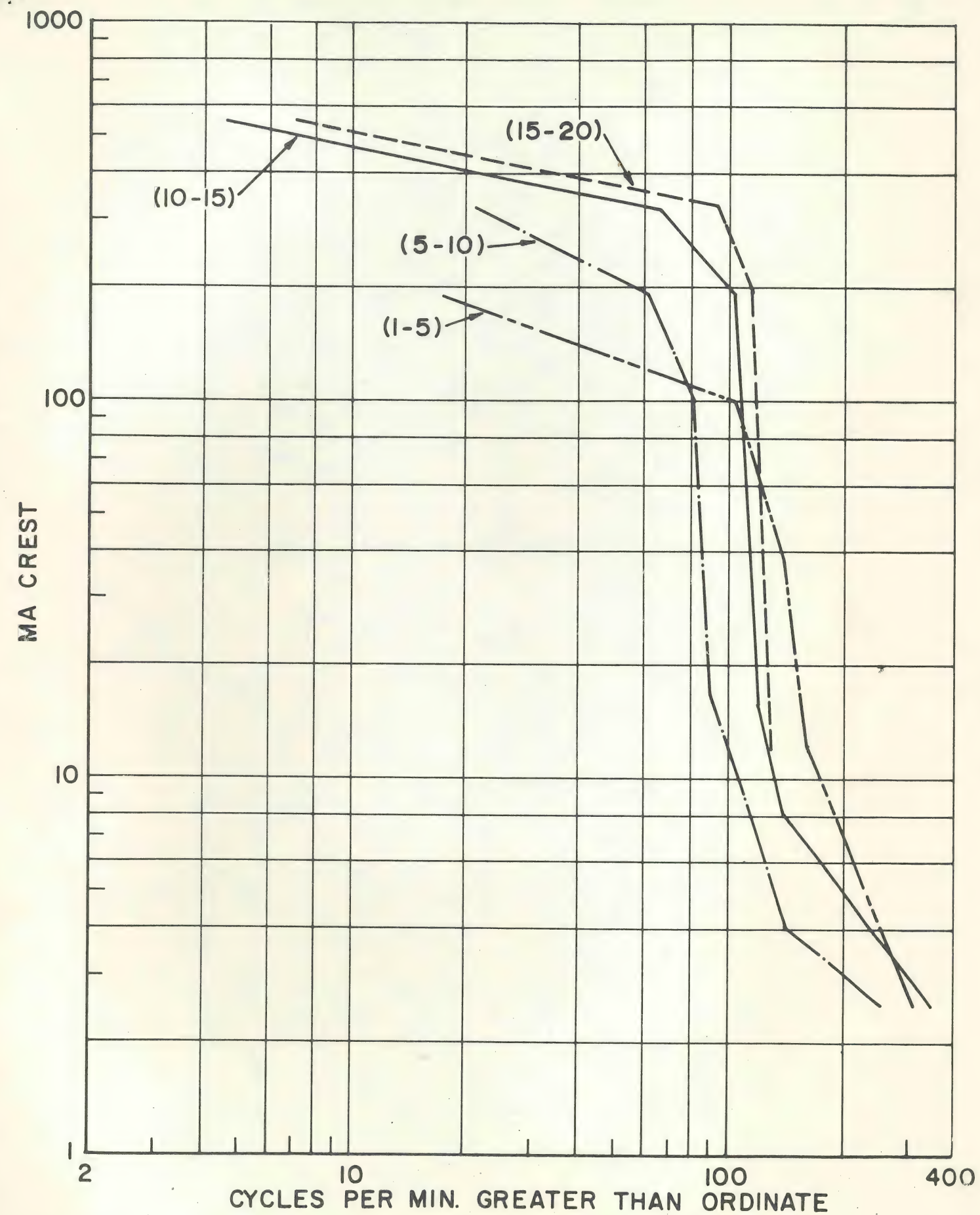
Figure 8. Surge analysis - 15 vee insulators with 0.2% salt contamination. Curve designations are time period in minutes, measured from start of fog.
