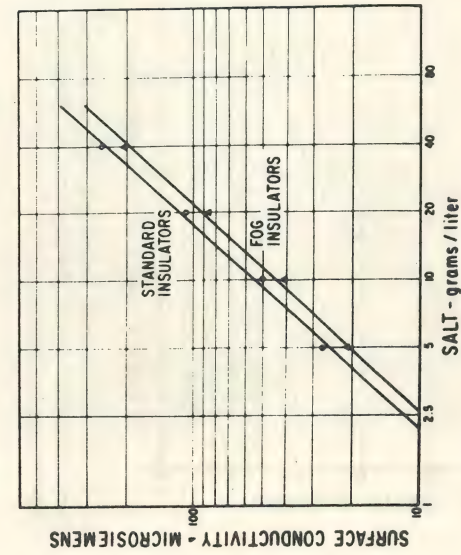
Fig. 10. Initial Surface Conductivity Versus the Salt in the Mixture for Standard and Fog-type Insulators.
