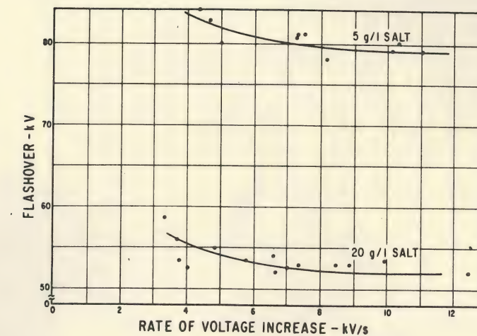
Fig. 18. Flashover Voltage Versus Rate of Voltage Increase for Slurries with Two Different Salt Con- centrations.
