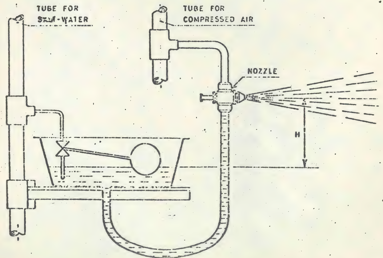
FIG. 6 ARRANGEMENT FOR PRODUCING FOG
