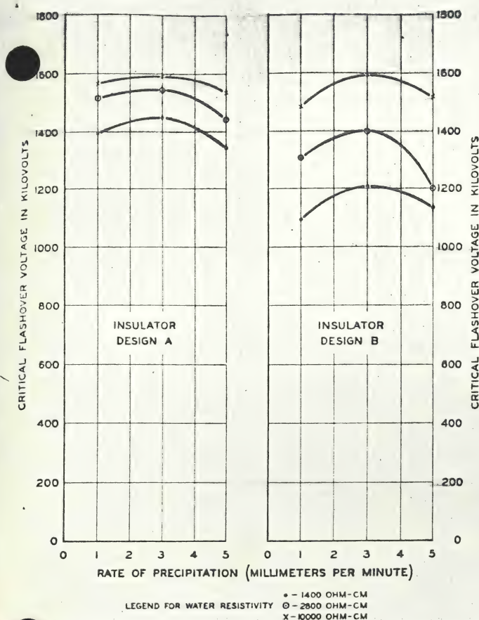
1. Influence of rainfall rate on critical (50 percent probability) flashover voltage for positive polarity switching surge, 181-inch insulators.
