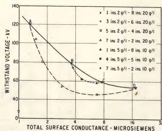
Fig. 8. Non-uniform Distribution of the Contaminant in the String. Withstand Voltages Versus the Total Surface Conductance. The Letters A, B, C, D Represent the Points Obtained for Uniform Slurry Coatings of 2, 5, 10 and 20 g/l Salt Respectively.
