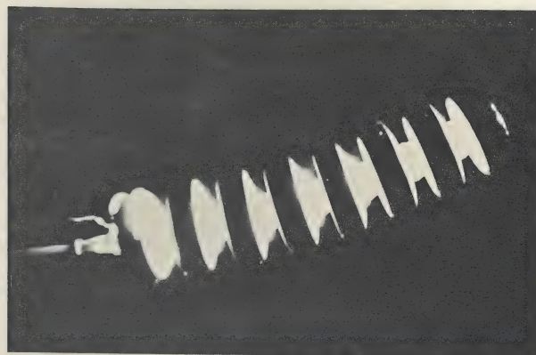
Fig. 16. Horizontal Fog Unit String During a Withstand Test.
