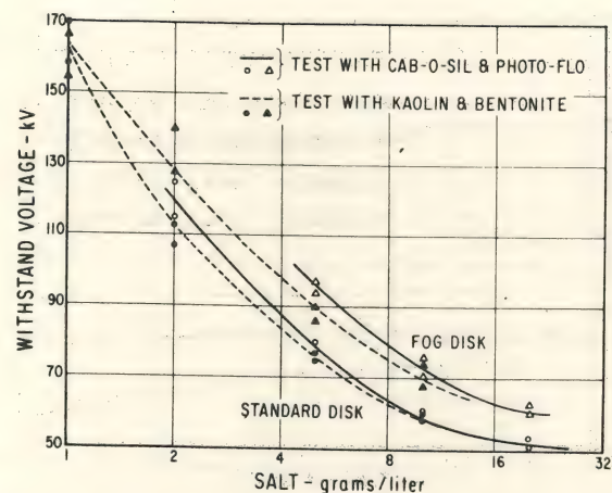
Fig. 7. Comparisons with Different Slurries. Withstand Voltages Versus the Salt in the Mixture.
