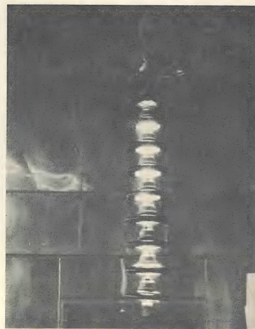
Fig. 17. Scintillation on Standard Insulator String During a Withstand Test.
