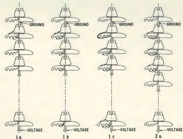
Fig. 9. Visual Observed Mechanism During Withstand Tests with Non-uniform Distribution of the Contaminant in the String:
