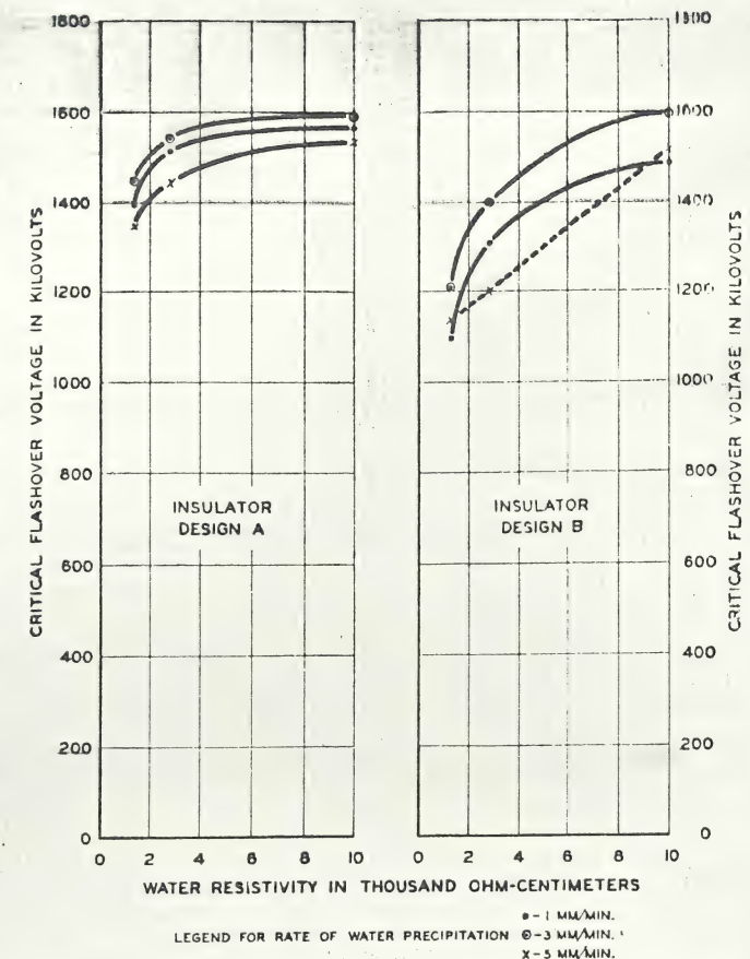
Fig. 2. Influence of water resistivity on critical (50 percent probability) flashover voltage for positive polarity switching surge, 181-inch insulators.
