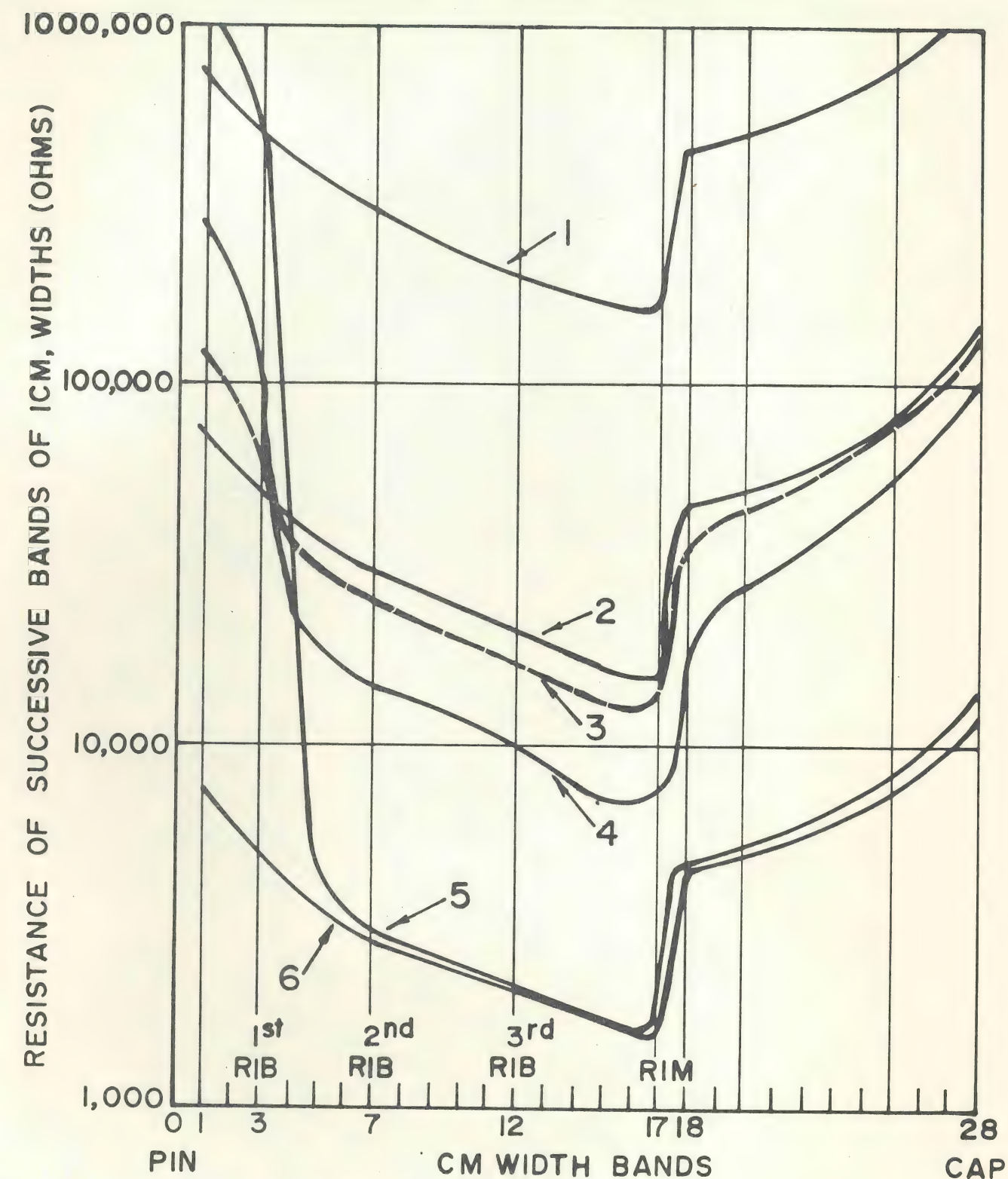
Fig. 14. Resistance of centimeter width bands on a contaminated insulator versus distance in centimeters from the pin (0) to the cap (28) (1) Approximate dry pollution with no current (2) Partially wet resistance 8 minutes after fog start. No current (3) Distortion by current heating in pin and cap area. (4) Further distortion by accelerated heating in pin area. (5) Prior to F/O. Very high resistance at pin. Current very low. Path away from pin tending towards fully wet resistance. (6) Fully wet resistance, total approximately 130,000 ohms. No current.
