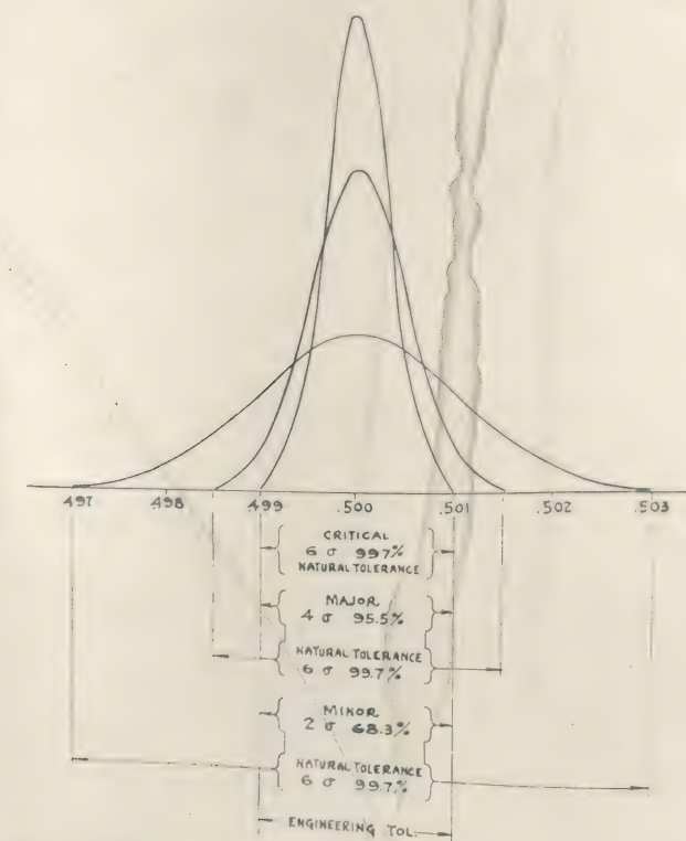
FIG. 1 RELATIONSHIP BETWEEN ENGINEERING AND NATURAL TOLERANCES FOR CRITICAL, AND MAJOR AND MINOR DEFECTS
