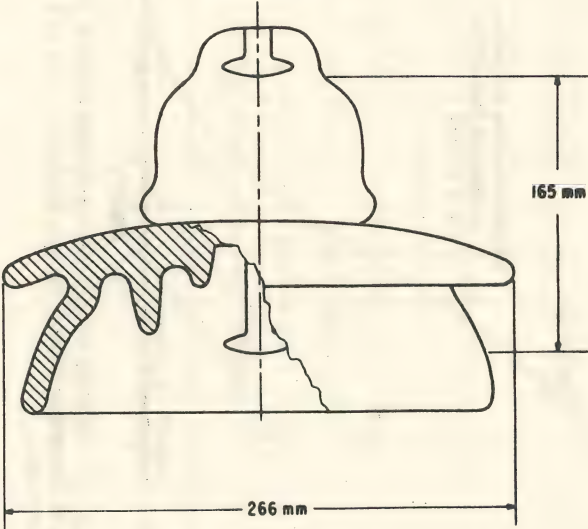
Fig. 3. Test Insulators.
