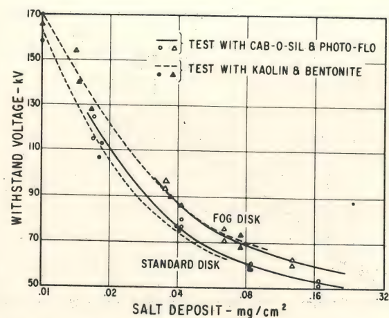
Fig. 6. Comparisons with Different Slurries. Withstand Voltages Versus the Total Salt Deposit Density.
