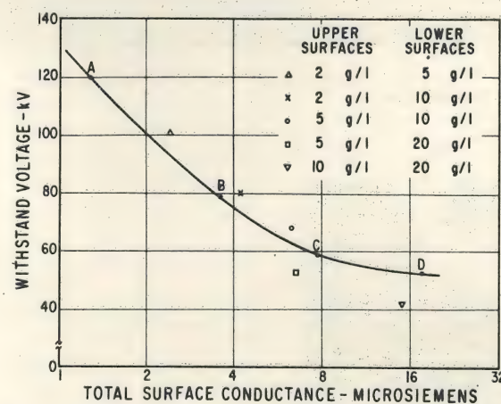
Fig. 10. Non-uniform Distribution of the Contaminant in the Insulators. Withstand Voltages Versus Total Surface Conductance. The Letters A, B, C, D Represent the Points Obtained for Uniform Slurry Coatings of 2, 5, 10 and 20 g/l Salt Respectively.
