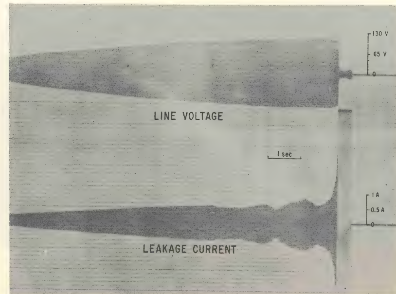
Fig. 16. Applied Voltage and Leakage Current Record: Test with Flashover.
