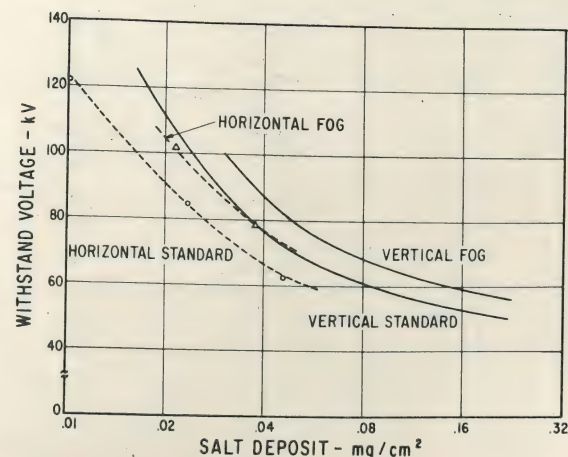
Fig. 13. Vertical and Horizontal Strings. Withstand Voltages Versus Total Salt Deposit Density.
