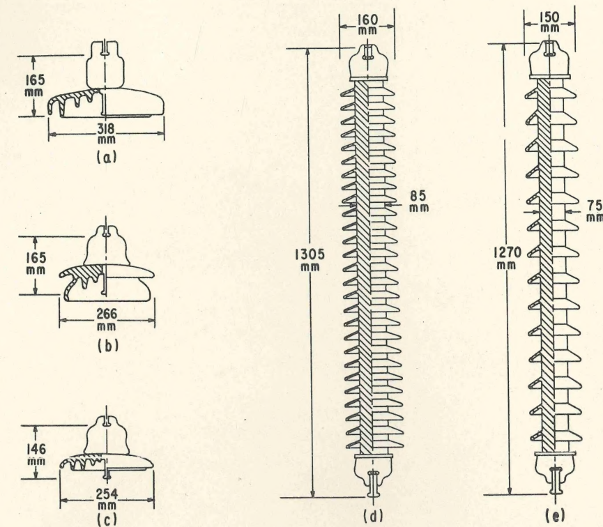
Fig. 1. Tested Insulators.
