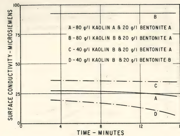
Fig. 2. Influence of Kaolin and Bentonite Types on the Surface Conductivity. Slurries with 5 g/l of Salt.
