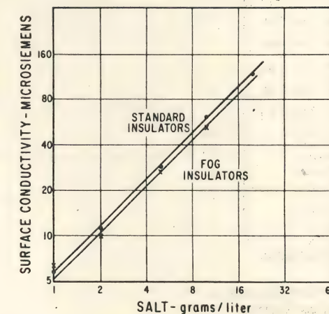
Fig. 4. Slurries with Kaolin and Bentonite. Initial Surface Conductivity Versus the Salt in the Mixture.
