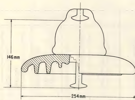
Fig. 1. Tested Insulators.
