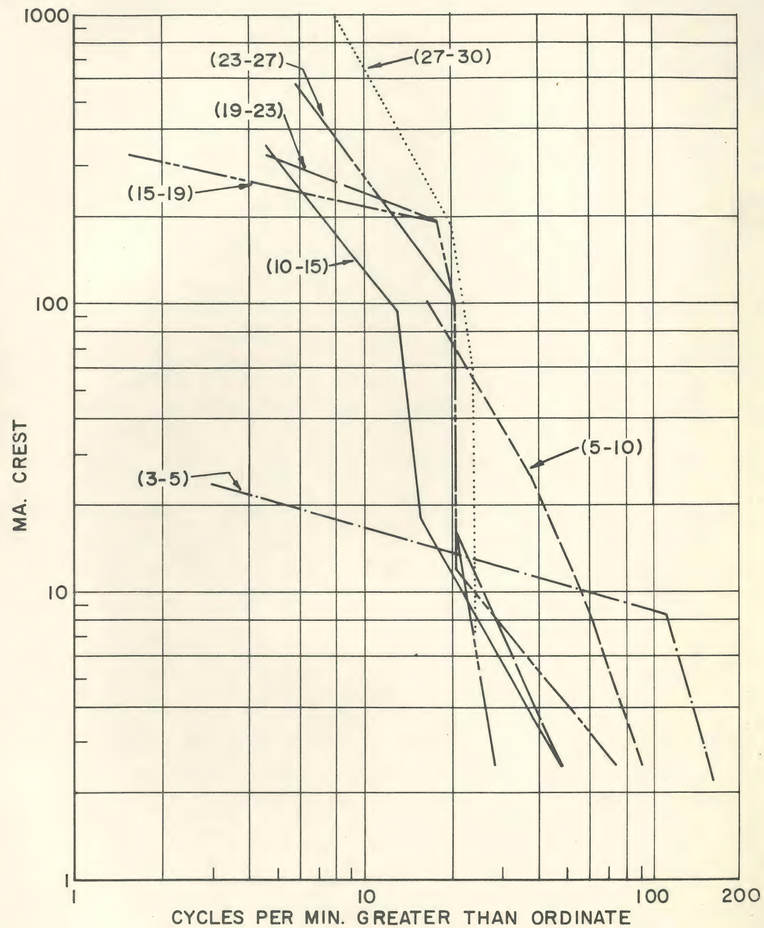
Figure 7. Surge analysis - 15 vertical insulators with 0.2% salt contamination. Curve designations are time period in minutes, measured from start of fog.
