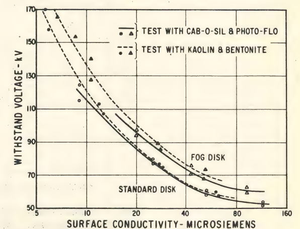
Fig. 5. Comparisons with Different Slurries. Withstand Voltages Versus the Initial Surface Conductivity.
