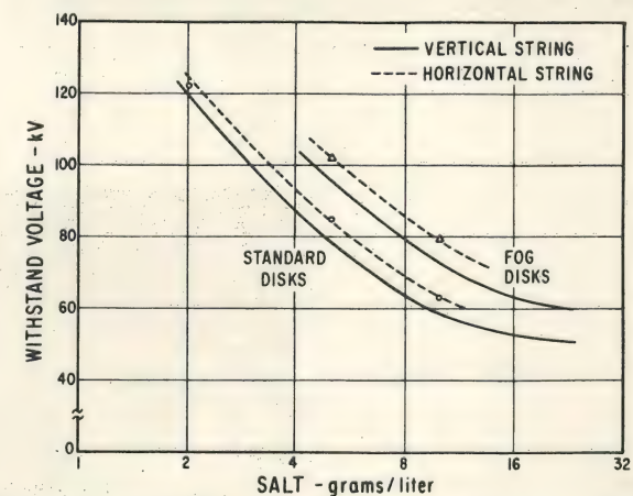
Fig. 11. Vertical and Horizontal Strings. Withstand Voltages Versus Salt in the Mixture.
