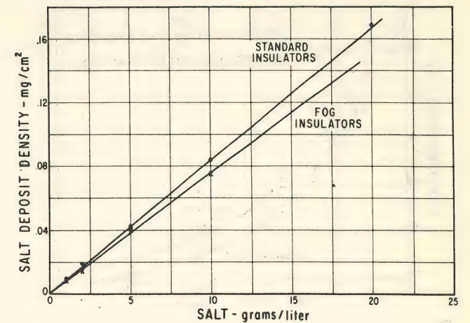
Fig. 3. Slurries with Kaolin and Bentonite. Total Salt Deposit Density Versus the Salt in the Mixture.
