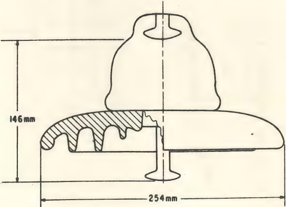
Fig. 3. Test Insulators.
