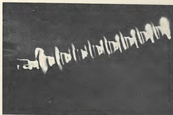
Fig. 14. Horizontal Standard Unit String During a Withstand Test.
