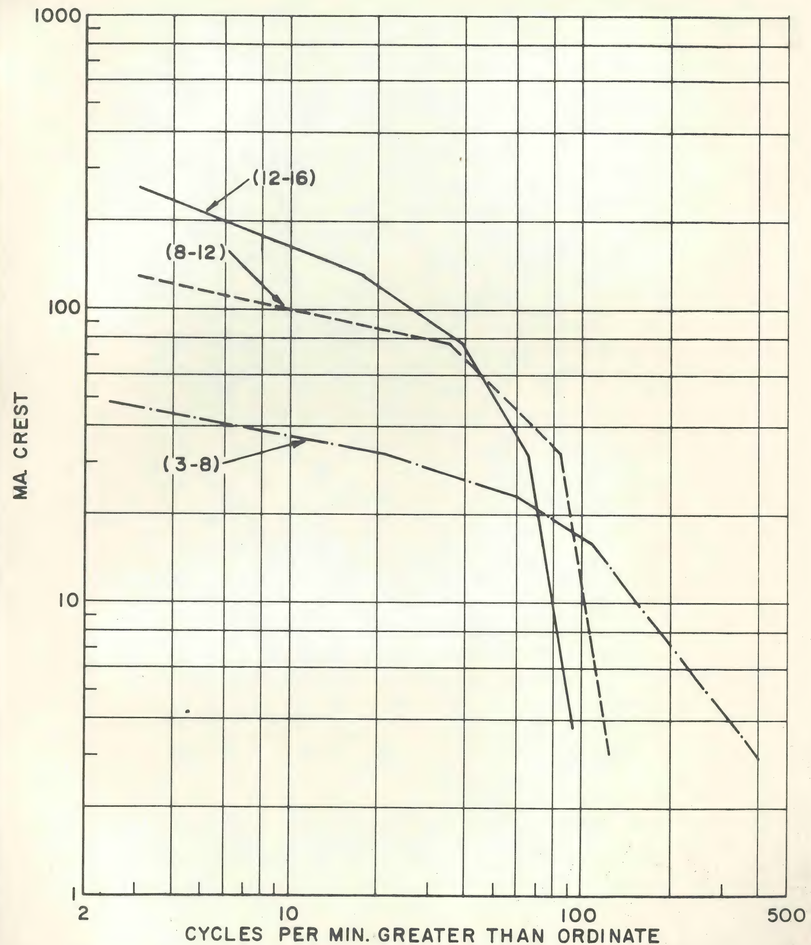
Figure 9. Surge analysis - 15 vertical insulators with 0.8% salt contamination. Curve designations are time period in minutes, measured from start of fog.
