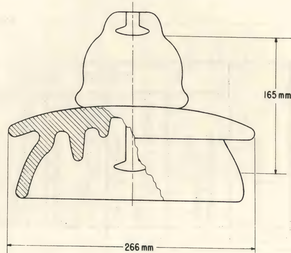
Fig. 1. Tested Insulators.
