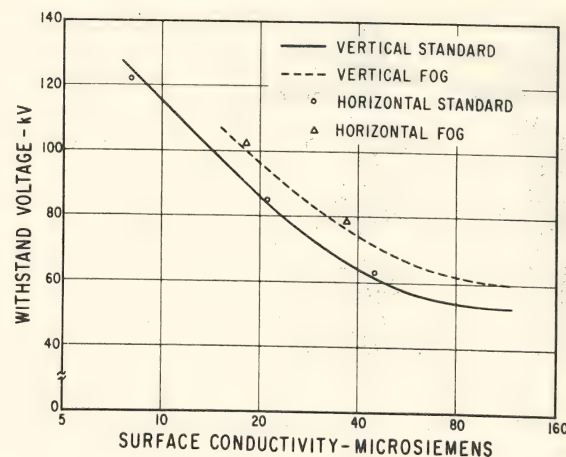
Fig. 12. Vertical and Horizontal Strings. Withstand Voltages Versus Surface Conductivity.
