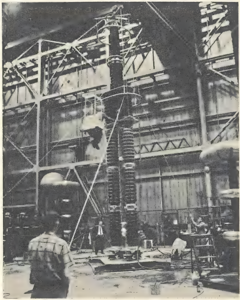
Fig. 2. Flow-coating Method Being Applied to a Lightning Arrester.
