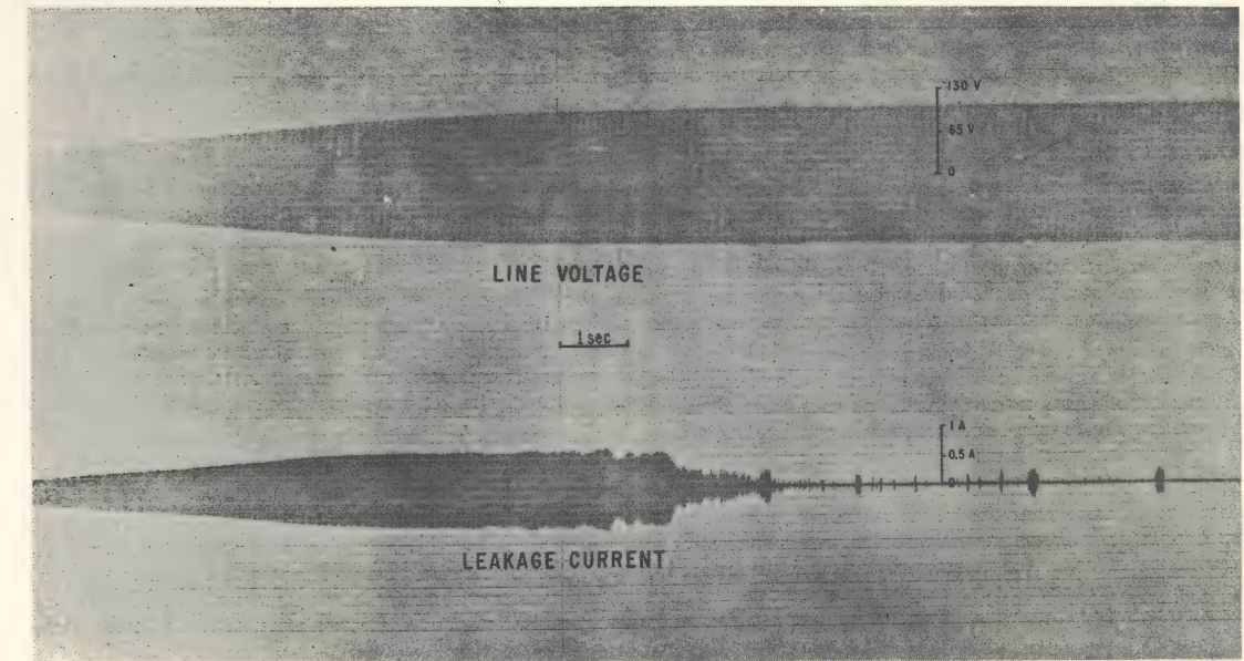
Fig. 15. Applied Voltage and Leakage Current Record: Test with Withstand.
