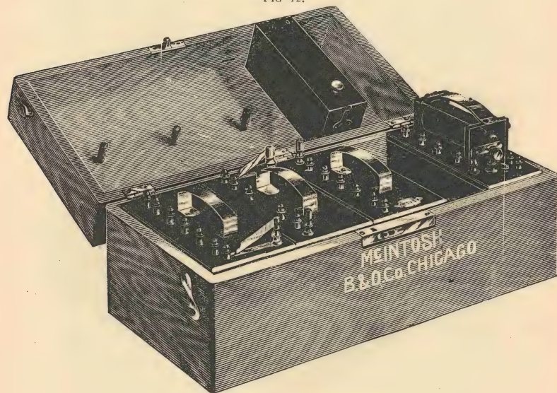
18-CELL COMBINED PORTABLE BATTERY.
