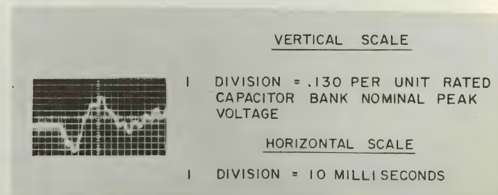
Fig. 11. Transient voltage drop across Cholla-Pinnacle Peak capacitor bank during energization of Cholla to Pinnacle Peak line with Cholla 345 Kv breaker (CB5, Fig. 6).
