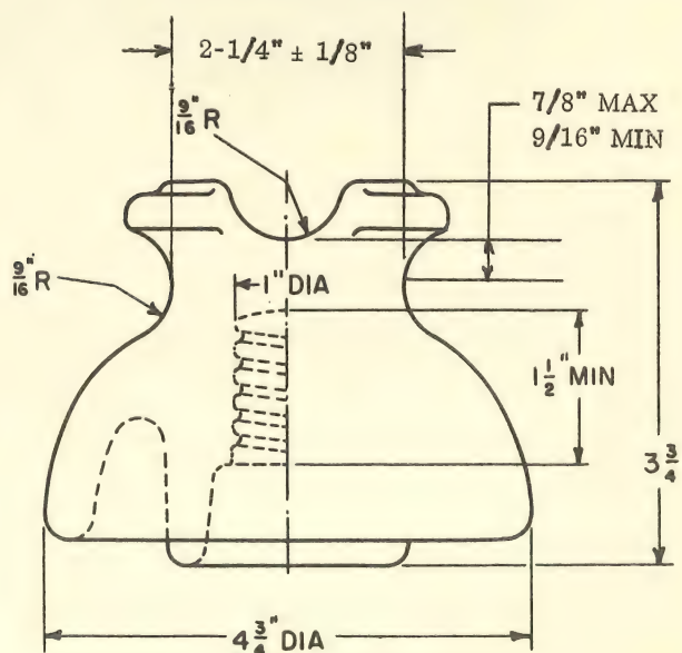
Fig. 3 Pin Insulator, Class 55-3
