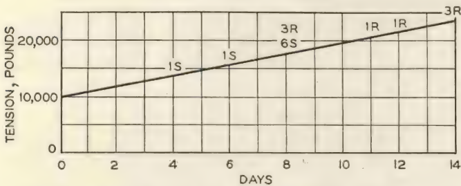
Fig. 8. Results of duration load test on porcelain insulators, showing effect of glazing treatment
