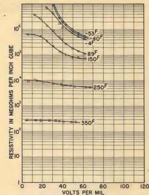
Figure 3. Voltage gradient vs resistivity, wet process electrical porcelain, thickness 0.8 inch, electrode area 30 square inches.
