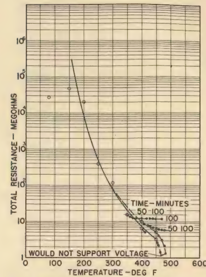
Figure 7. Temperature vs resistance of 23 kv NEMA Standard outdoor switch and bus insulator, total voltage applied 14 kv d-c.
