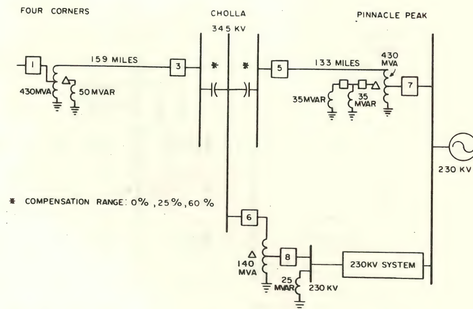
Fig. 5. One line diagram of model system representation without Four Corners generation.
