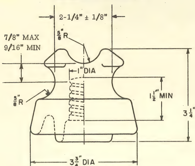
Fig. 2 Pin Insulator, Class 55-2
