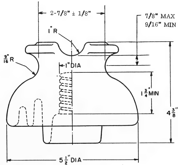
Fig. 4 Pin Insulator, Class 55-4
