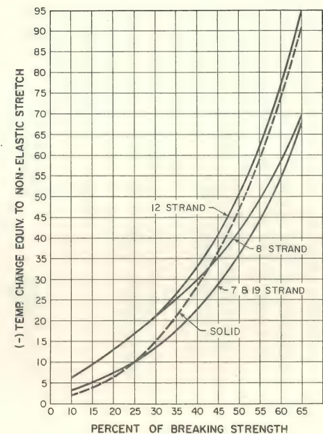
Fig. 2. Non-elastic Stretch Chart.
