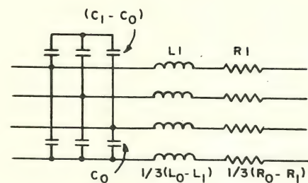
Fig. 4. Typical 10 mile model line section used in Transient Network Analyzer study. Subscripts 0 and 1 denote zero and positive sequence quantities respectively.
