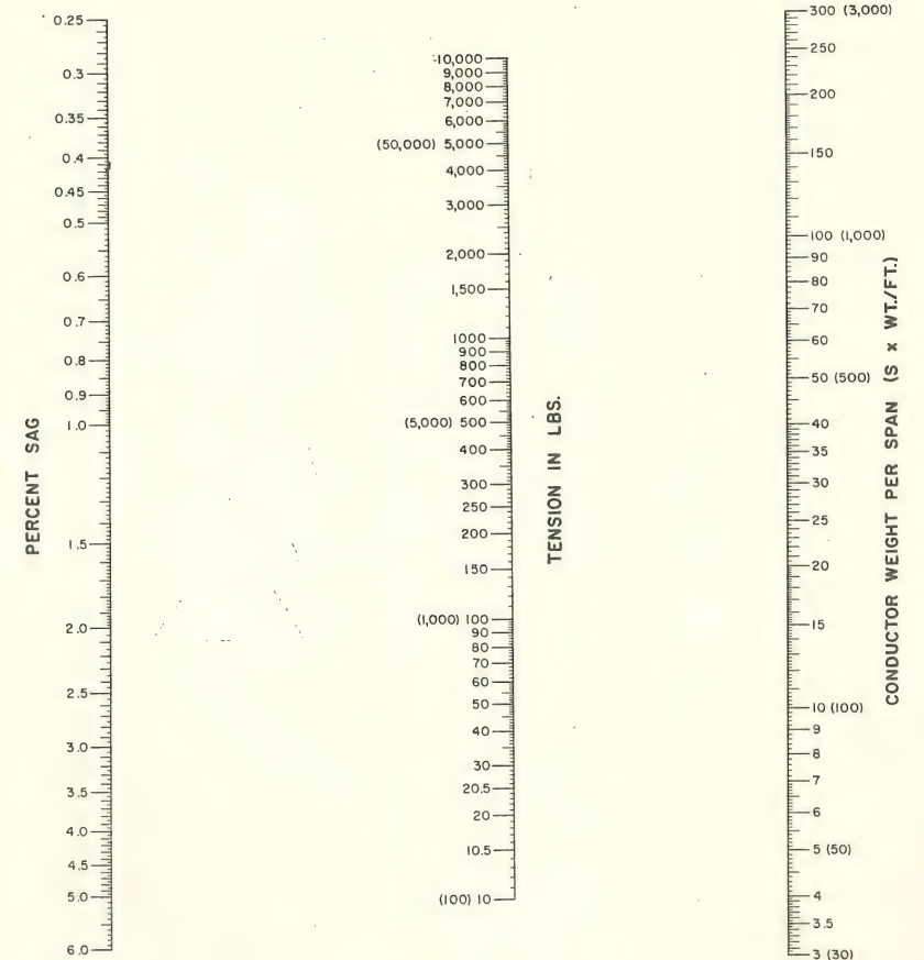
Fig. 3. Sag-Tension Chart
