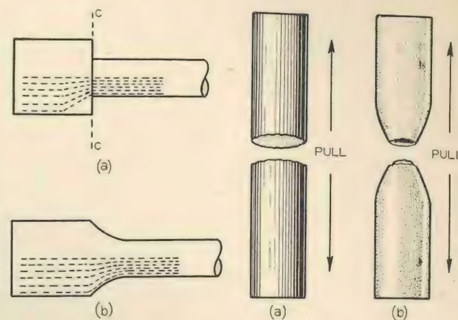
Fig. 1. Effect of shape on nonductile specimens in tension
