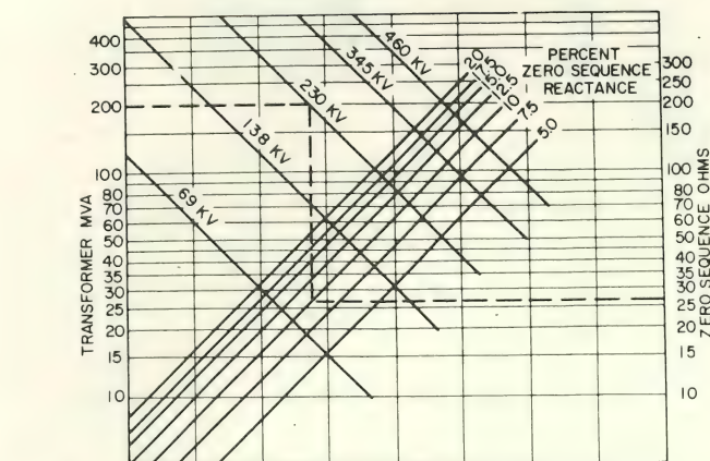
Fig. 6. Zero sequence ohms as function of transformer MVA, voltage rating, and percent zero sequence reactance. Example shown for a 200 MVA, 230 kv transformer having a 10 percent zero sequence reactance.
