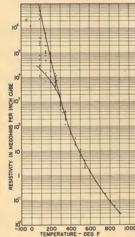
Figure 4. Composite curve. Temperature vs re- sistivity wet process electrical porcelain.
