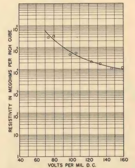
Figure 13. Voltage gradient vs resistivity, wet process Steatite, temperature 84 F, specimen thickness 0.188 inch and 0.203 inch.
