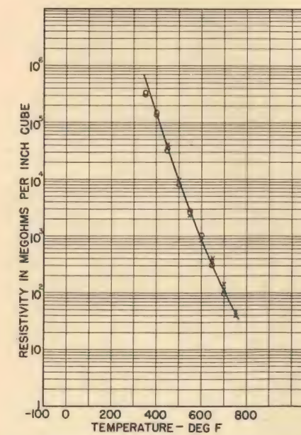
Figure 12. Temperature vs resistivity, wet process steatite, voltage gradient 20 and 40 volts per mil, specimen thickness 0.188 inch and 0.203 inch.
