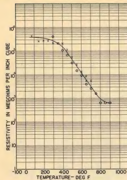
Figure 14. Temperature vs resistivity, zircon, 40 volts per mil, 2 square inch electrode 0.489 inch thick and 1 square inch electrode 0.196 inch thick.
