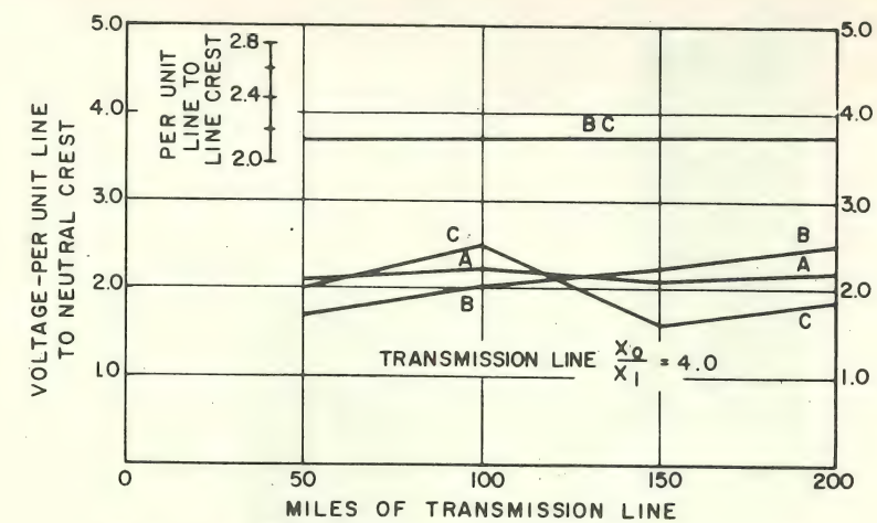
Fig. 7. Phase-to-neutral voltages giving maximum phase-to-phase voltage on open-ended line.
