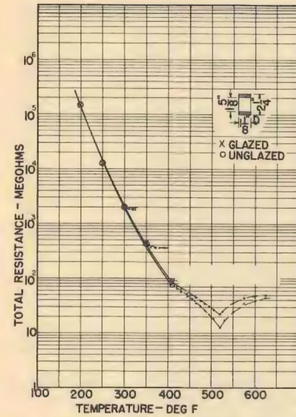
Figure 6. Temperature vs resistance, comparison of glazed and unglazed wet process electrical porcelain, total voltage applied 5000 volts d-c.
