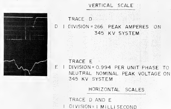
Fig. 8B. Energization transient of Fig. 8A as modified by lightning arrester operation.
