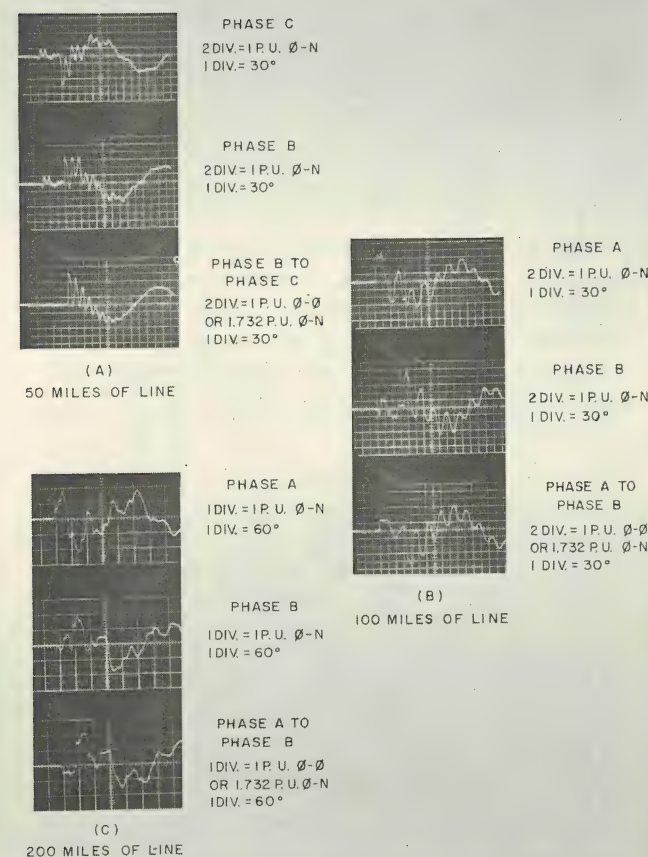
Fig. 8. Typical oscillograms from TNA study. Voltage at receiving end of open-ended line is shown for 50 miles, 100 miles and 200 miles, respectively. X_0/X_1 of line = 4.
