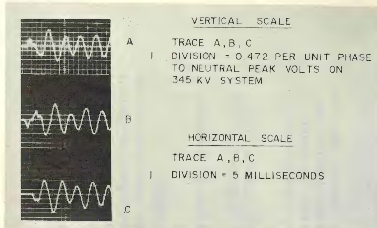
Fig. 10. Recovery voltage across Cholla 345 Kv breaker contacts, (CB5, Fig. 6) following restrike upon de-energization of Cholla-Pinnacle Peak line.
