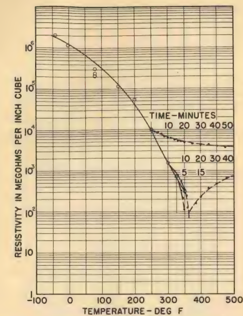
Figure 2. Temperature vs resistivity, wet pro- cess electrical porcelain, voltage gradient 40 volts per mil d-c, thickness 0.8 inch, electrode area 30 square inches.
