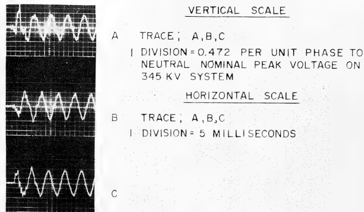
Fig. 8A. Transient voltage at Four Corners high side (unmodified by lightning arrester) during energization of Cholla to Four Corners line with Cholla 345 Kv breaker. (CB3, Fig. 5). No series capacitors; two 35 MVAR reactors on Pinnacle Peak tertiary; 1.10 P.U. preswitching voltage at Cholla 345 Kv bus.
