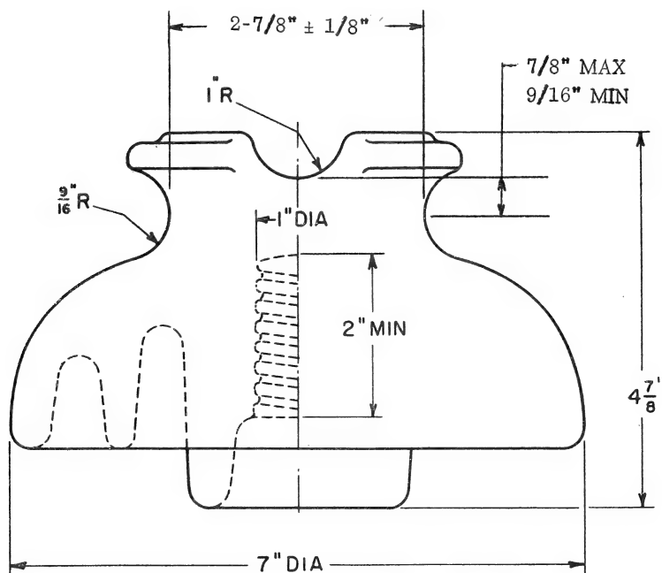
Fig. 5 Pin Insulator, Class 55-5
