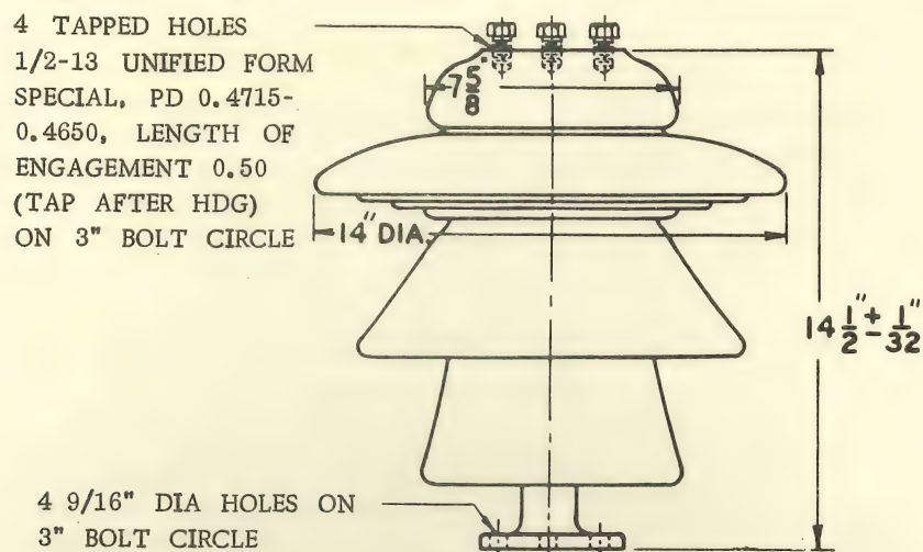
Fig. 16 Apparatus Insulator, Cap and Pin Type
