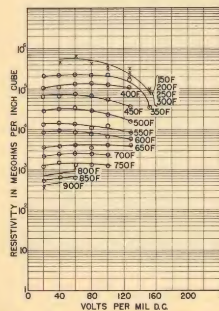
Figure 15. Voltage gradient vs resistivity, zircon, 1 square inch electrode, specimen thickness 0.196 inch.
