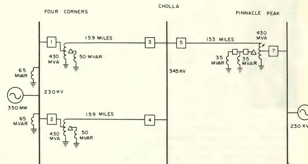
Fig. 7. One line diagram of model system representation without Cholla 230 Kv tie.
