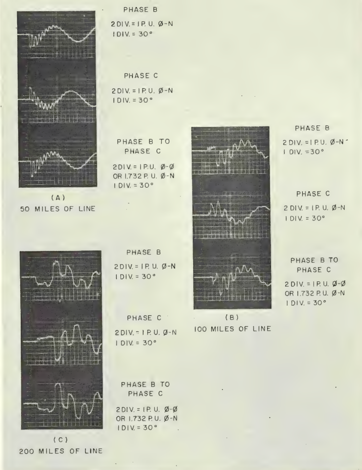
Fig. 5. Typical oscillograms from TNA study. Voltage at receiving end of transformer terminated line is shown for 50 miles, 100 miles and 200 miles, respectively. X_0 of transformer = 26.4 ohms. X_0/X_1 of line = 4.
