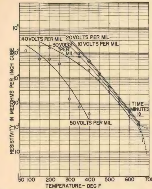
Figure 10. Temperature vs resistivity, lead glass specimen thickness 0.50 inch.
