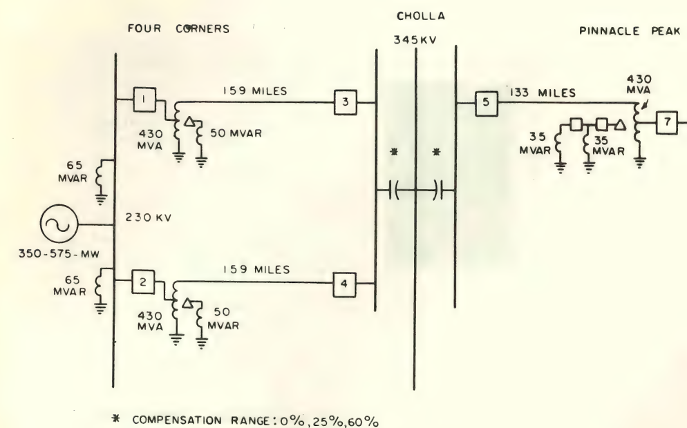
Fig. 6. One line diagram of model system representation without Pinnacle Peak and Cholla 230 kv ties.
