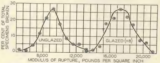
Fig. 11. Distribution curves for failure of unglazed and glazed specimens
