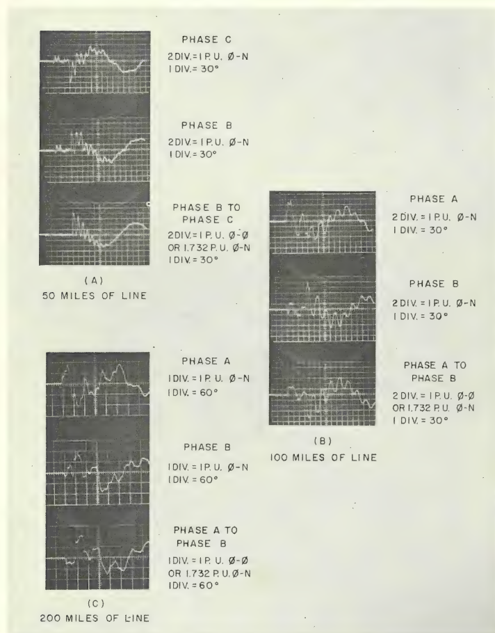
Fig. 8. Typical oscillograms from TNA study. Voltage at receiving end of open-ended line is shown for 50 miles, 100 miles and 200 miles, respectively. X_0/X_1 of line = 4.
