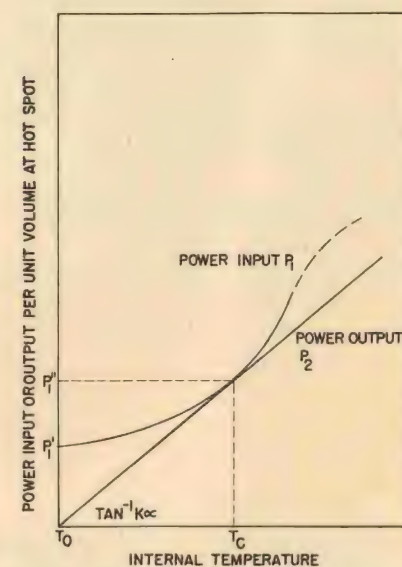
Figure 17. Power input and power output conditions leading to ultimate breakdown.
