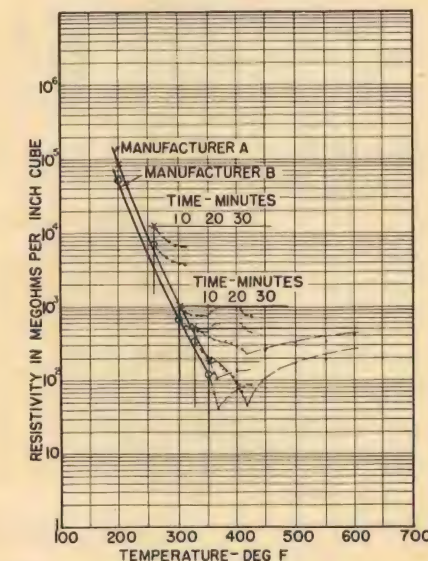
Figure 5. Temperature vs resistivity, compari- son of two manufacturers of wet process electri- cal porcelain, voltage gradient 20 volts per mil, specimen thickness 0.55 inch.
