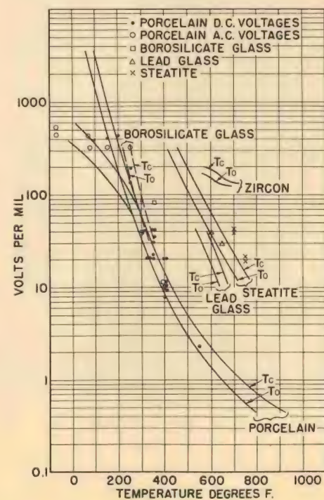
Figure 18. Temperature vs voltage gradient for breakdown.
