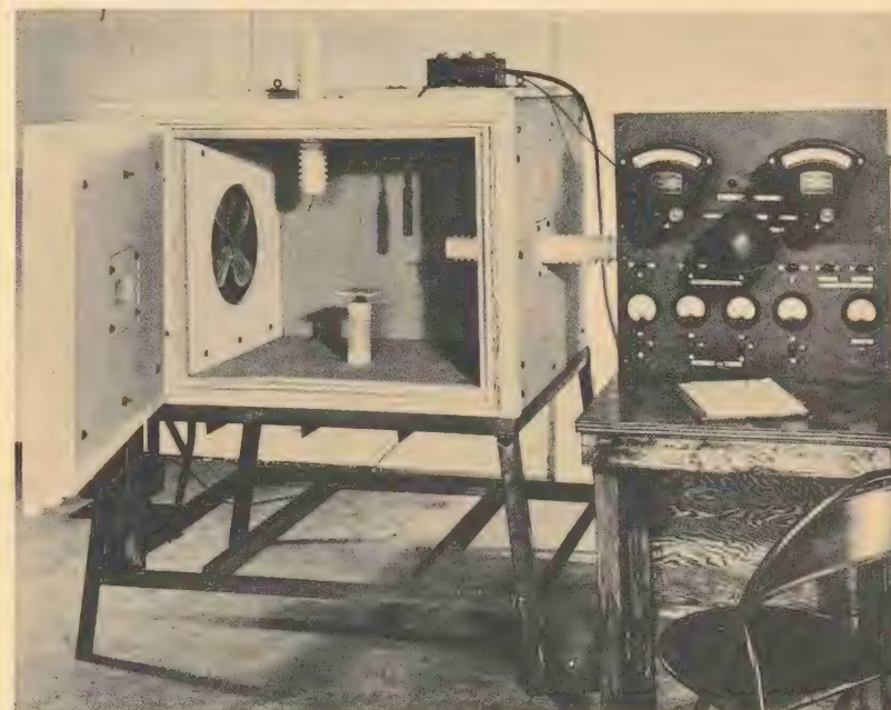
Figure 1. Test chamber and operating panel with specimen mounted in position.
