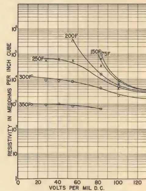
Figure 9. Voltage gradient vs resistivity, boro-silicate glass, thickness 0.36 inch.
