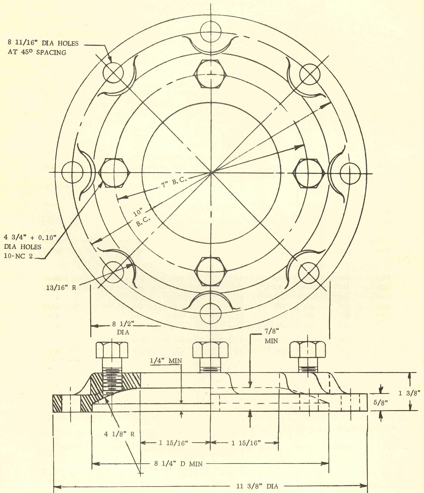
Fig. 20-1 TRANSITION PLATE (UPRIGHT) TR NUMBER 151
