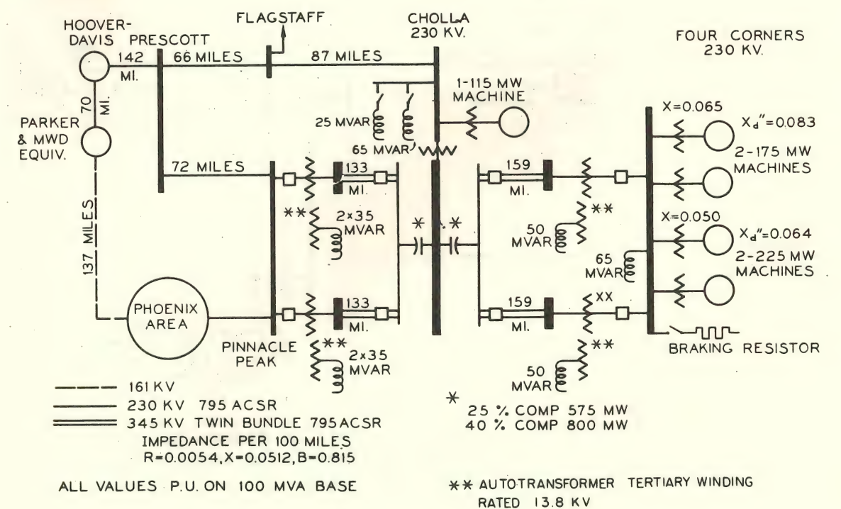
Fig. 3. 345 Kv transmission facilities for 575 MW and 800 MW Four Corners generation.
