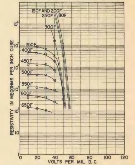
Figure 11. Voltage gradient vs resistivity, lead glass, specimen thickness 0.50 inch.
