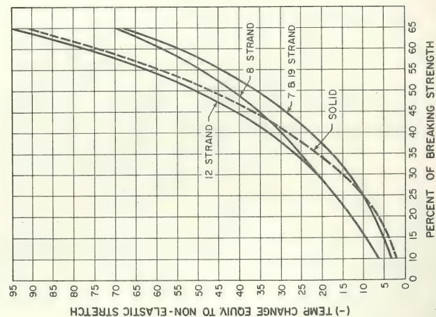
Fig. 2. Non-elastic Stretch Chart.
