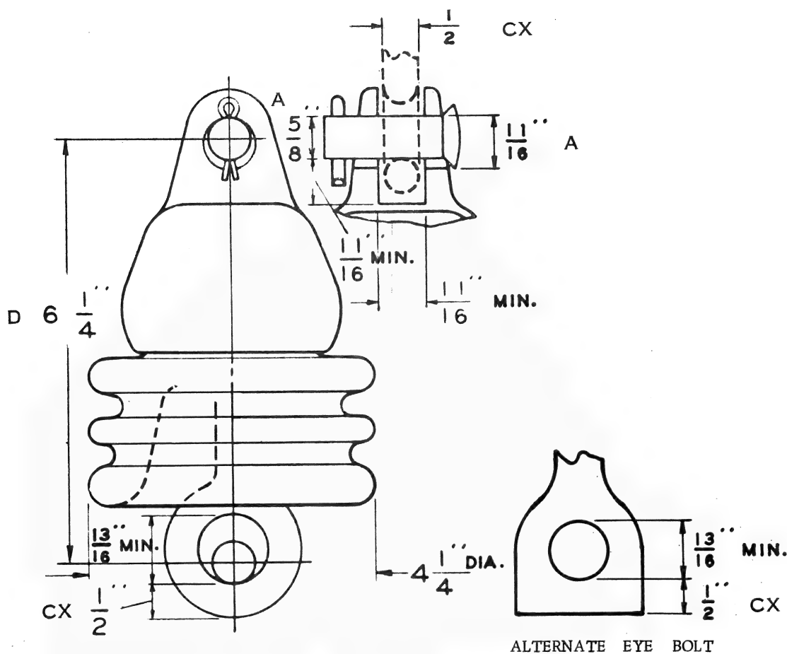
Fig. 7b Dead-end Suspension Insulator, Class 52-9
