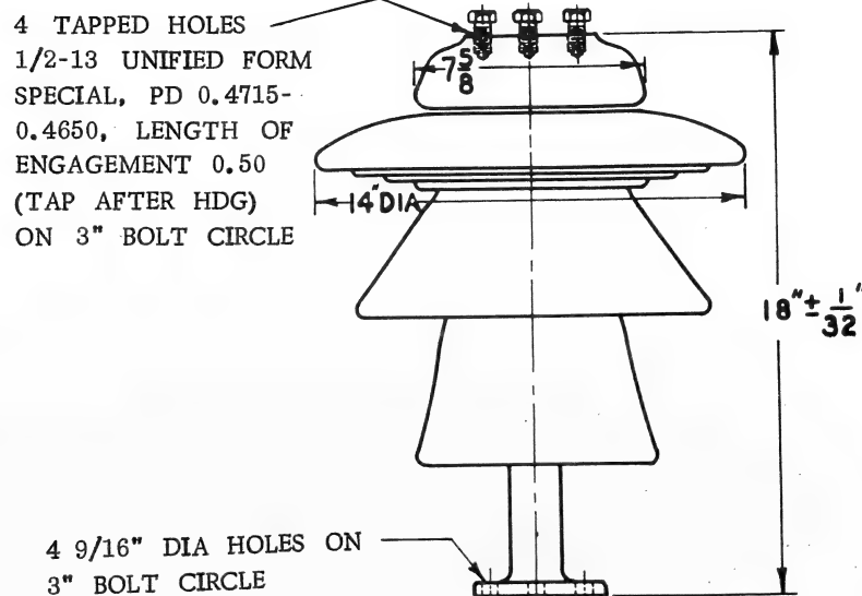
Fig. 17 Apparatus Insulator, Cap and Pin Type
