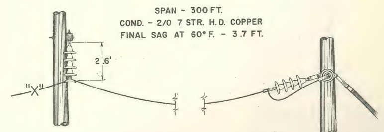
Fig. 4. Line Configuration for Broken Conductor Problem.
