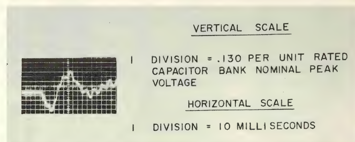
Fig. 11. Transient voltage drop across Cholla-Pinnacle Peak capacitor bank during energization of Cholla to Pinnacle Peak line with Cholla 345 Kv breaker (CB5, Fig. 6).
