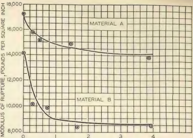
Fig. 13. Results obtained on time load tests; abscissa is the reciprocal of the rate of loading in pounds per square inch per second in modulus of rupture
