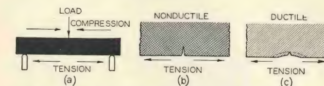
Fig. 3. Behavior of cracks in nonductile and ductile materials in tension
