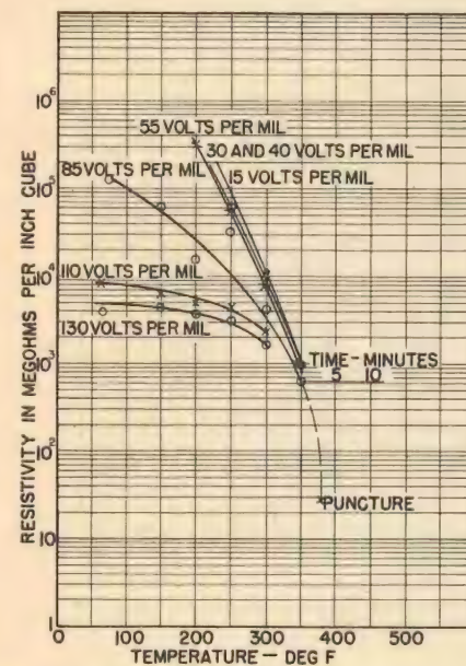
Figure 8. Temperature vs resistivity, boro-silicate glass, thickness 0.36 inch.
