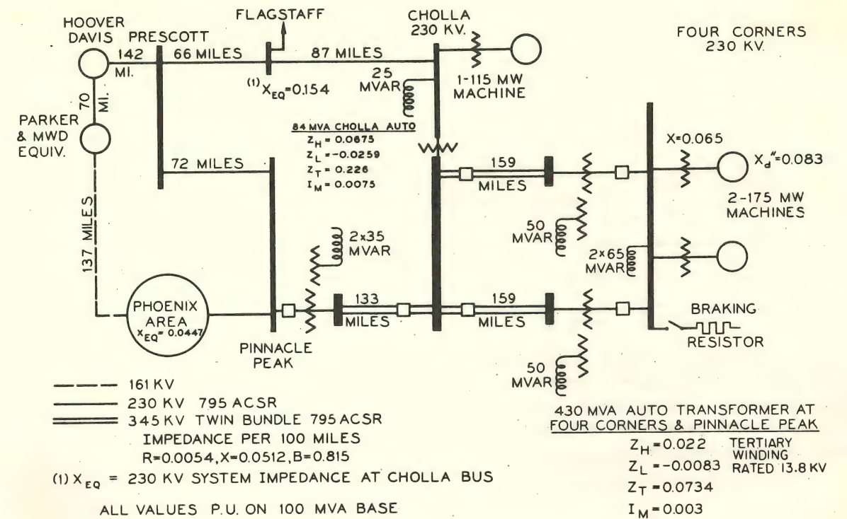
Fig. 2. 1963, 345 Kv transmission facilities for 350 MW Four Corners generation.
