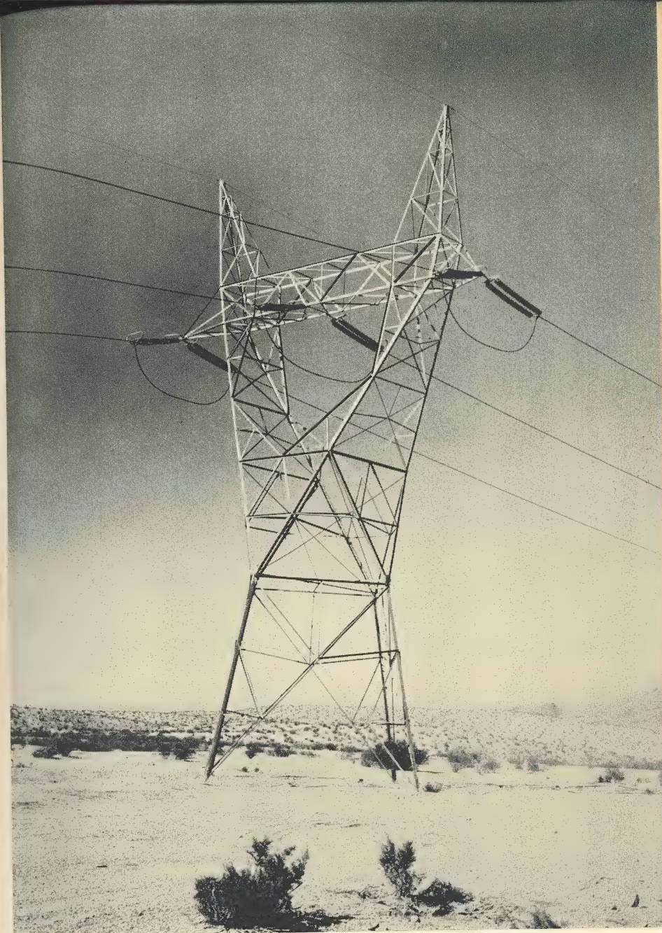
A strain-tower of the Hoover Dam-Los Angeles 287-kilovolt line of the City of Los Angeles. Note two overhead ground wires at top of structure. Courtesy Bureau of Power and Light, City of Los Angeles.
