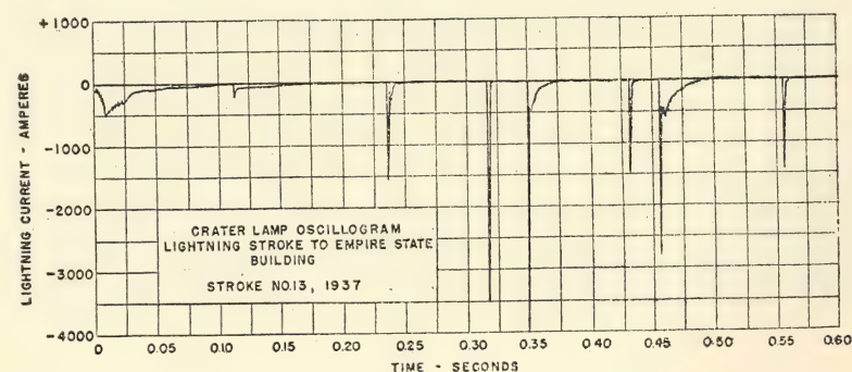
(Top) Still- and moving-lens photographs of stroke No. 13. Oscillogram of same stroke is shown. Notice close correlation between current magnitude and photographic density. Record taken in 1937.
