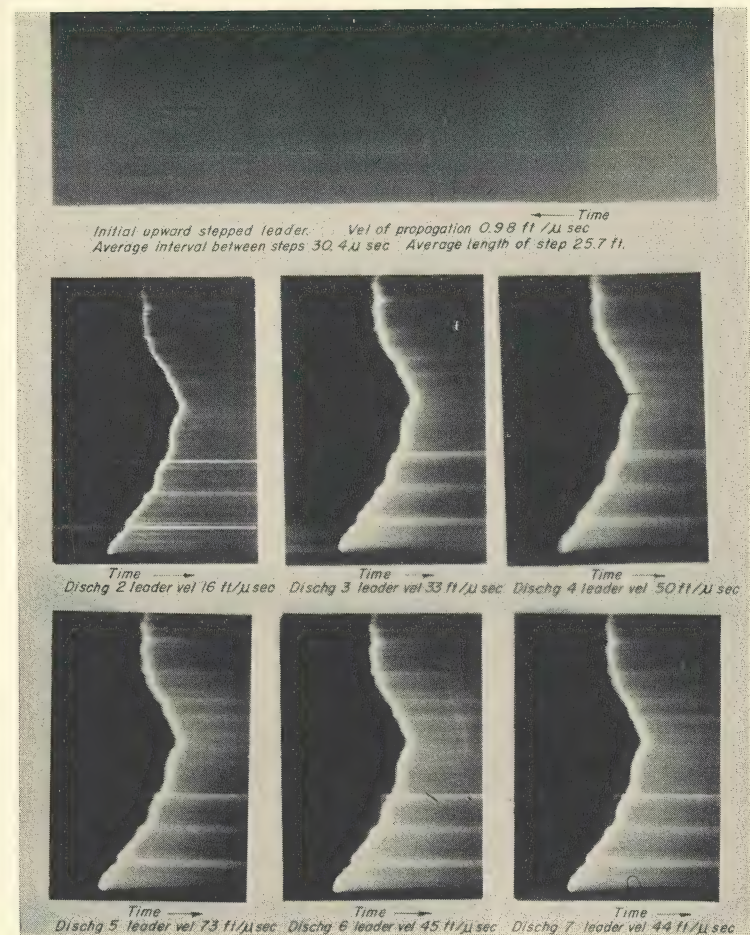
Multiple stroke to Empire State tower, consisting of a long-continuing low-current discharge preceded by initial upward stepped leader and followed by six non-continuing discharges all having downward continuous leaders. These are high-speed Boys camera photographs of stroke No. 16, taken August 11, 1937. Oscillogram of this stroke shown below.
