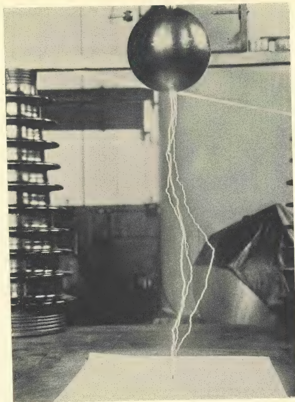
Laboratory lightning striking a miniature rod to determine the protected area around rod. Tests by F. W. Peek.
