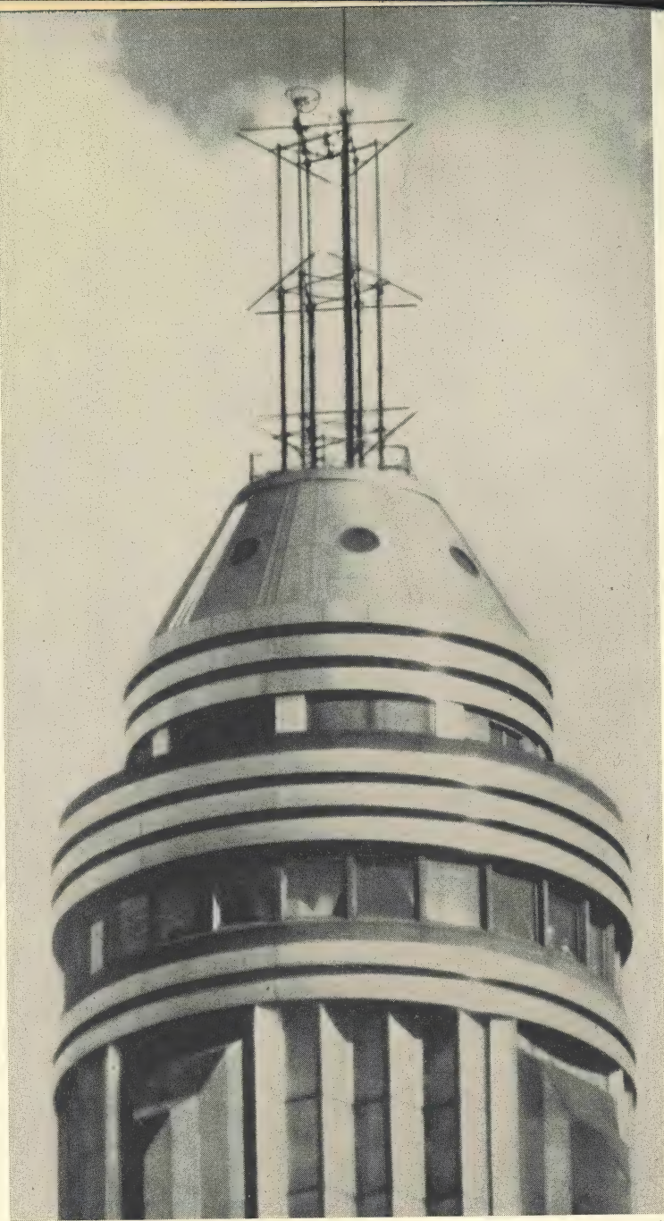
The antenna system atop the Empire State Building, completed in this form in July, 1936. Oscillographs connected to highest antenna.
