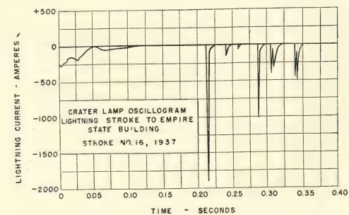
Oscillogram of stroke No. 16, showing steady current-flow in beginning, followed by six current-peaks of widely different values. Oscillograph is delayed slightly compared to photograph of this stroke.
