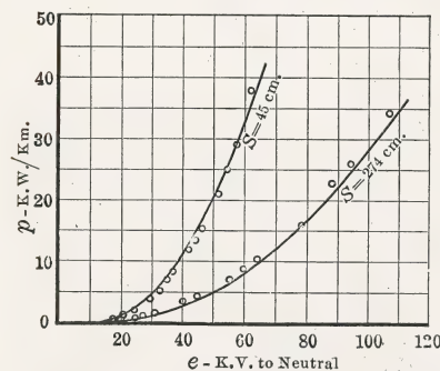
FIG. 152.—Comparison of calculated and measured corona loss for small conductors at small and large spacings.
