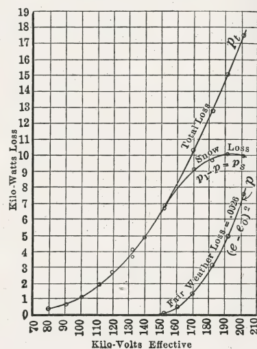
FIG. 162.—Corona loss during snow storm.
