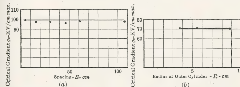
FIG. 29(a).—Variation of visual critical gradient with spacing. (Parallel wires. Diameter constant = 0.034 cm.) FIG. 29(b).—Variation of visual critical gradient with radius of outer cylinder. (Concentric cylinders. Diameter of inner wire constant = 0.118 cm.)
