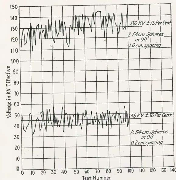
FIG. 178.—Curves showing variation of dielectric strength of oil during one hundred successive tests.
