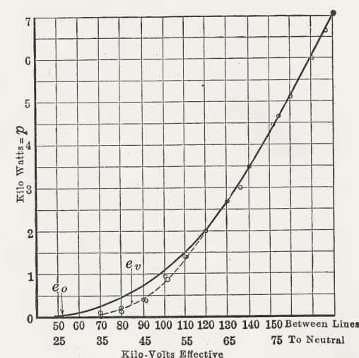
Fig. 142.—Characteristic corona loss curve for small wire. No. 8 copper wire. Diameter, 0.328 cm. Total length, 29,050 cm. Spacing, 0.328 cm. Table XLVI, Line B.
