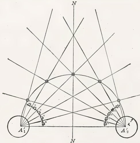
FIG. 259.—Graphical method of drawing lines of force between two cylinders. on N. N. , and passing through the point of intersection of the radial line N. N. , A'_1 , and A'_2 . The lines of force are therefore determined. The centers, etc., might have been calculated from equation (8), page 20. The line of force is also determined graphically by drawing the diagonal line through the intersection of radial lines, as shown in Fig. 259.
