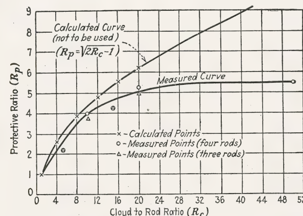
FIG. 215.—Curves showing relation between R_p (ratio of protected radius to rod height, or protective ratio), and R_c (ratio of cloud height to rod height). Calculated curve not to be used. See also Fig. 267, page 397.
