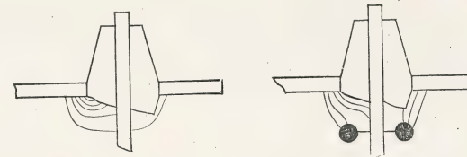
FIG. 241.—Making bushing shown in Fig. 240 operative by flux control after lower part had broken off.
