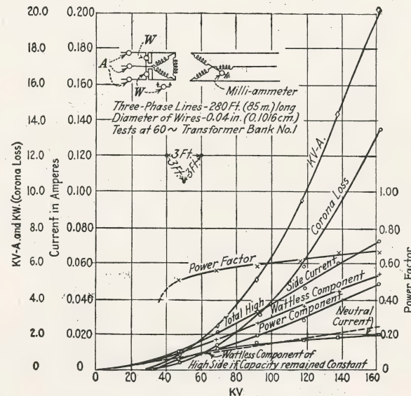
FIG. 176.—Characteristics of a three-phase line with Y grounded neutral transformers, as affected by corona.
