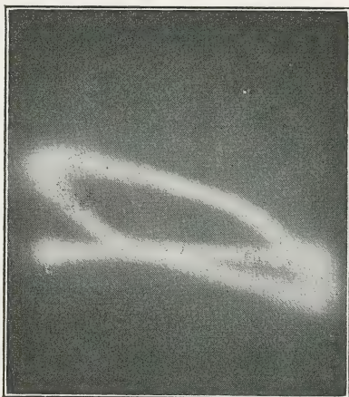
FIG. 172.—Corona loss cyclogram indicating coulomb-voltage relation per cycle
