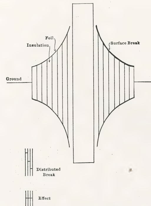
FIG. 237.—Condenser bushing.
