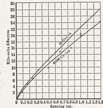
FIG. 115.—Sphere gap spark-over voltages at 60 cycles and 40,000 cycles.
