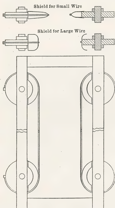
FIG. 28.—Wire support for visual corona tests.
