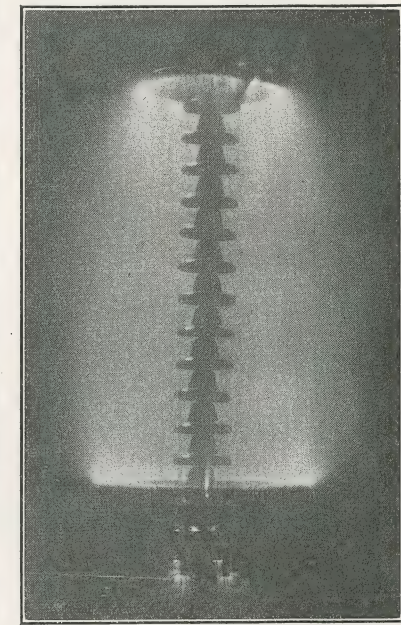
FIG. 250.—Dissipation of lightning energy by corona on insulator shields.
