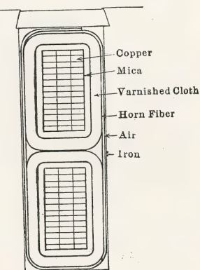
FIG. 233.—Corona on generator coils.
