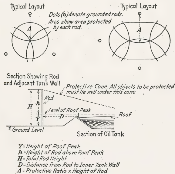
FIG. 216.—Method of protecting oil tanks from direct lightning strokes.
