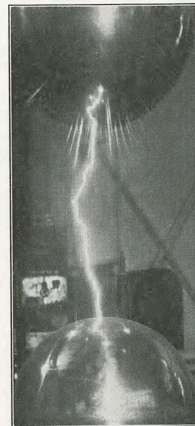
FIG. 121.—Impulse sparkover between 100 cm. spheres.
