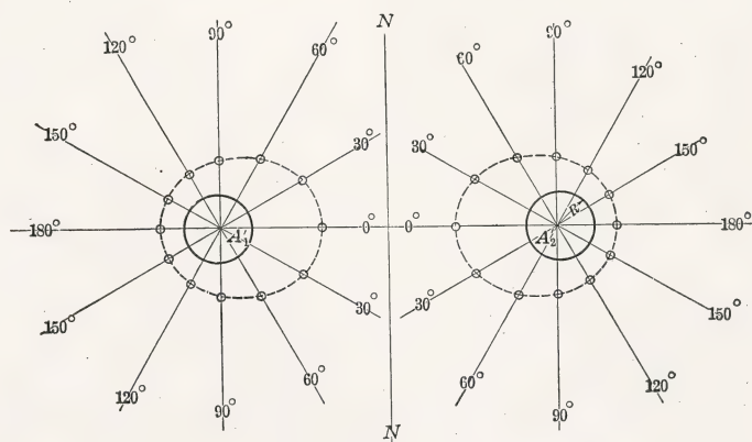
FIG. 260.—Method of plotting equigradient curves.
