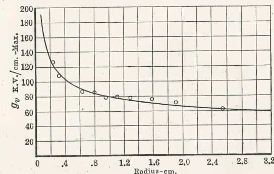
FIG. 180(a).—Strength of oil at 60 ~. (Concentric cylinders— g_v at surface of inner cylinder.)
