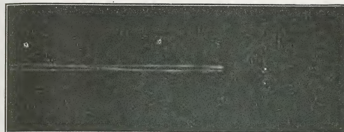
(3) With stroboscope -. Diameter, 0.325 cm. Spacing, 120 cm. Volts, 180,000.
