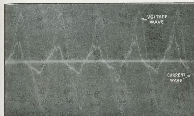
FIG. 89.—Corona current from needle point at one million volts. (Carroll & Cozzens, Stanford Univ. )
