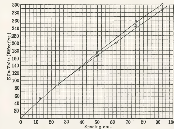
FIG. 111.—Spark-over voltages between points. o, dry; Δ, wet; x, rain. 0.25' per minute. 60° points on 1.25 cm. rods.
