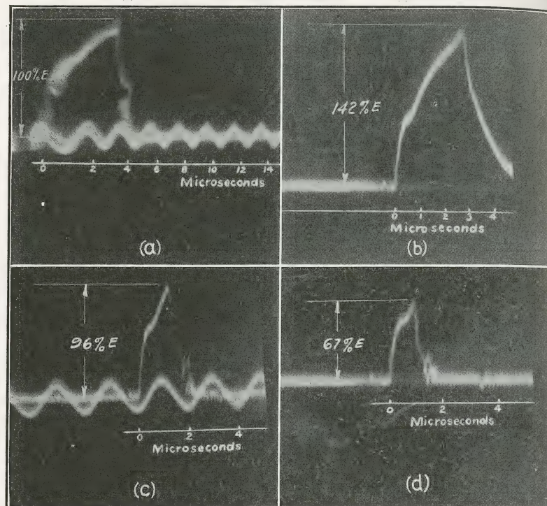
FIG. 207.—Cathode ray oscillograms of waves on transmission lines: (a) Initial wave at sending end; (b) initial wave reflected to double voltage at open far end, after attenuation to 71 per cent.; (c) wave at far end chopped by gap set at 96 per cent. of sending voltage; (d) wave at far end chopped by gap set at 67 per cent. of sending voltage.
