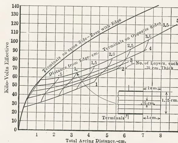
FIG. 194.—Surface arc-over in oil. (Hendricks.)
