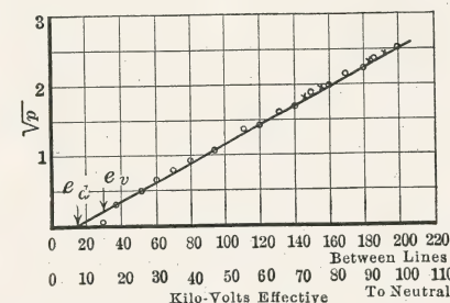
Fig. 144.—Corona loss plotted between \sqrt{p} and e to illustrate the quadratic law. Phosphor-bronze conductor. Diameter, 0.051 cm. Spacing, 366 cm. Total length, 29,050 cm. Temp., -6.5^\circ C. Bar., 77.3 cm. Line B.
