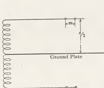
FIG. 55.—Arrangement for two conductors at same potential, and plate.
