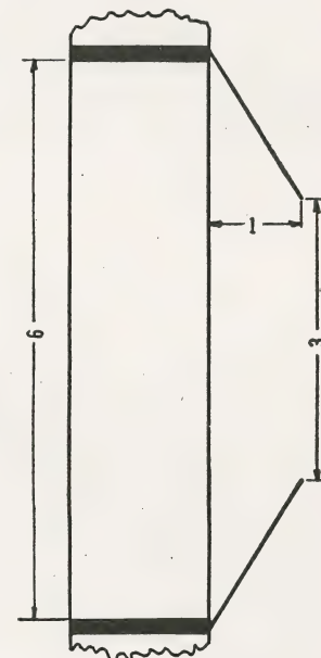
FIG. 265.—Proportions for wood-pole protective gap. (Note discussion in text below.)
