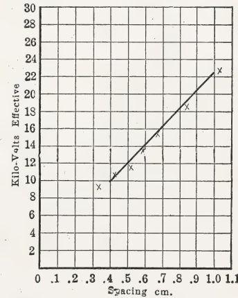
FIG. 114.—Sphere-gap spark-over voltages at 60 cycles and 1000 cycles. 12.5 cm. spheres.
