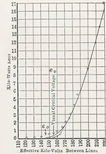
FIG. 220.—Loss near the critical voltage of new and old cables. (Data Fig. 219. Line calculated. x, new cable. o, weathered cable.)
