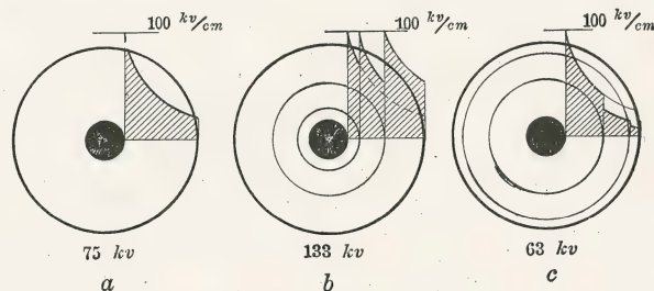
FIG. 235.—Graded cable.
