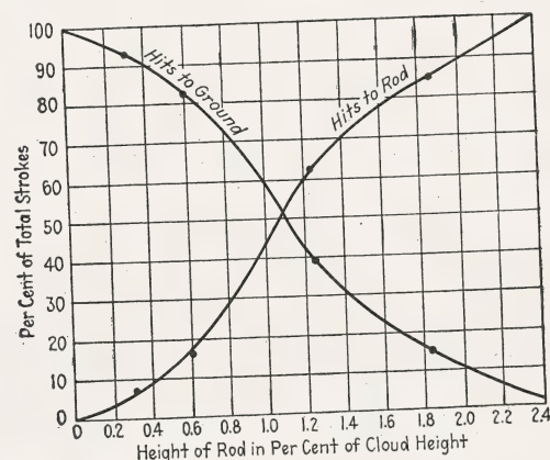
FIG. 214.—Division of laboratory lightning hits between rod and ground with different rod heights.
