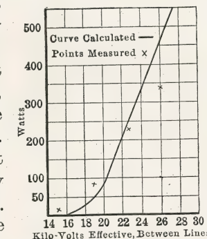
FIG. 173.—Corona loss at high frequency.
