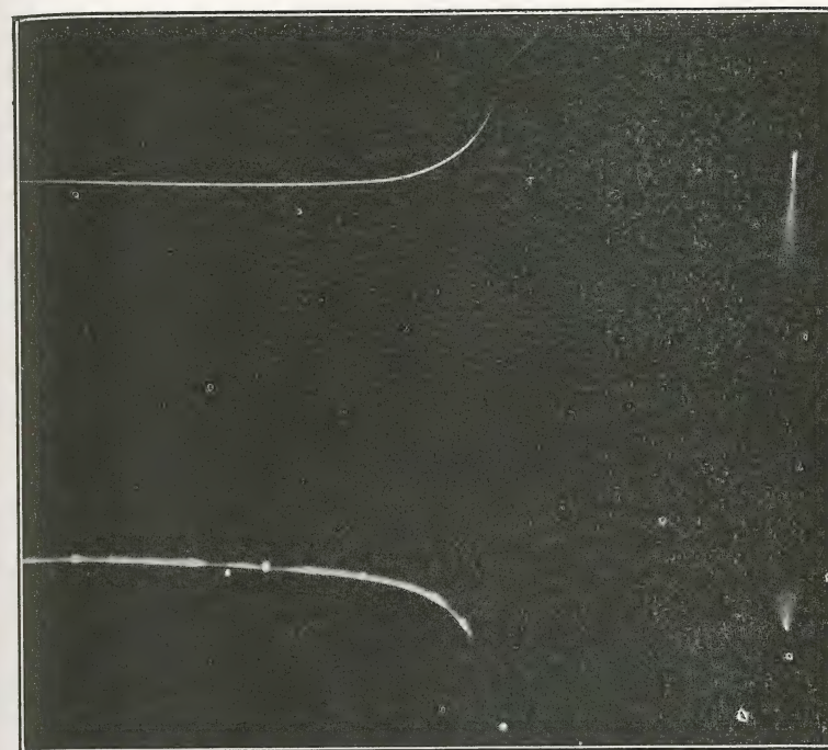
Fig. 75.—Comparison of — and + A. C. corona on wire and points. (Same as Fig. 75 with stroboscope.)
