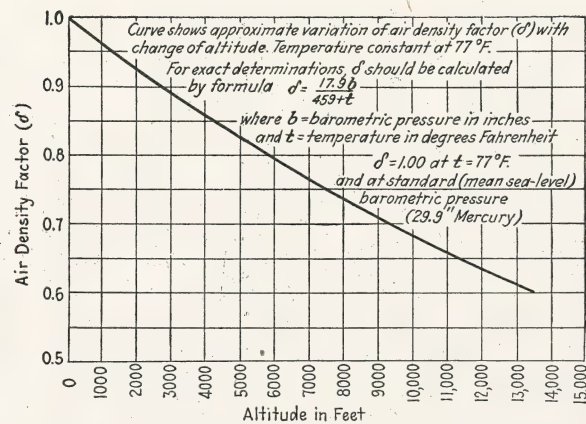
Fig. 230.—Air density factor ( \delta ) as affected by altitude.
