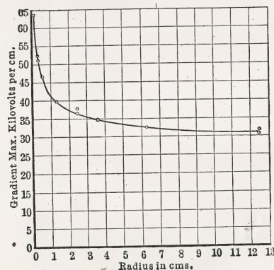
FIG. 46.—Variation of the apparant strength of air with sphere radius. Points measured gradient from constant part of curve. Drawn curve, calculated from equation (27).
