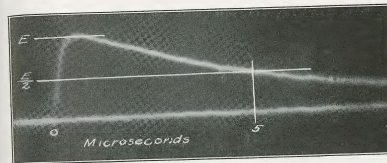
FIG. 124.—Cathode-ray oscillogram of typical impulse wave of lightning generator.
