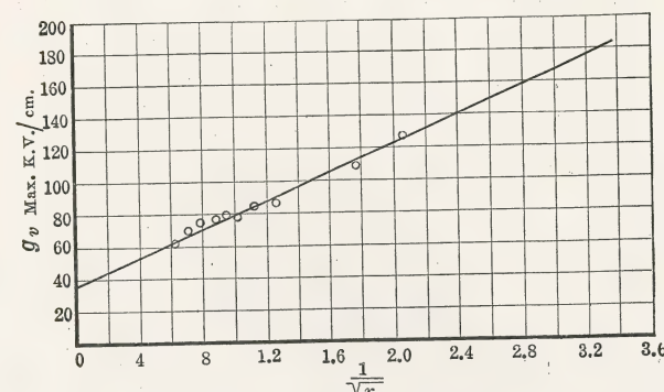
FIG. 180(b).—Strength of oil at 60 ~. (Method of reducing values given in Fig. 180a to equation.)
