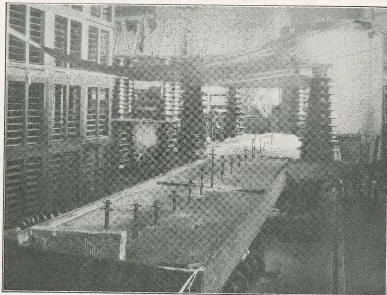
FIG. 212.—Typical laboratory cloud and transmission-line model for studying induced lightning voltages.
