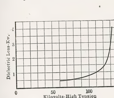
FIG. 193 (a).—Dielectric loss vs. voltage in a 2750 kv-a, 120 kv, 60 ~ transformer.
