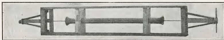
FIG. 32.—Apparatus for determining the visual corona voltage in concentric cylinders.
