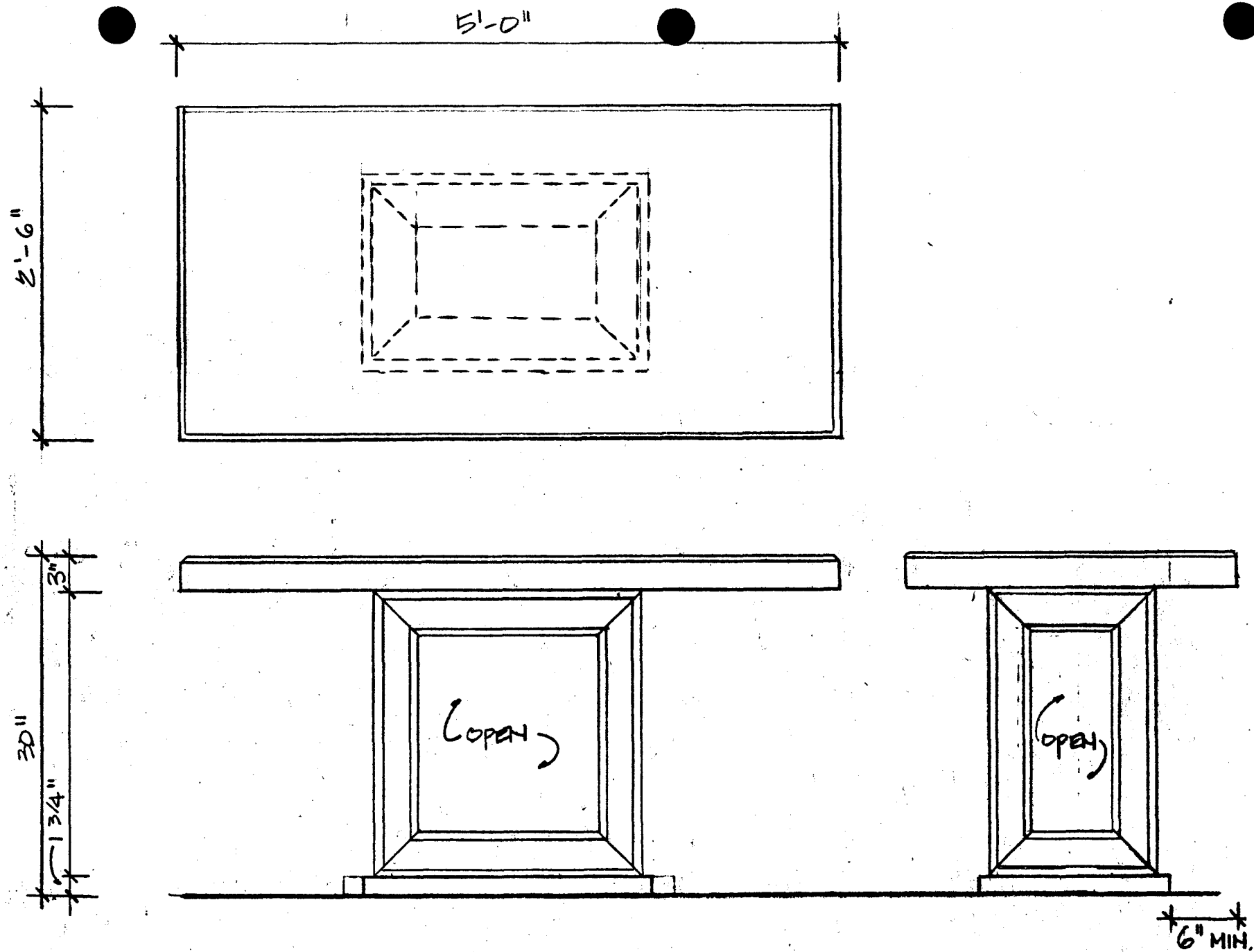
JASMINE CREEK RESIDENCE - DINING ROOM CONSOLE - SCALE: 1" = 1'-0"
