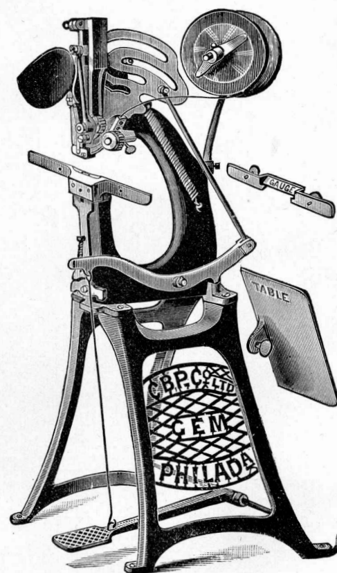
FOOT POWER, No. 31.
