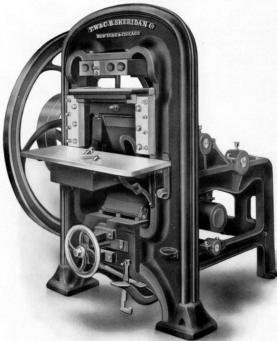
No. 4 ARCH EMBOSSE, HEAD 16\frac{1}{2}'' x 14''
