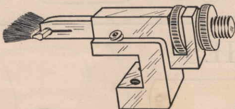
AUXILIARY BRUSH FOR CYLINDER PRESSES
