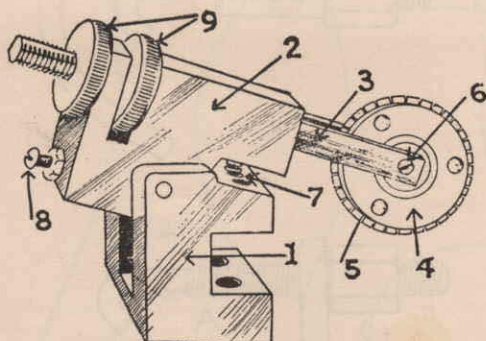
COWAN BALL BEARING PERFORATOR FOR CYLINDER PRESSES
