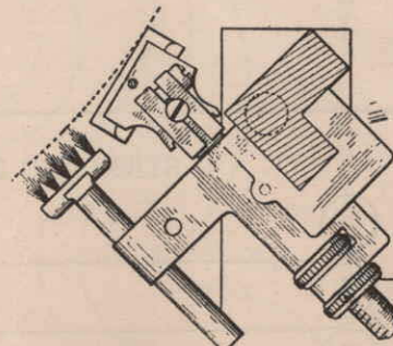
COWAN SLITTER FOR CYLINDER PRESSES
