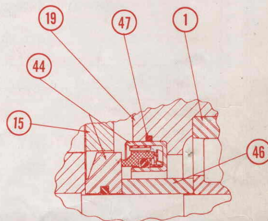
MECHANICAL SEAL 4500 MS Gas Pump Only
