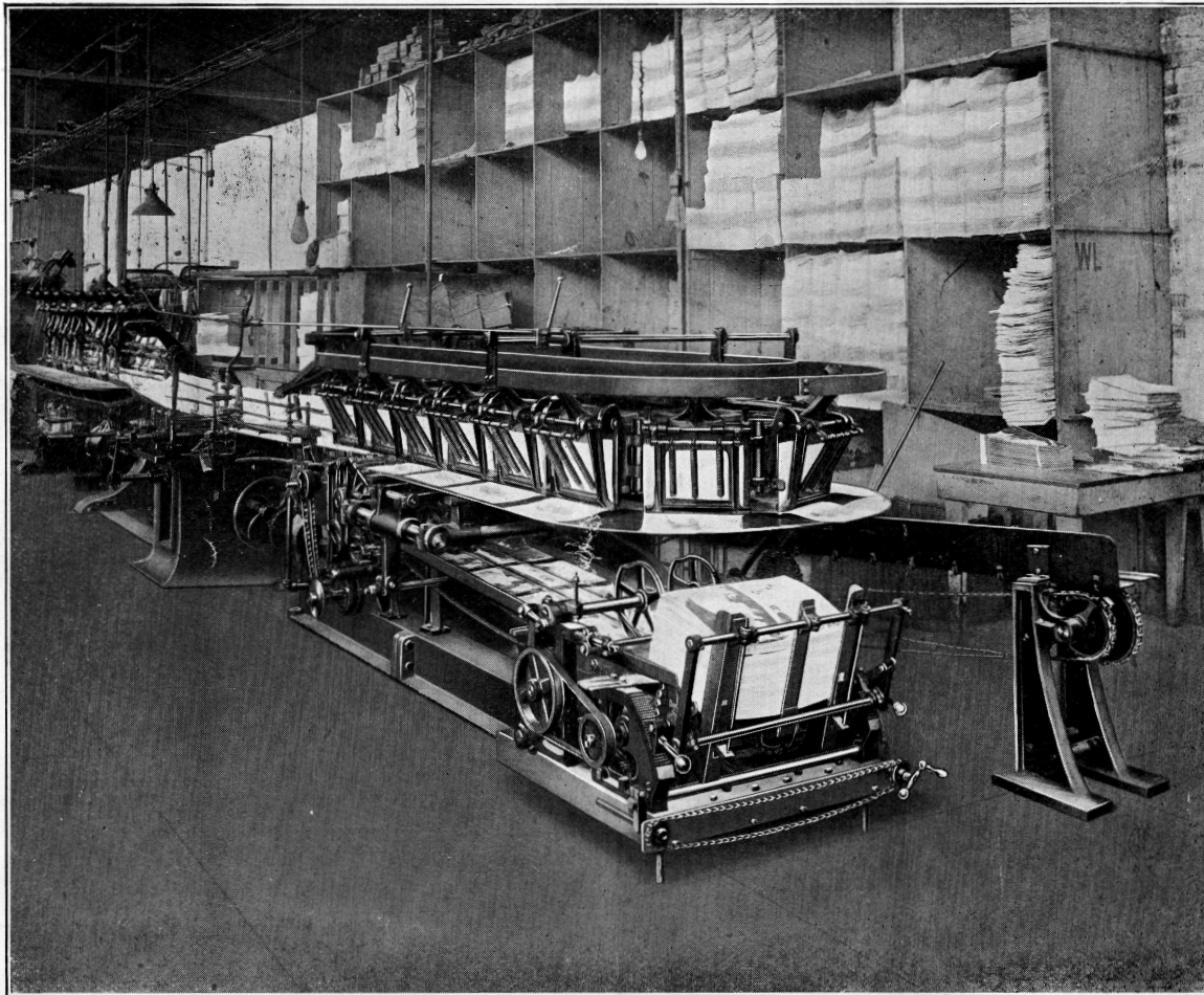
THREE-MACHINE COMBINATION Five operations at one time
