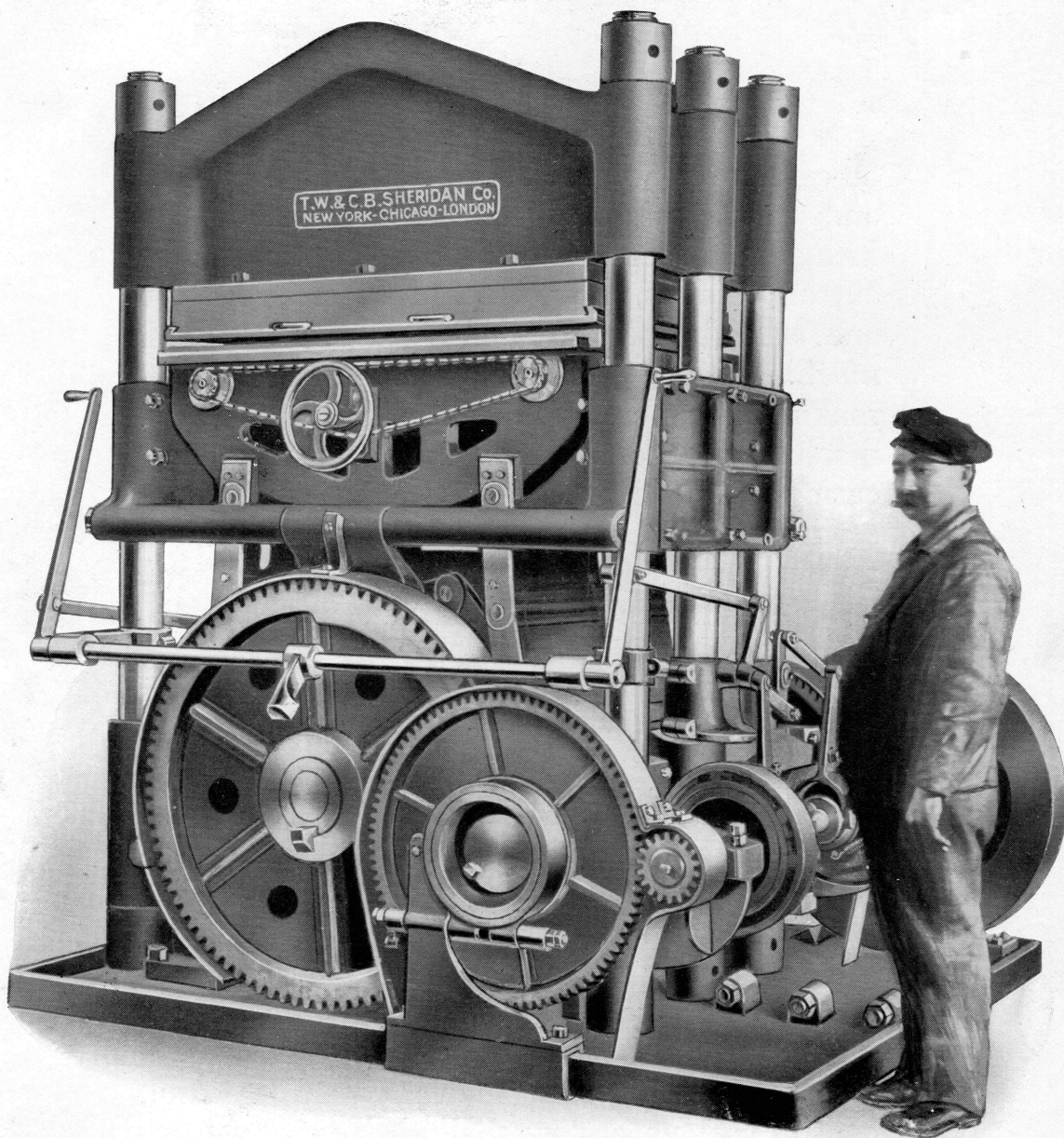
No. 10 PRESS, HEAD 54" x 36"
