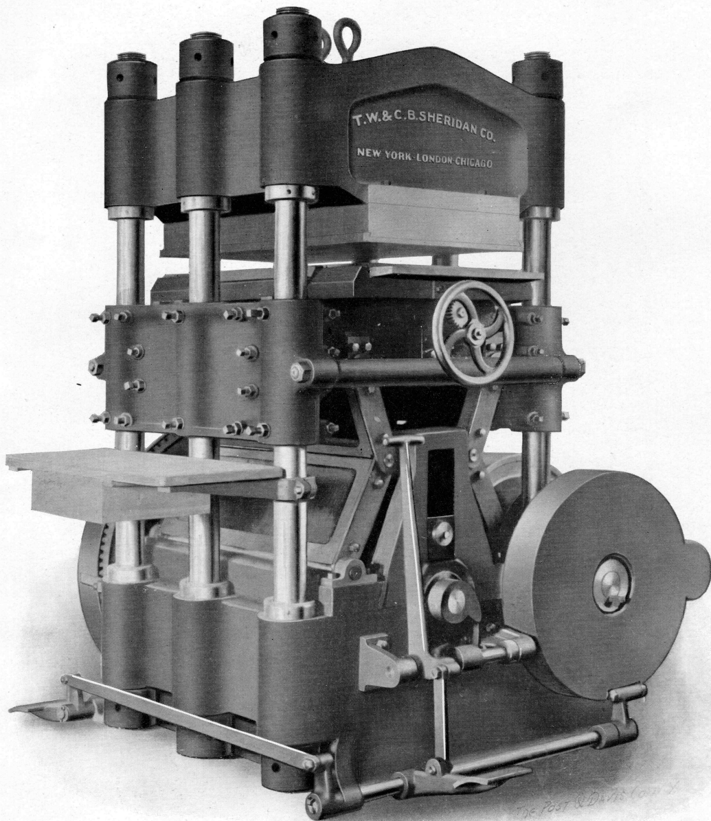
NO. 6B PRESS, HEAD 27" x 40"
