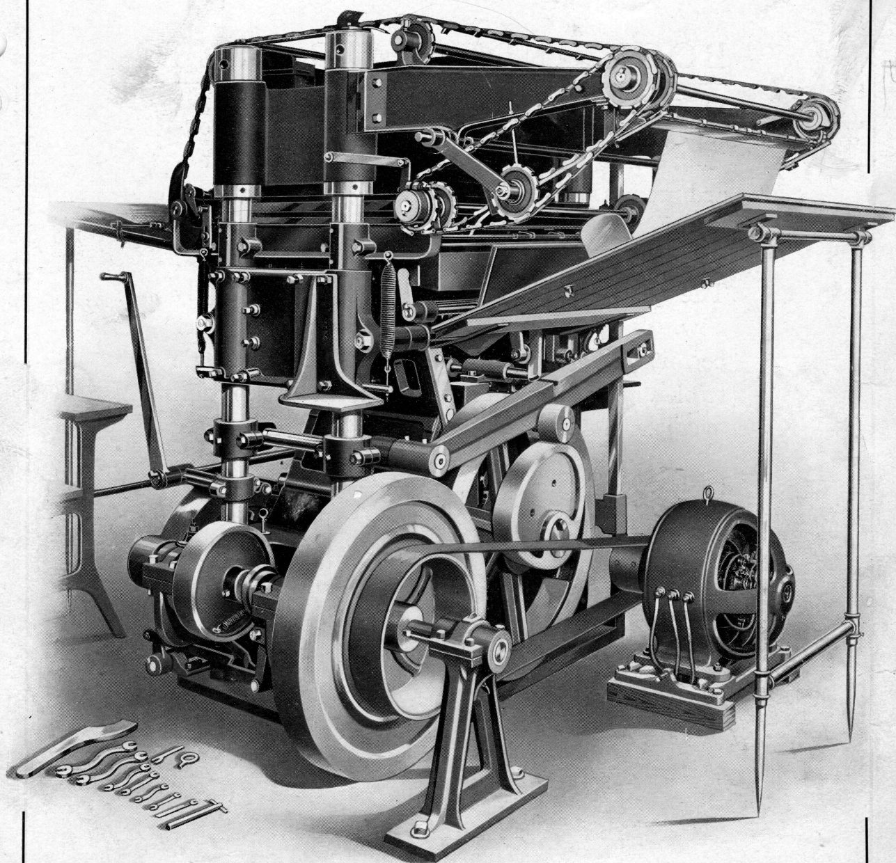
No. 8D PRESS, REAR VIEW
