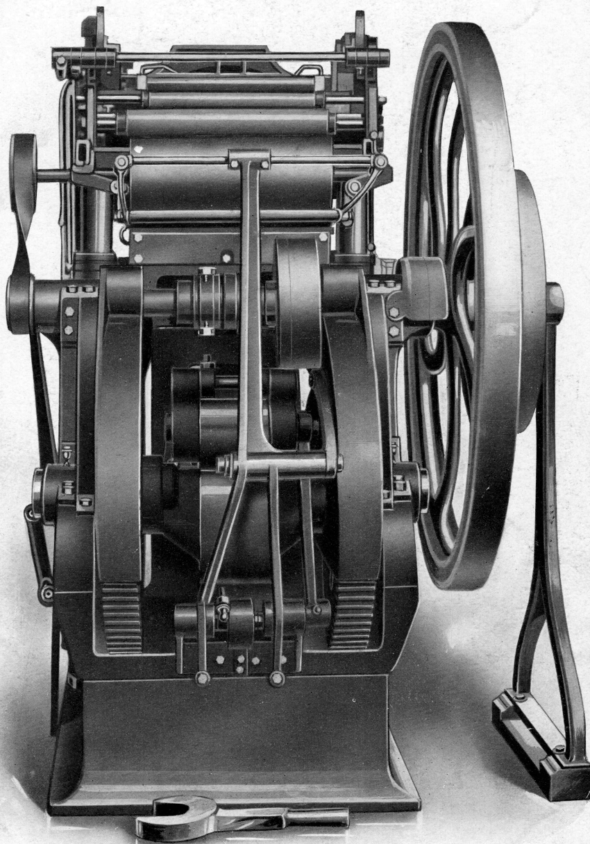
No. 11B PRESS-INKER, REAR VIEW
