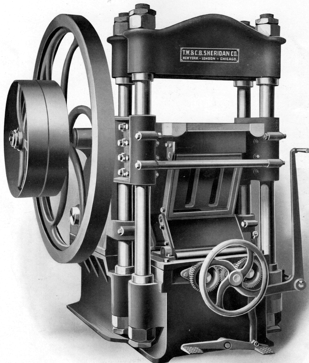
NO. 19 PRESS-SMASHER, HEAD 20" x 18"
