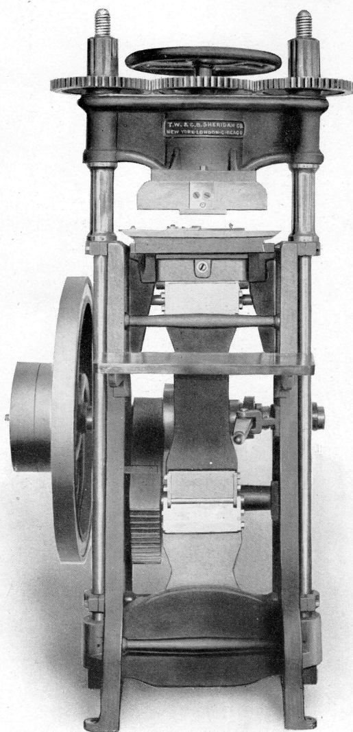
No. 2A PRESS, HEAD 15" x 11"
