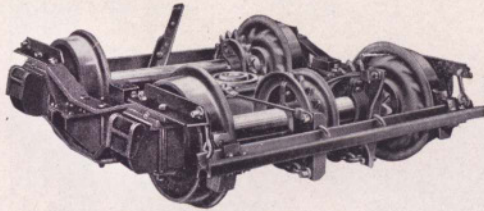
4-wheel trucks used on Clyde Decker Loaders, equipped with shoe brakes on all wheels.
