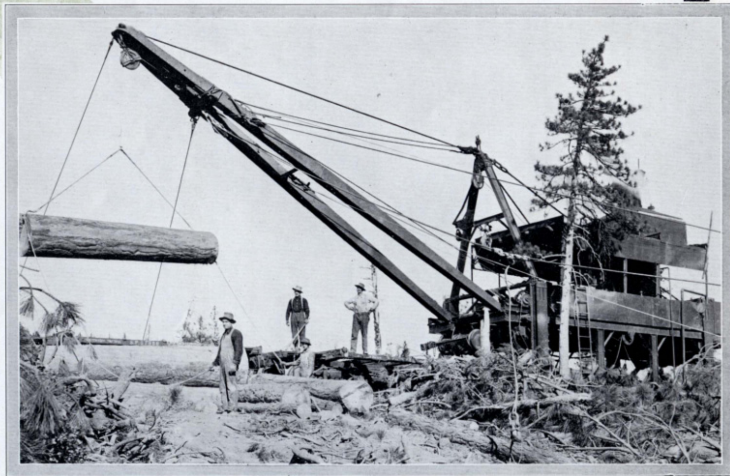
McGiffert Loader. Western type, for skidding and loading, using cable for haul back.
