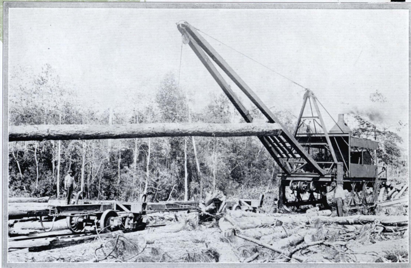
McGiffert Loader, with swinging boom, latticed at the base for heeling logs of extra length and loading with tongs.
