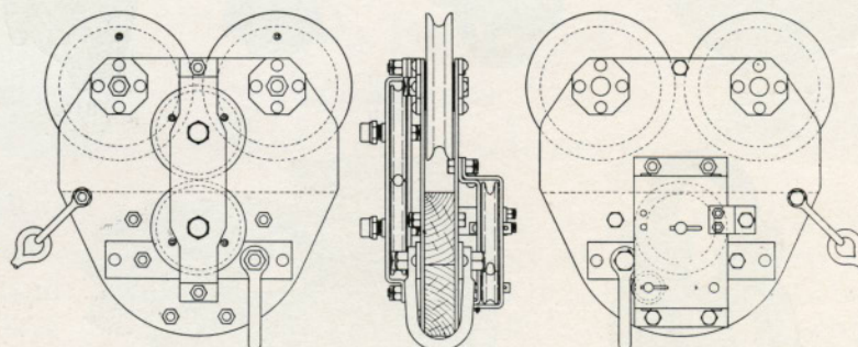
DH3050: Regular type of trolley carriage for cableway skidders. Steel trolley sheaves with hollow self lubricating sheaves, bronze bushed.
