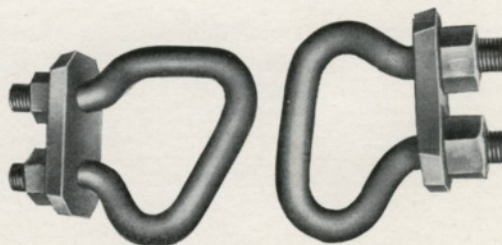
Shackles: Open face shackles or suspension links for hanging blocks to skidder boom. Made in various forms and sizes and material from 1-inch to 2-inch.
