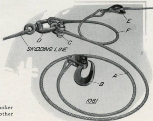
1061: Tag Line, with swivel connection to skidding, for connecting between skidding line and outhaul used with cable outhaul ground skidders.
