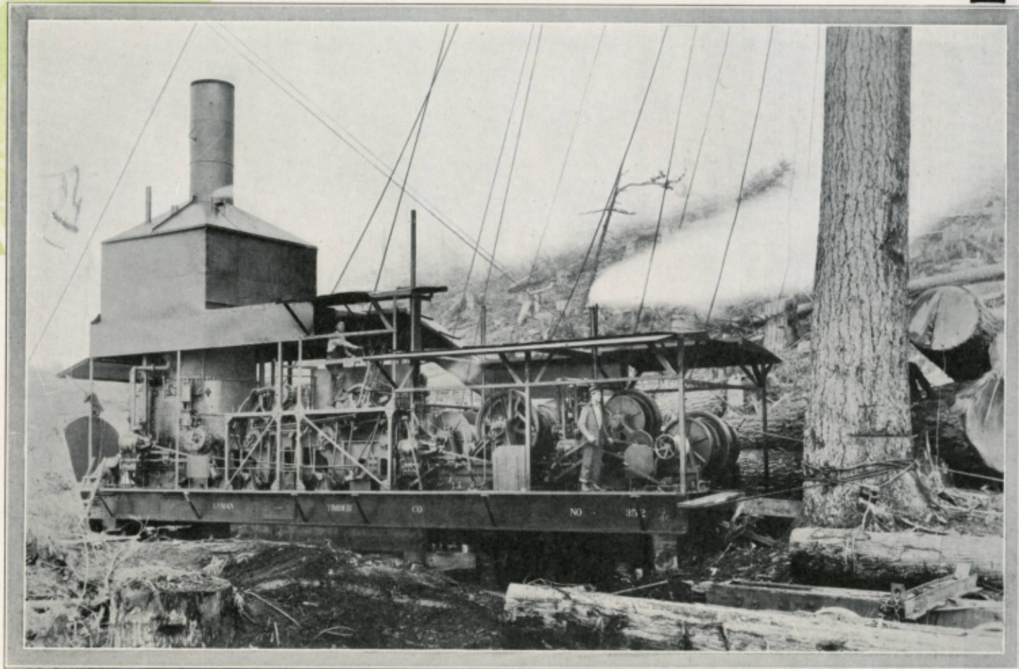
Clyde Western Type Cableway Skidder and Loader for Tree Rigging. (Operator's Side.)
