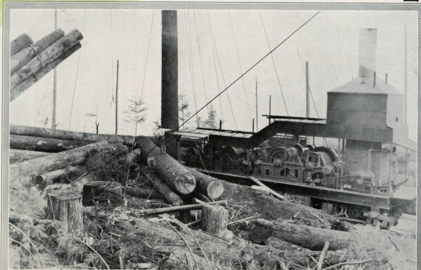
Clyde Western Type Cableway Skidder and Loader for Tree Rigging.
