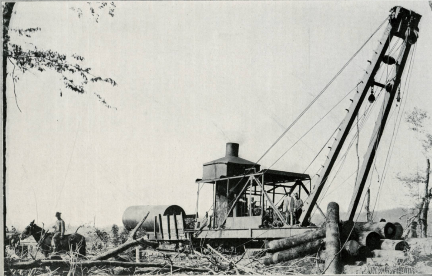
Clyde Two-Line Single End Skidder with Cable Outhaul.
