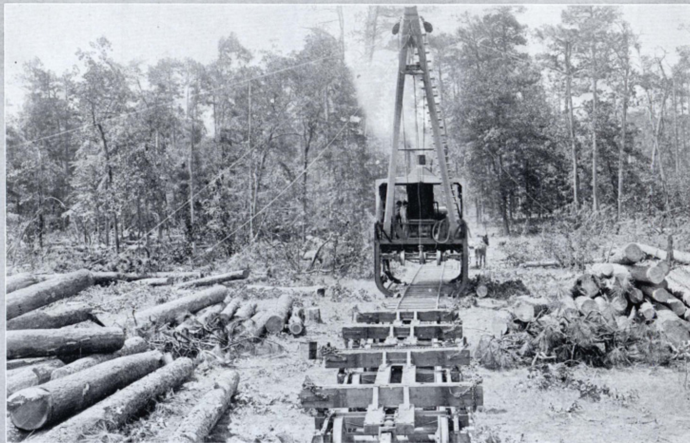
McGiffert Loader, used for skidding with two lines, one running from each side and horse for taking the line out.
