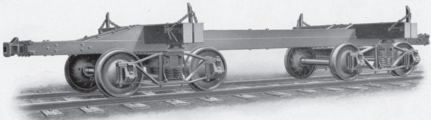
60,000 Lbs. Capacity Logging Car with Steel Trucks.
