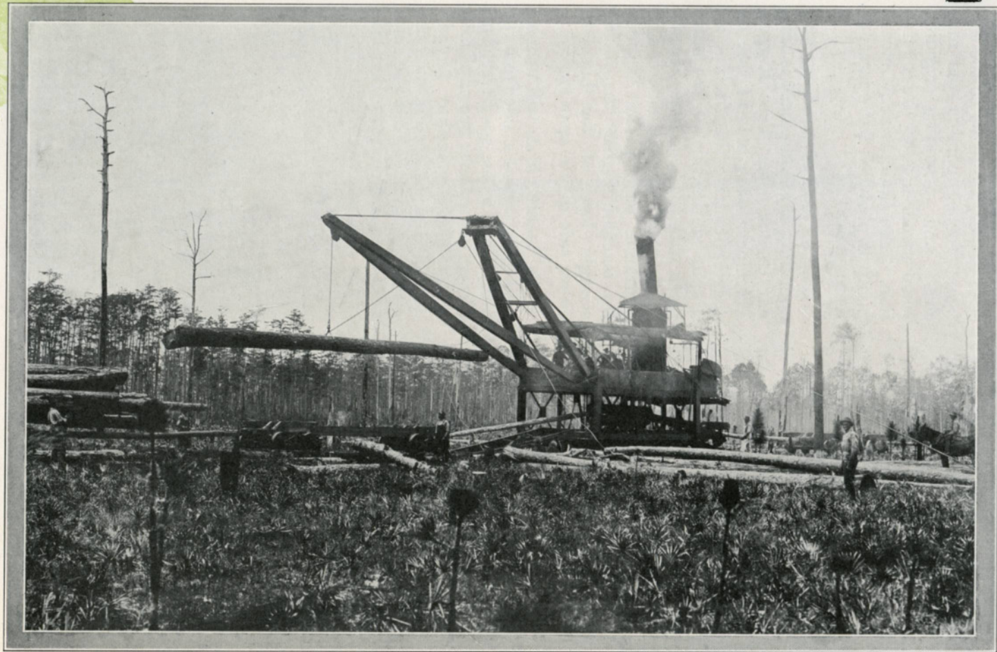
Clyde Universal Skidder and Loader Operating Two Skid- ding Lines with Horse Outhaul.
