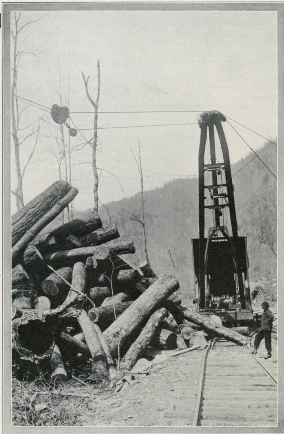
Clyde Cableway Skidder.
