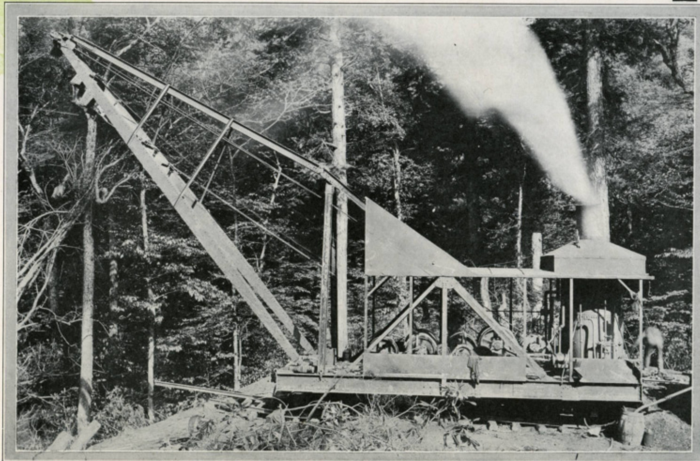
Clyde Cableway Skidder.
