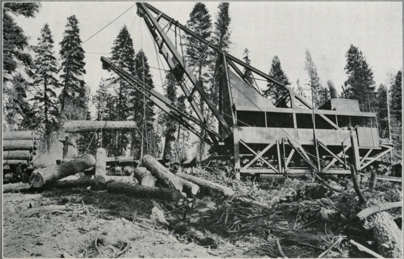
Clyde Universal Skidder and Loader for Operating Two Skidding Lines with Cable Outhaul (Both skidding lines operating on same side).
