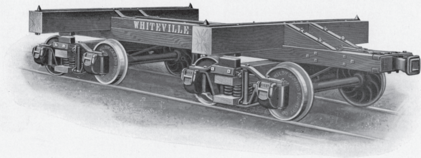
40,000 Lbs. Capacity Logging Car.
