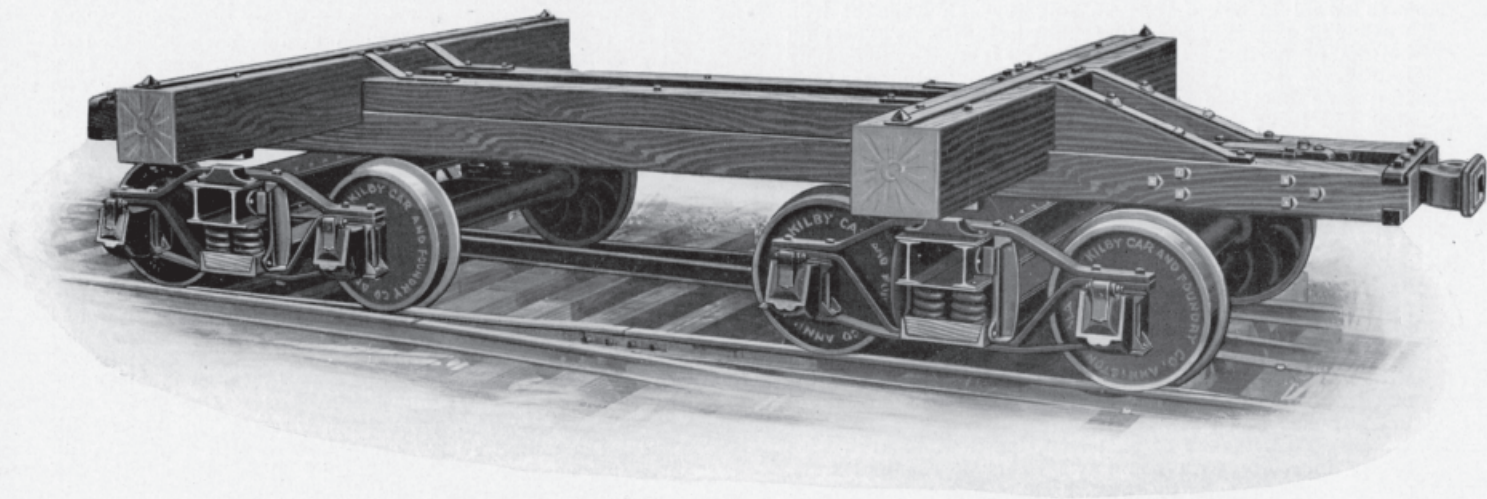
40,000 Lbs. Capacity Logging Car with Steel Trucks.
