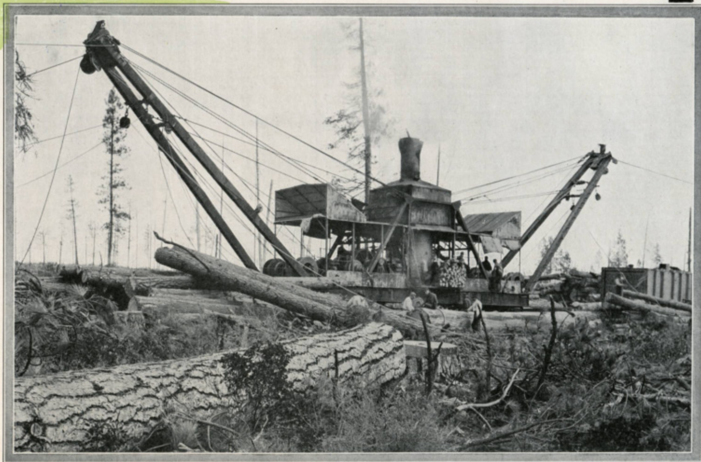
Clyde Four-Line Skidder with Cable Outhaul.
