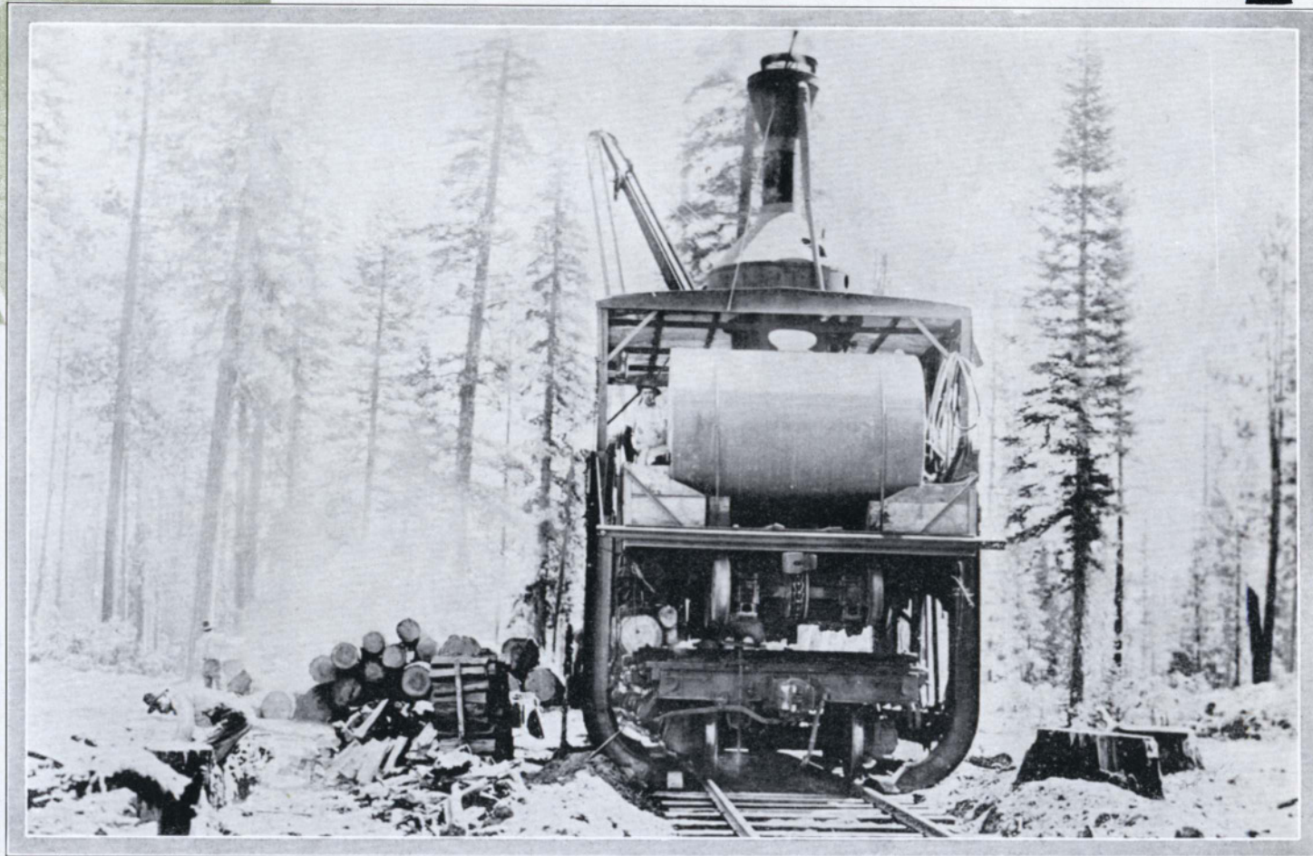
McGiffert Loader, Rear view, showing Trucks raised and standard flat car pass- ing through.
