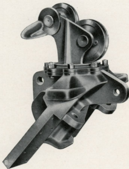
Cast steel boom cap for cableway skidder equipped with storage drum for main cable. Sheaves for main cable and takeup line are mounted in a swiveling bracket so as to lead perfectly in any direction.
