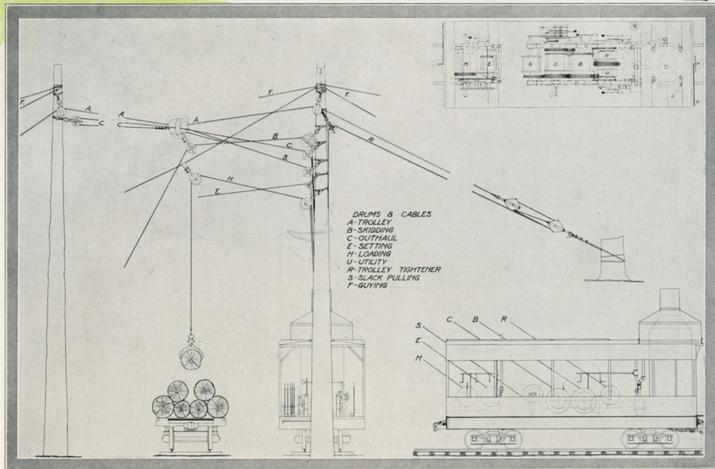
Clyde Cableway Tree Rigged Skidder.
