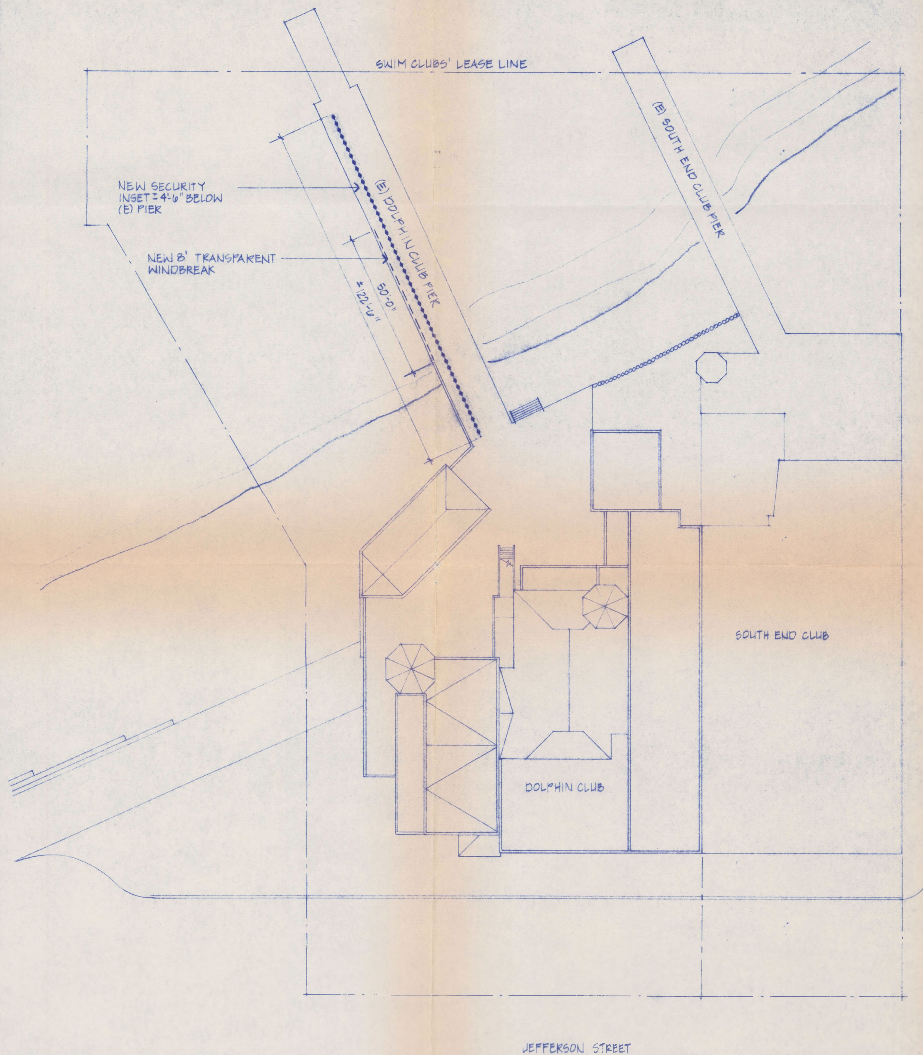
SITE PLAN
