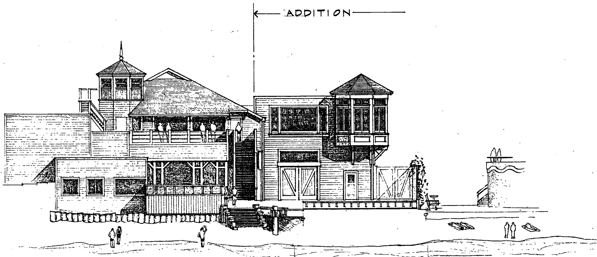
NORTH ELEVATION
