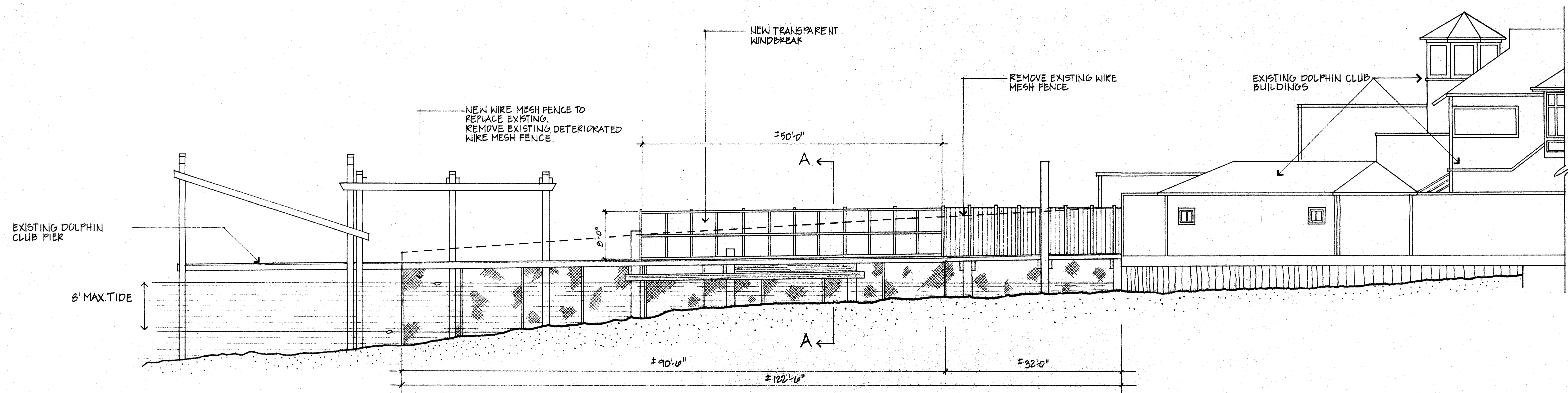
1 WEST ELEVATION 2 SCALE - 1/8" = 1'-0"
