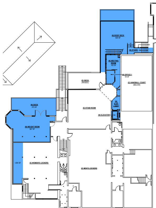
FLOOR 02
