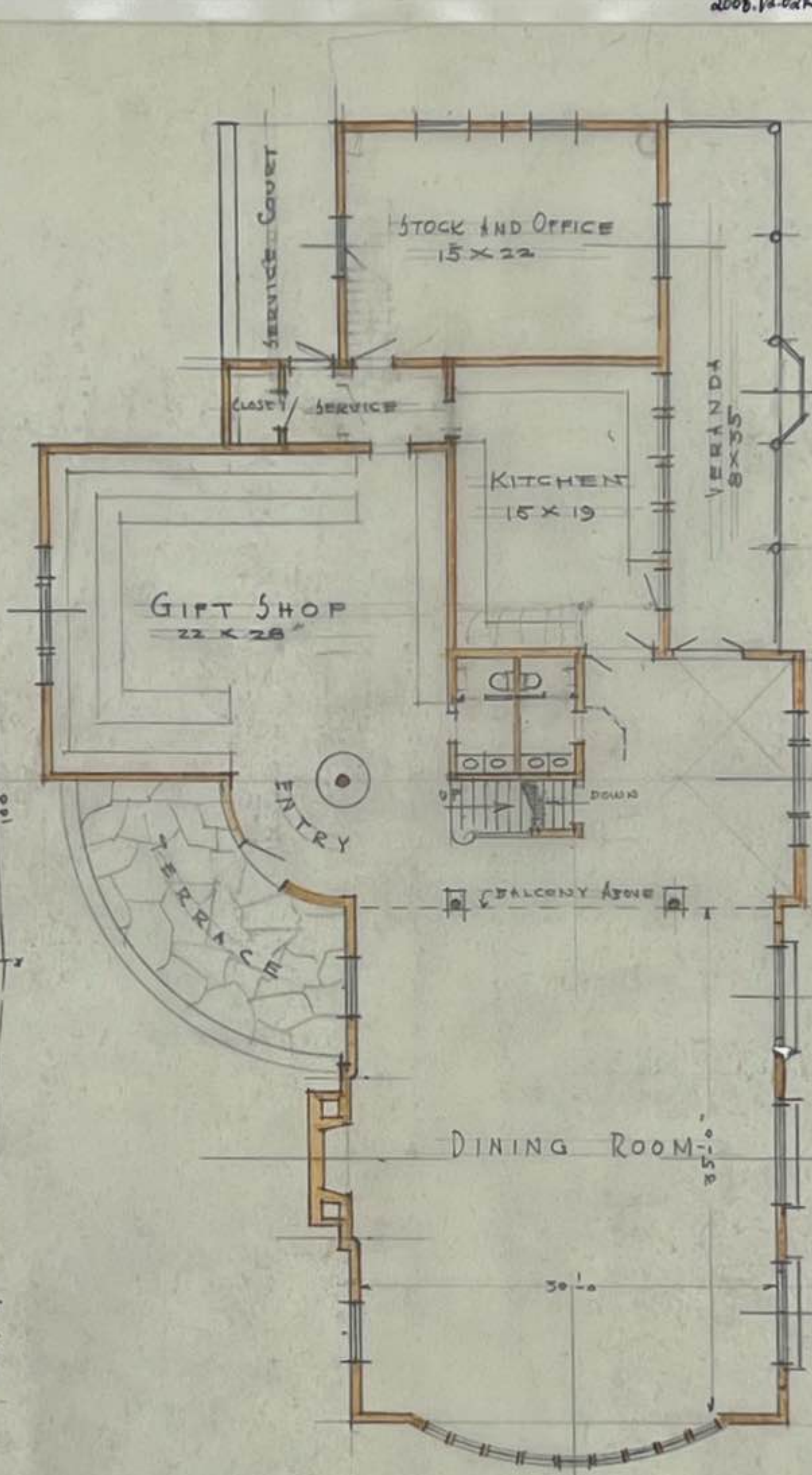
MAIN FLOOR PLAN.
